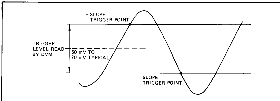
Figure 3-18. Hysteresis Band
