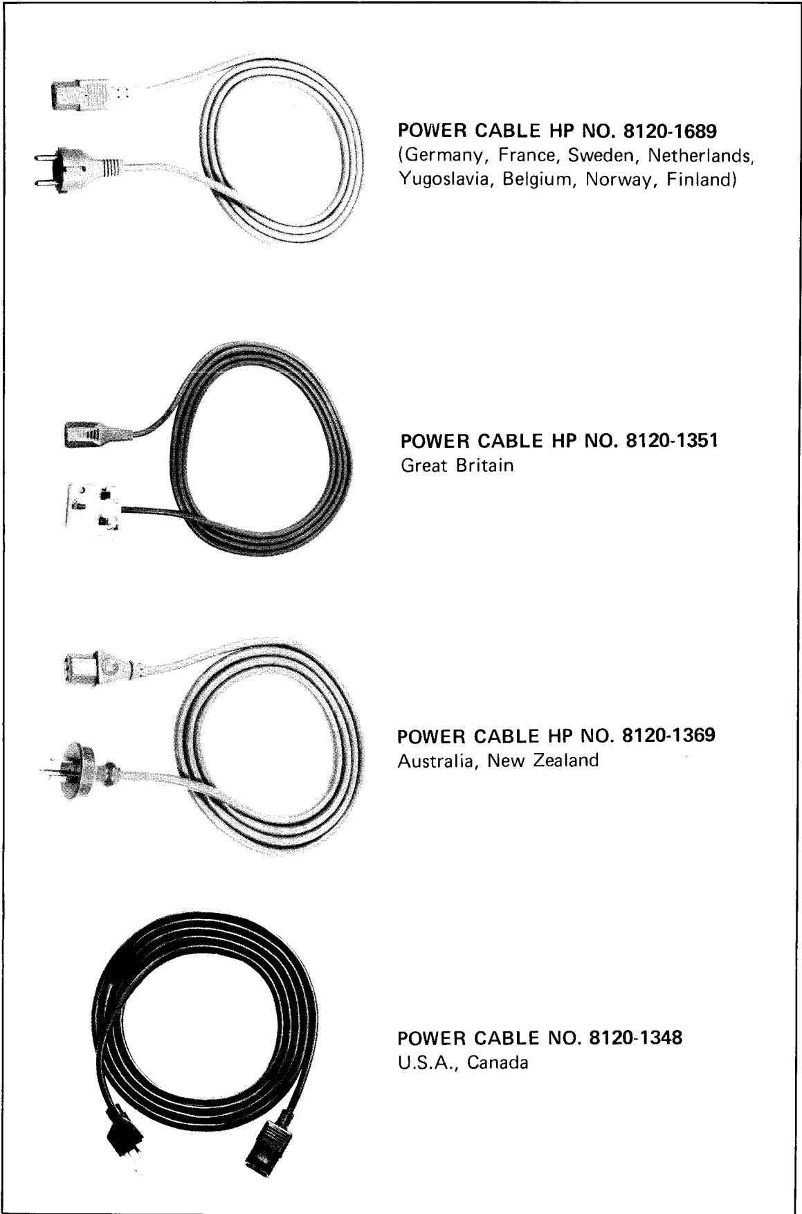
Figure 2-1. Power Cables
