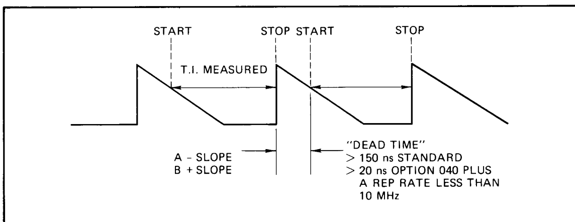
Figure 4-3. Dead Time
