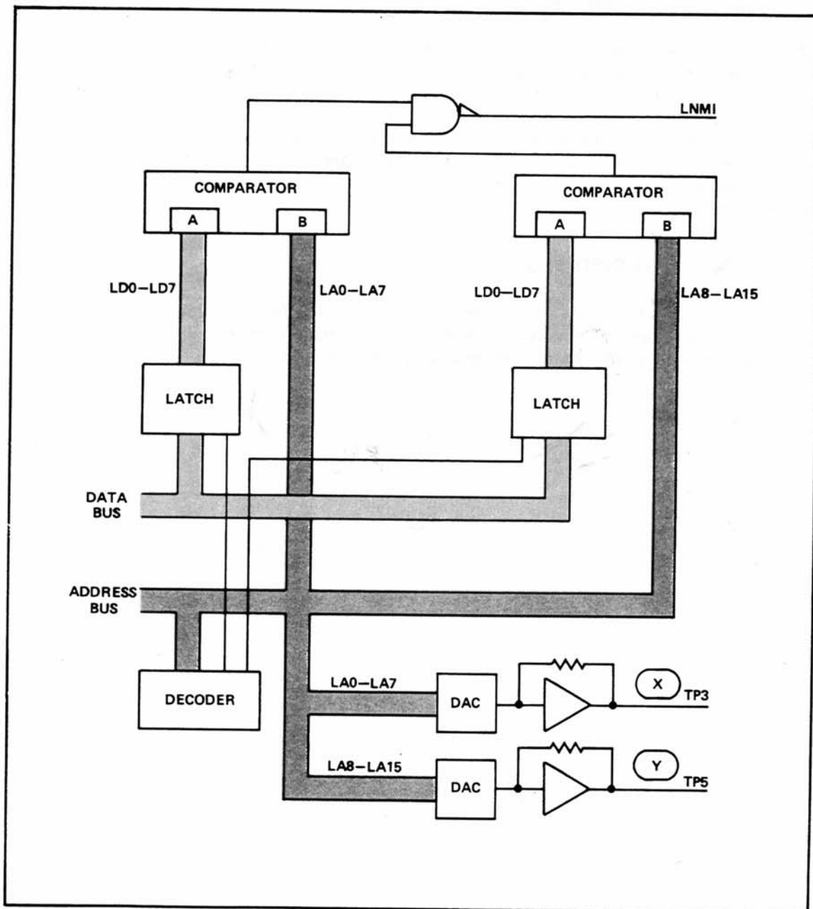
Figure 8-4. 05370-60014 Block Diagram
