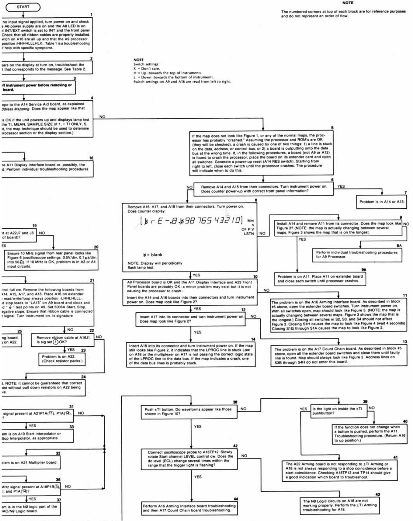
Figure 8-13. Troubleshooting Assembly Isolation Flowchart Fifth (and final) part of page 8-53, which folds out.
