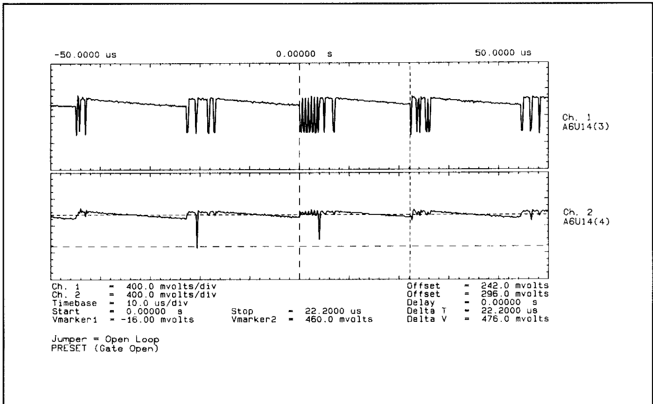
Figure 7F-8. Waveform at A6U14(3,4)
