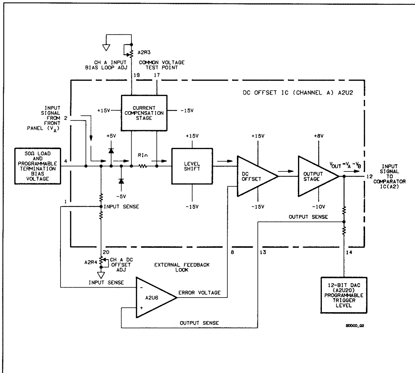
Figure 7C-1. DC Offset IC Simplified Block Diagram
