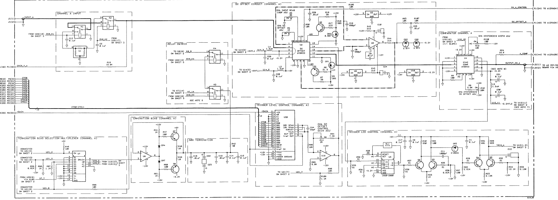
Figure 7C-9. A2 Input Amplifier Board, Schematic Diagram (Sheet 1 of 3)
