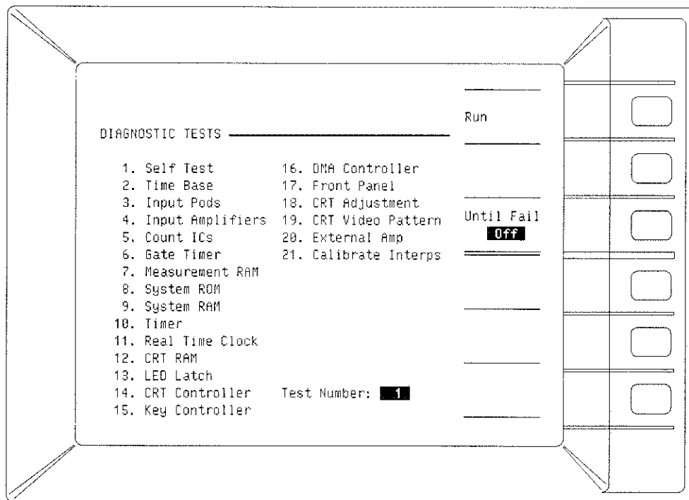
Figure 7A-1. TEST Menu Screen
