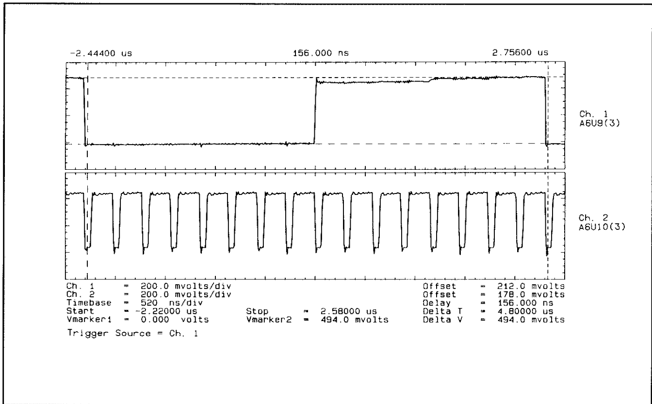
Figure 7F-4. A6U10(3) Waveform
