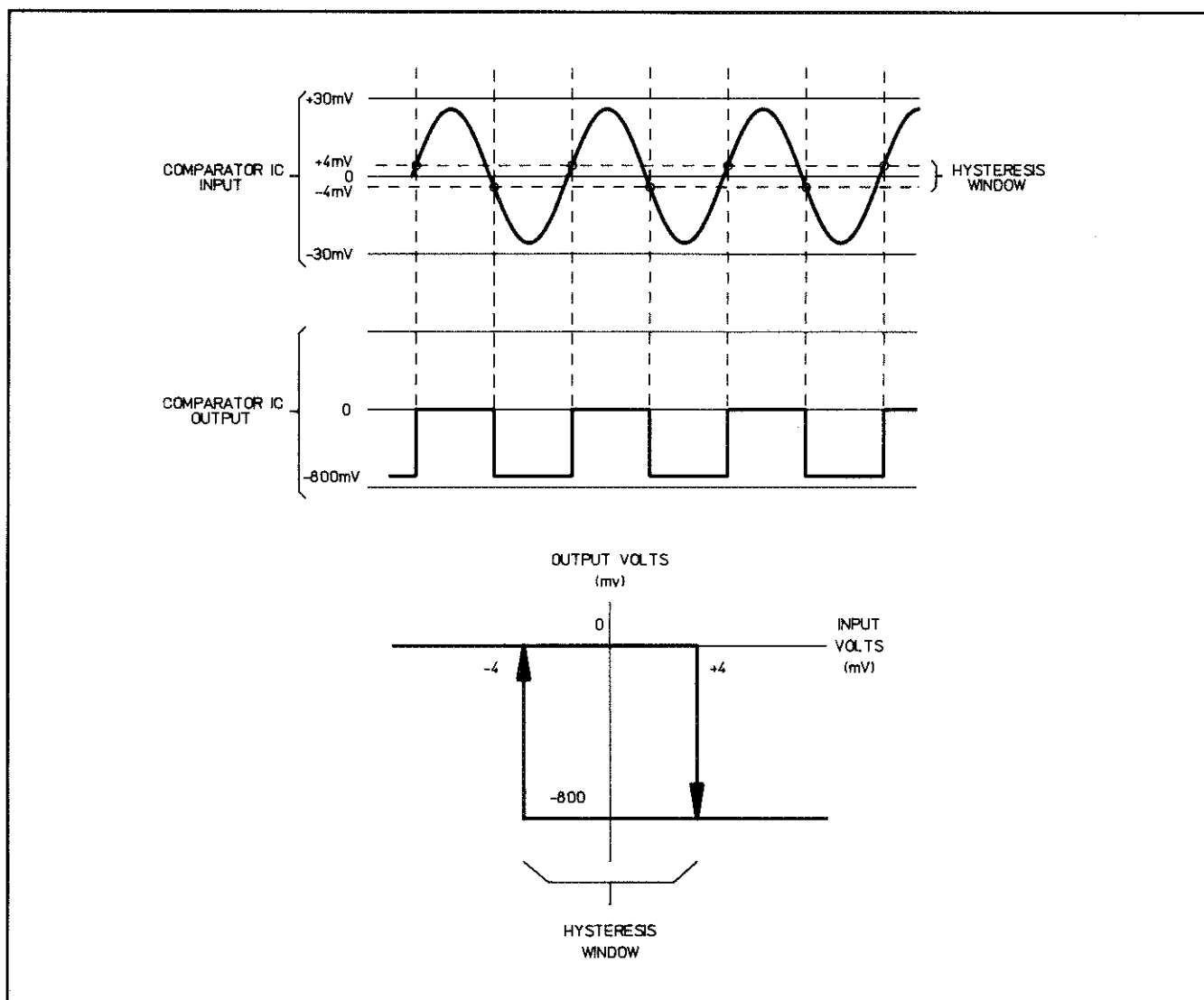
Figure 7C-3. Comparator IC Hysteresis Window
