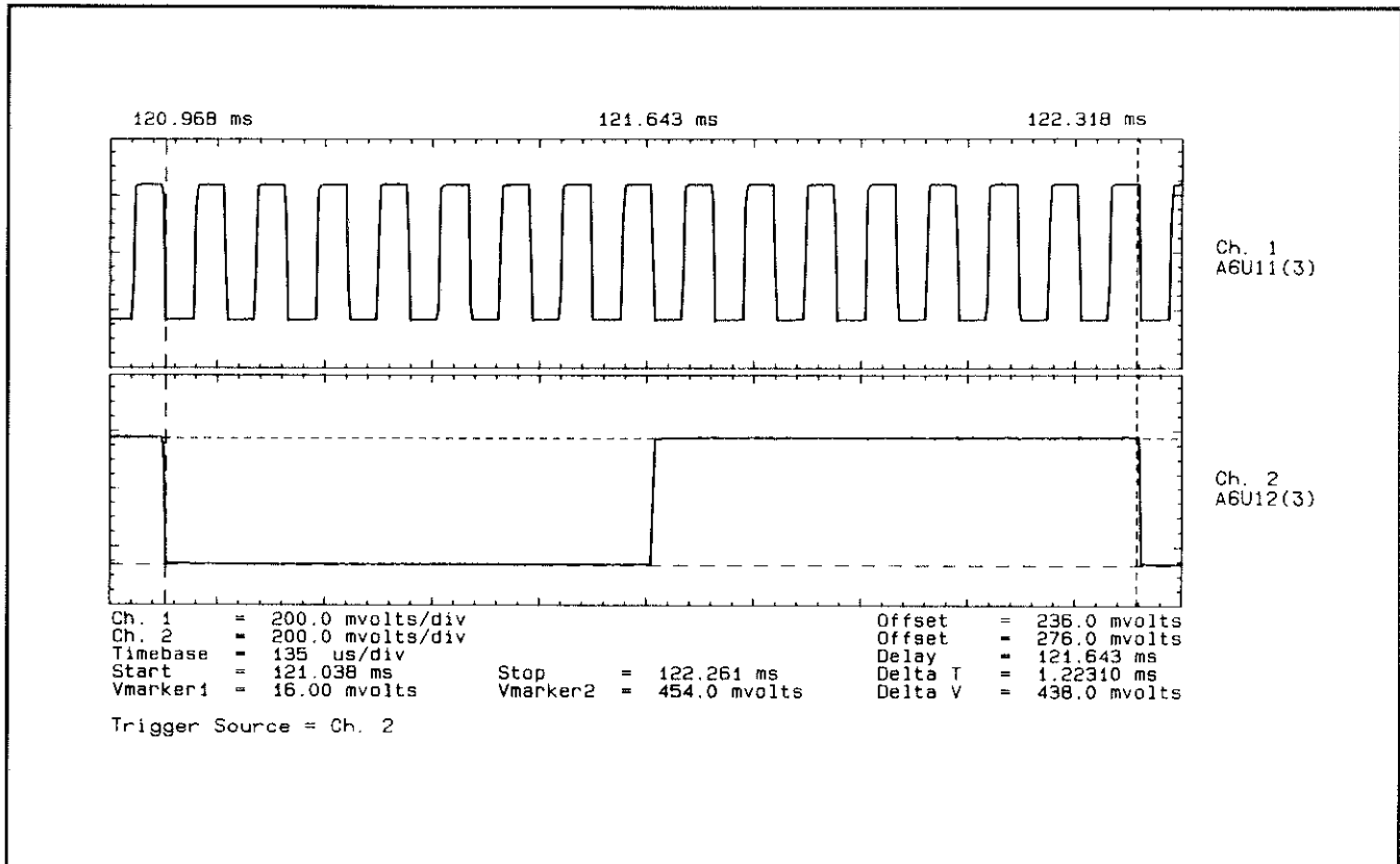
Figure 7F-5. Waveforms at A6U11(3)
