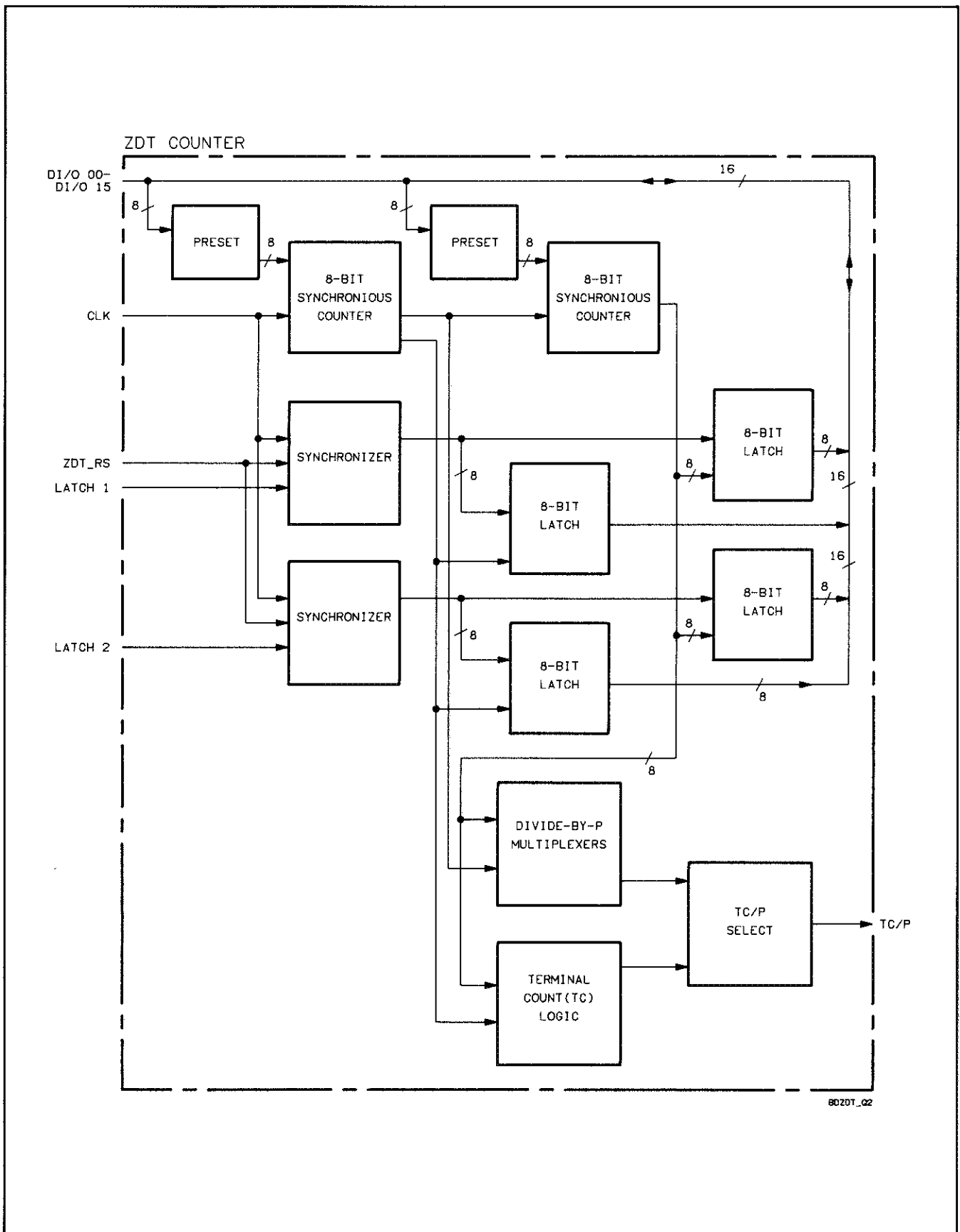
Figure 7E-3. Simplified Zero-Dead-Time (ZDT) Counter Block Diagram
