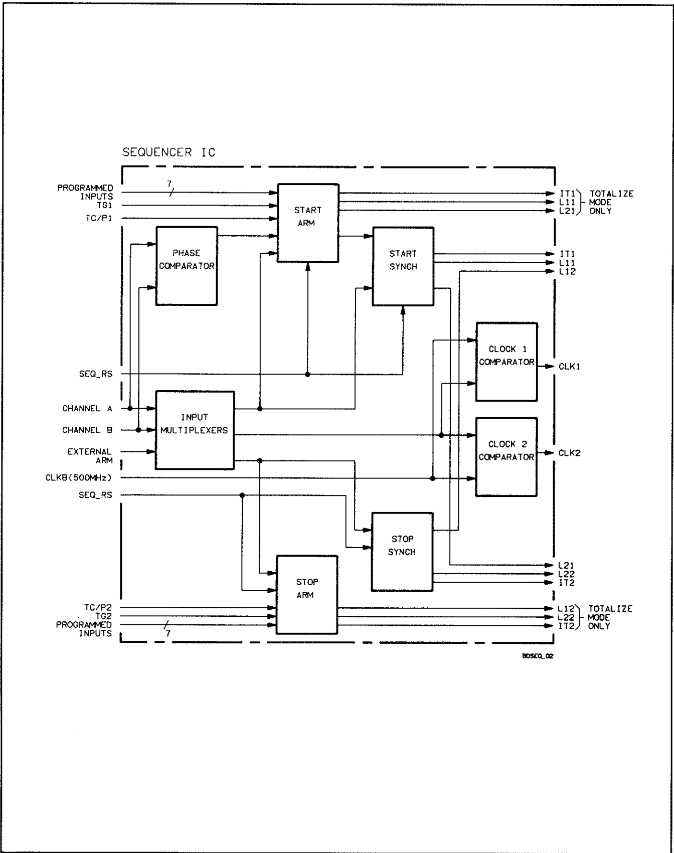
Figure 7E-2. Simplified Sequencer IC Block Diagram
