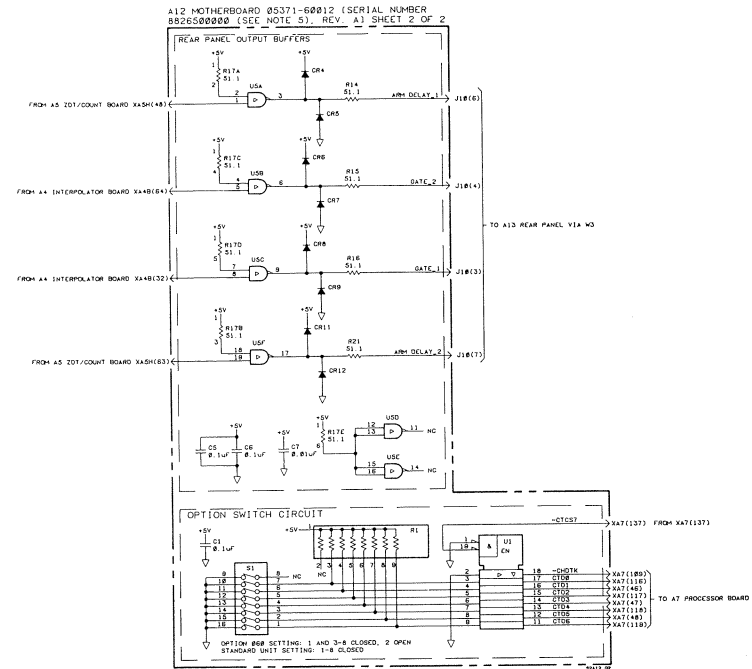
Figure 7K-1. A12 Motherboard, Schematic Diagram (Sheet 2 of 2)
