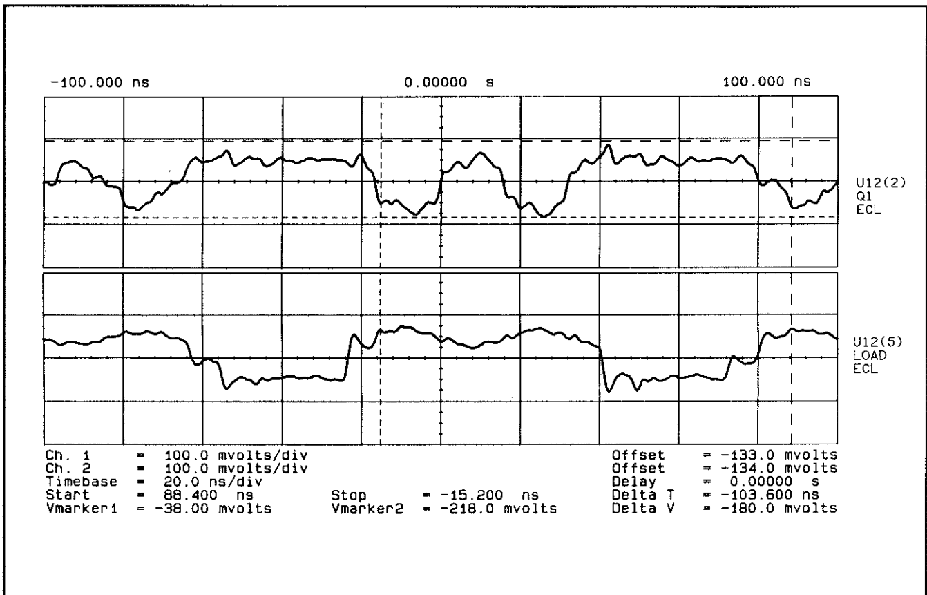
Figure 7E-9. Waveform at A5U12(2)
