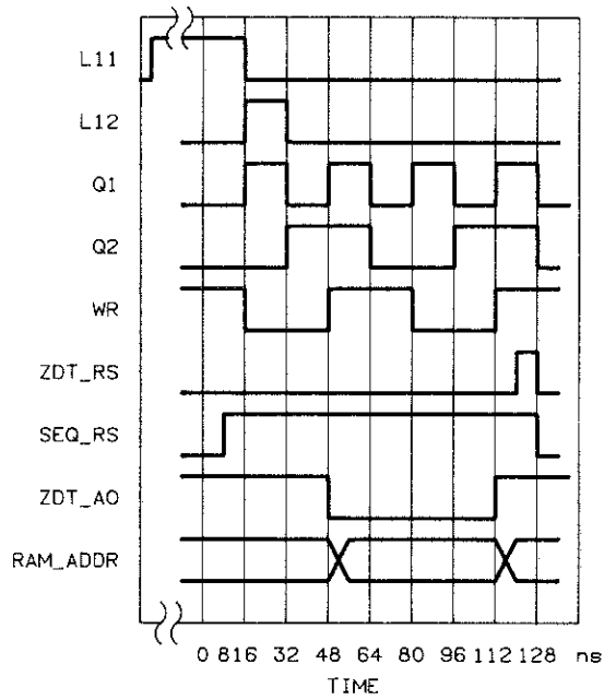
Figure 7E-5. Double-Write Measurement Timing Diagram
