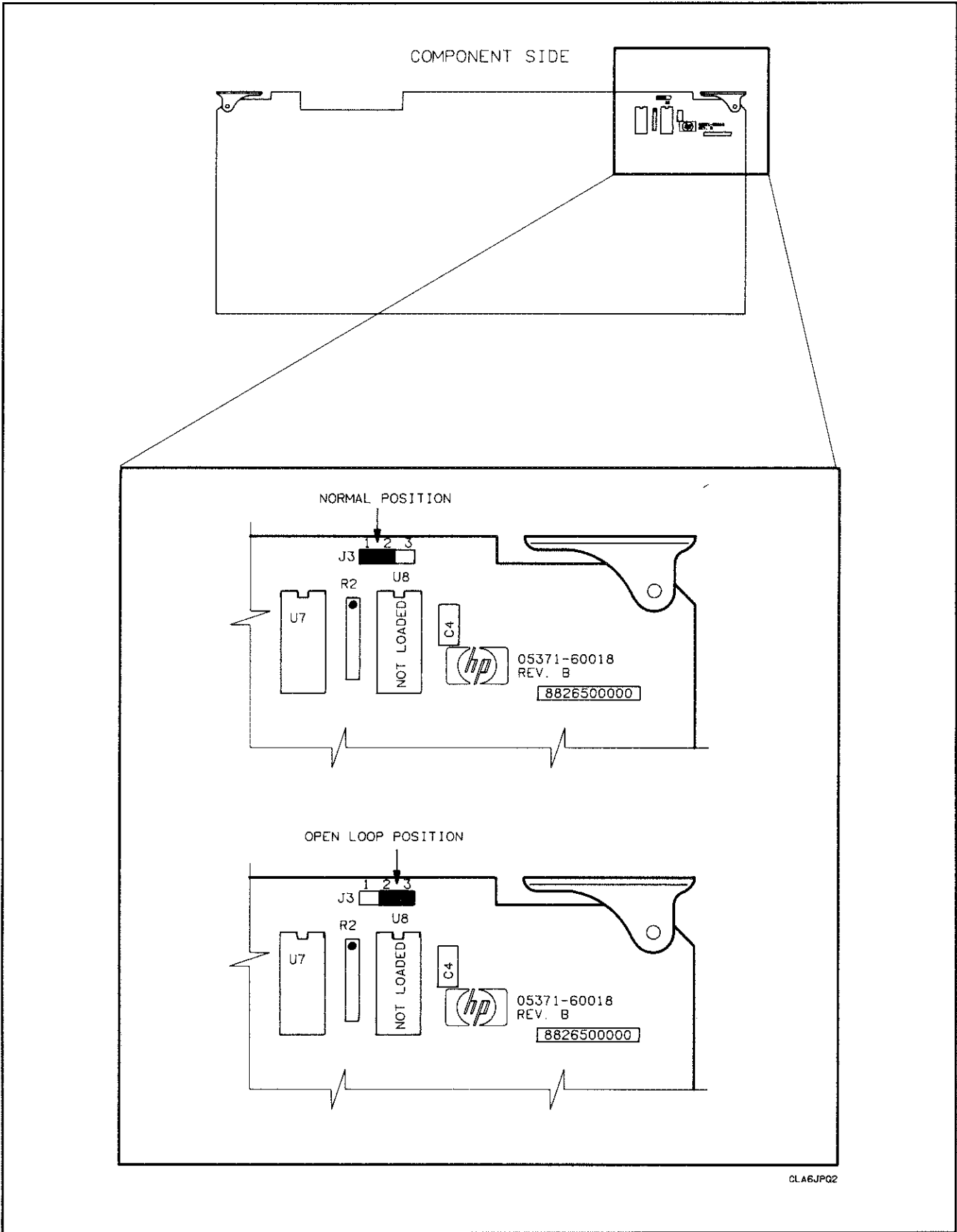
Figure 7F-2. A6 DMA/GATE Assembly Jumper Positions
