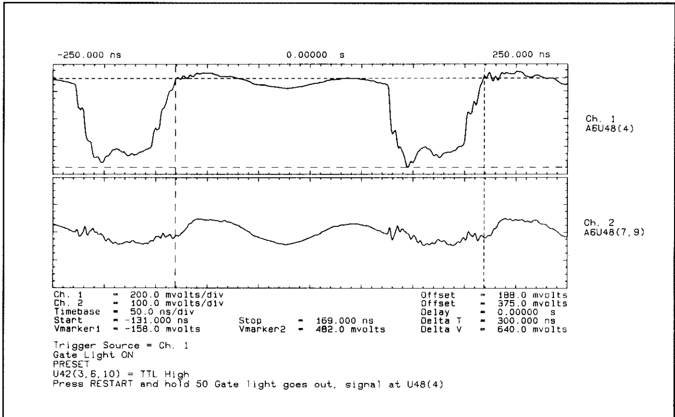
Figure 7F-9. Waveforms at A6U48(4,7,9)
