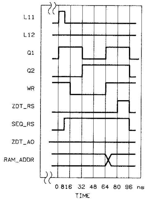
Figure 7E-4. Single-Write Measurement Timing Diagram
