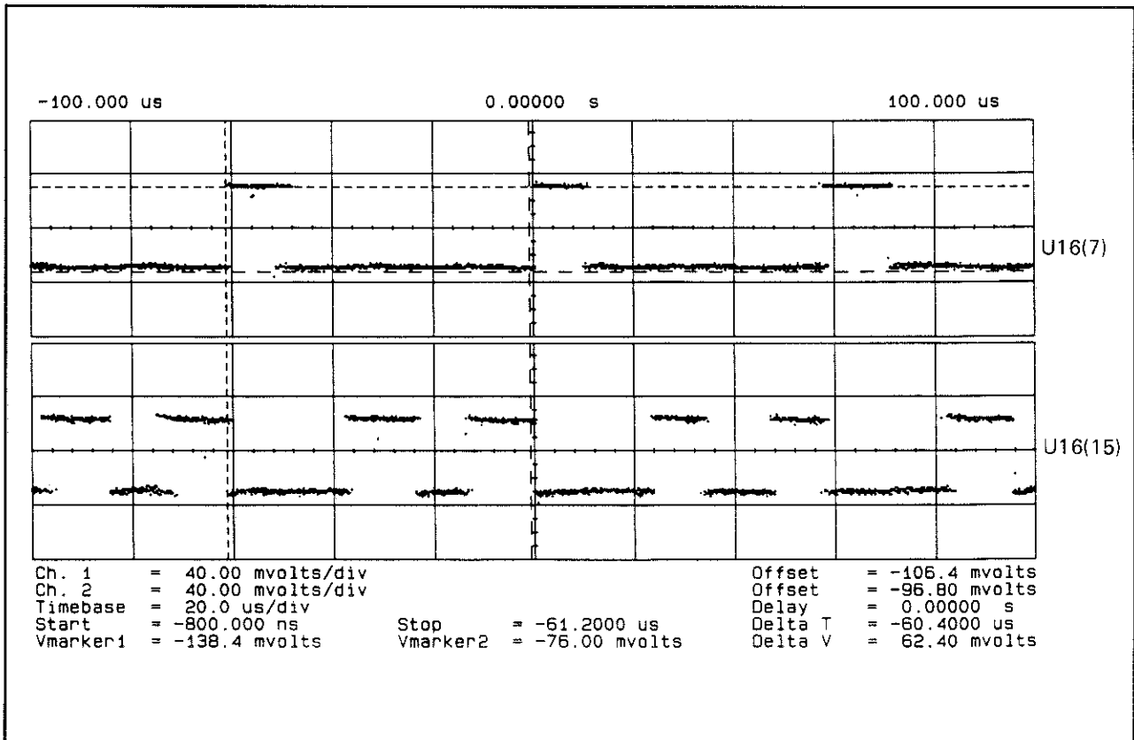
Figure 7D-14. Waveforms at A4U16(11) and A4U27(11)
