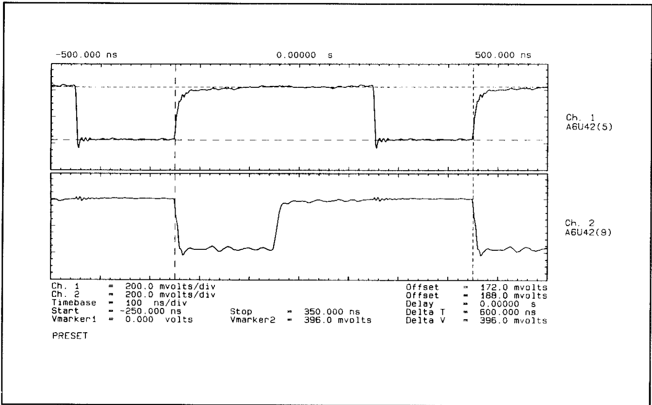
Figure 7F-15. Waveforms at A6U42(5,9)
