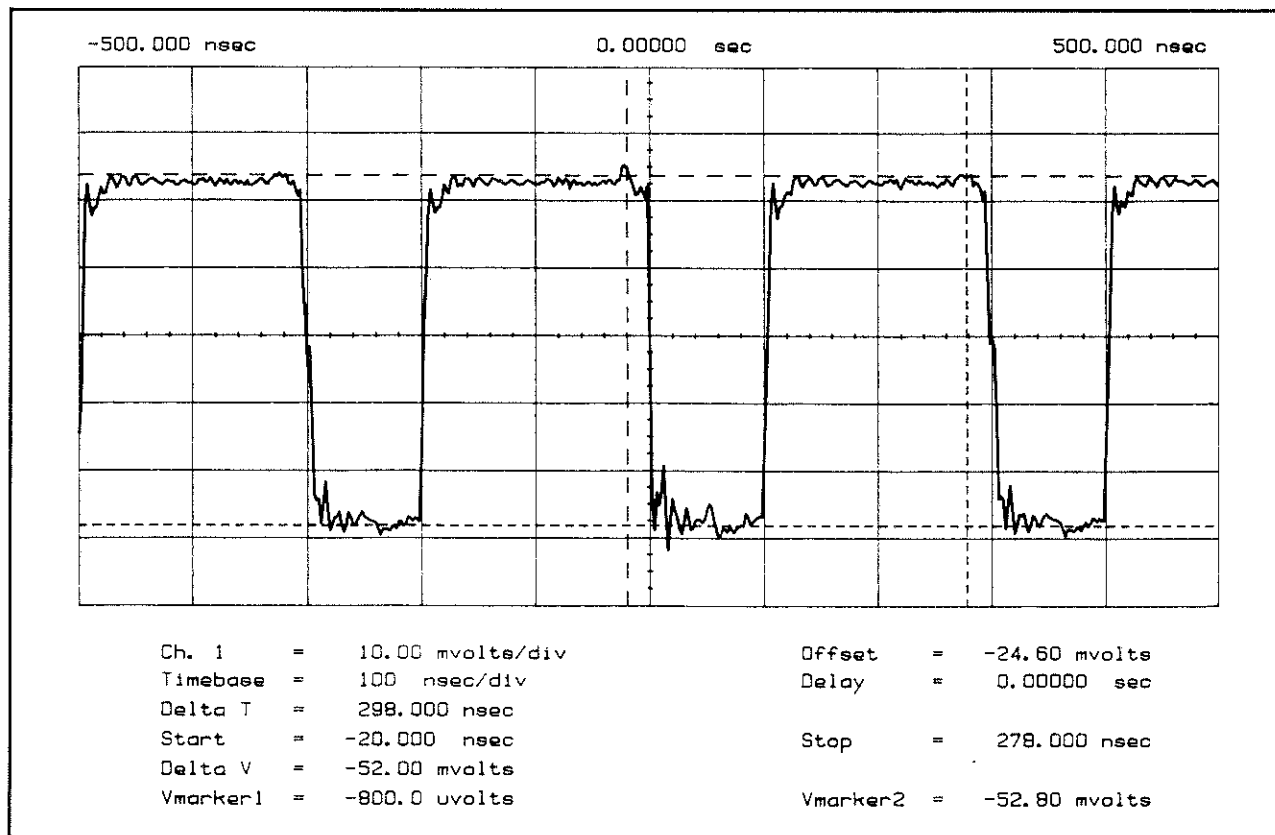
Figure 7D-9. Waveforms at TP4 and TP6
