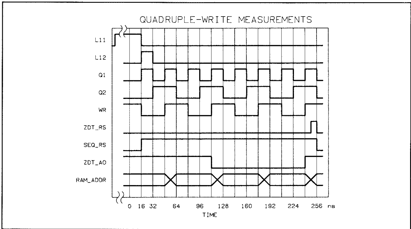
Figure 7E-6. Quadruple-Write Measurement Timing Diagram
