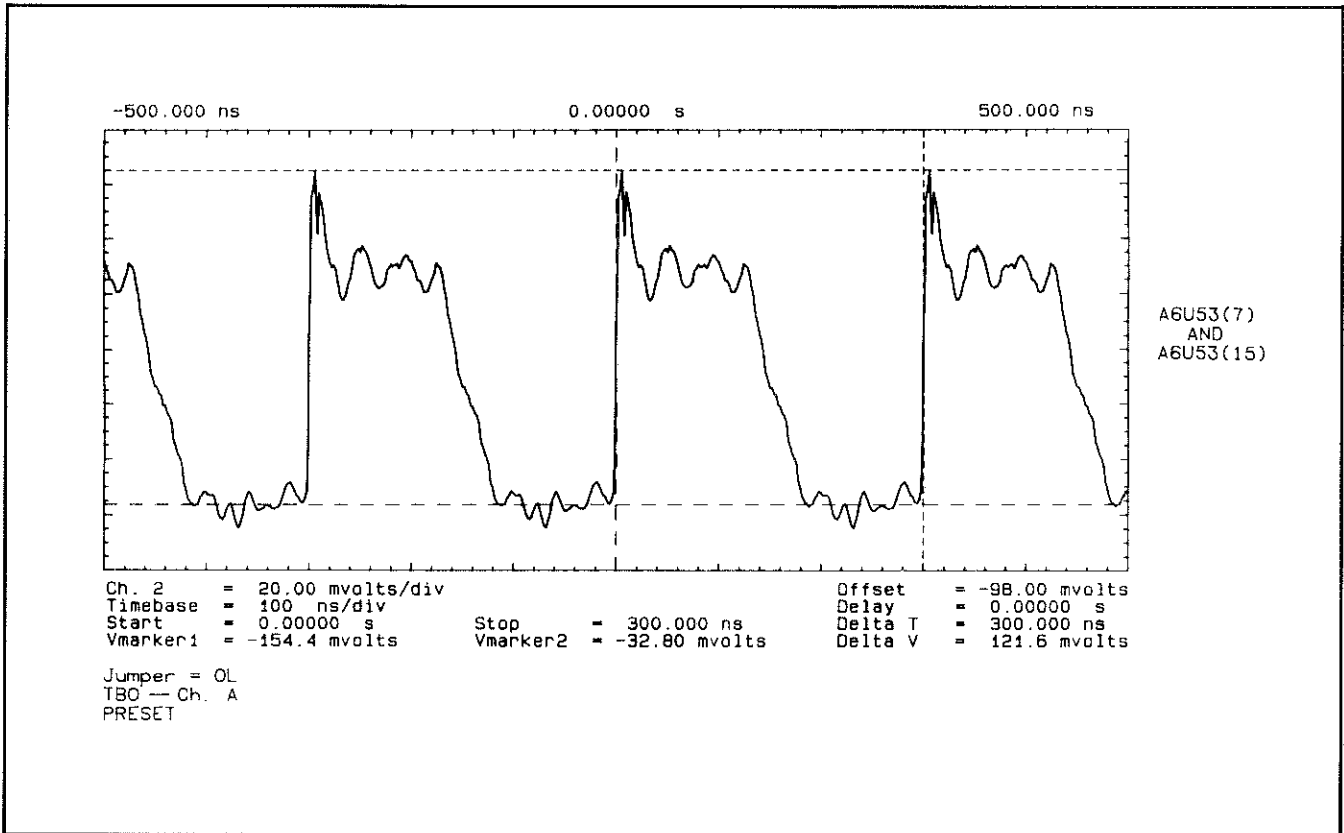
Figure 7F-23. Waveforms at A6U53(7,15)
