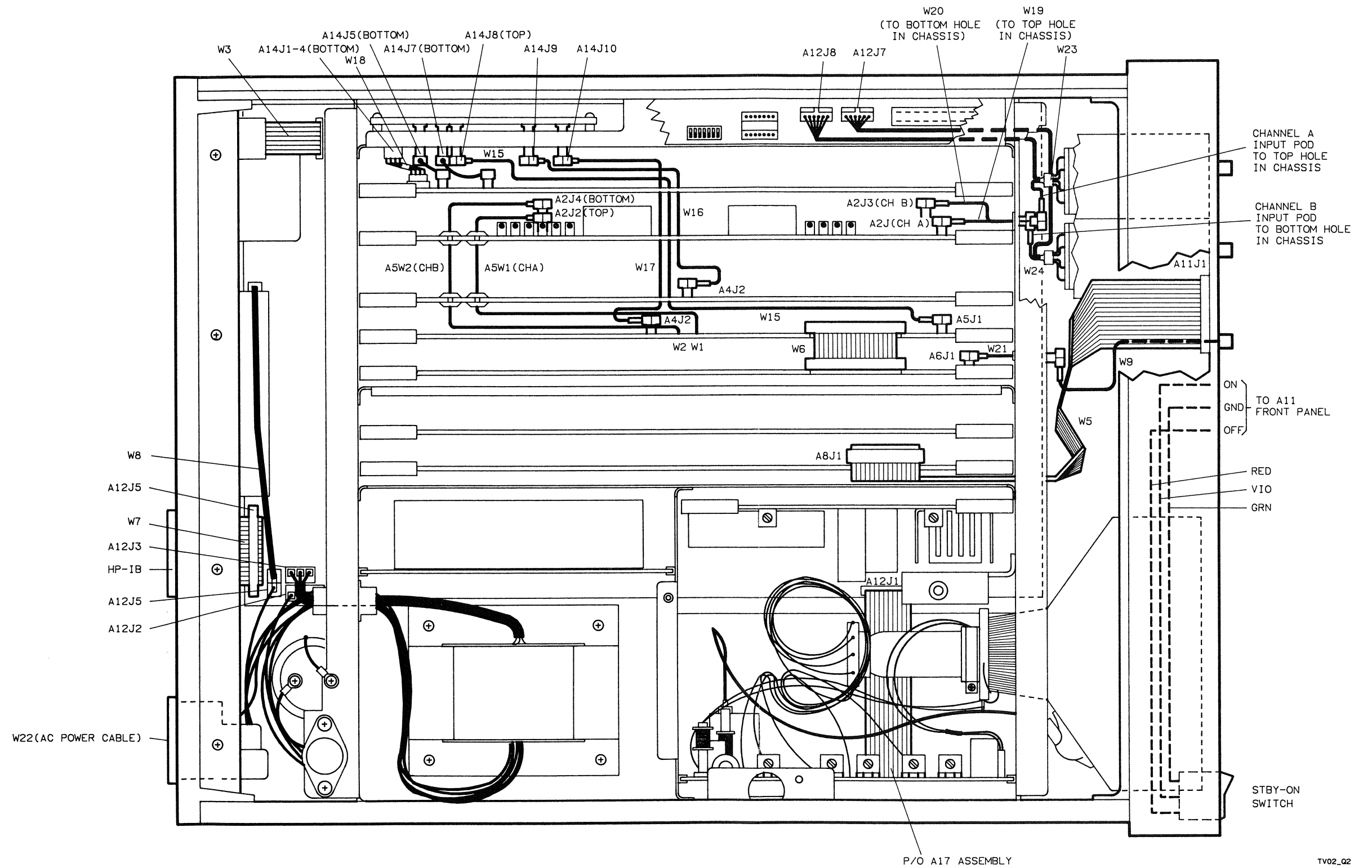
Figure 7N-1. HP 5371A Top Internal View
