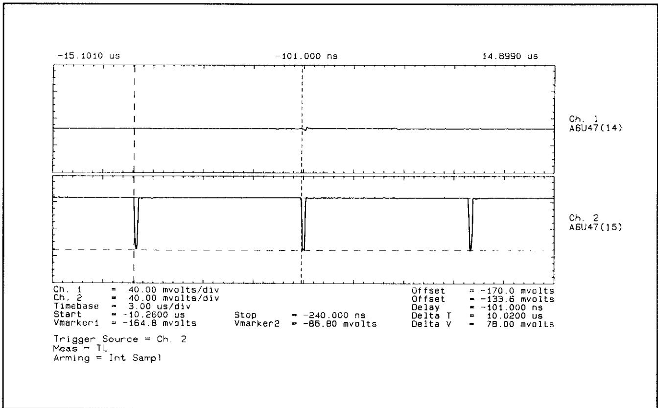
Figure 7F-17. Waveforms at A6U47(14,15)
