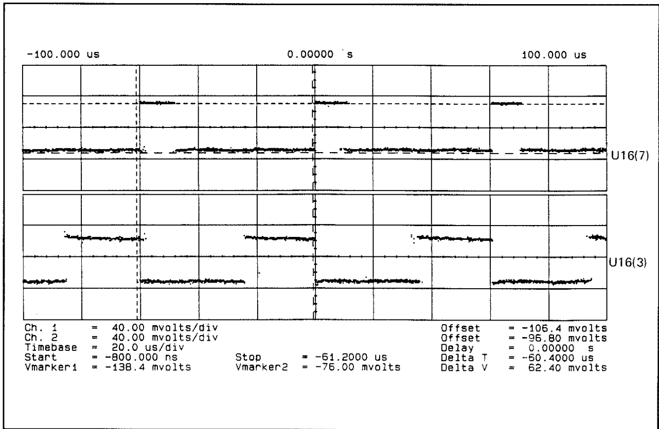
Figure 7D-13. Waveforms at A4U16(7) and A4U27(7)
