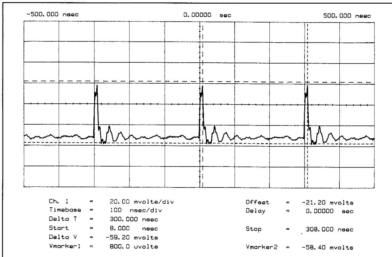
Figure 7D-10. IT1 (TP3) and IT2 (TP5) Waveforms
