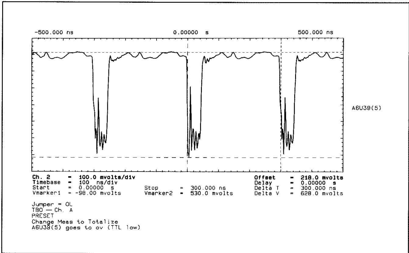
Figure 7F-29. Waveforms at A6U39(5)
