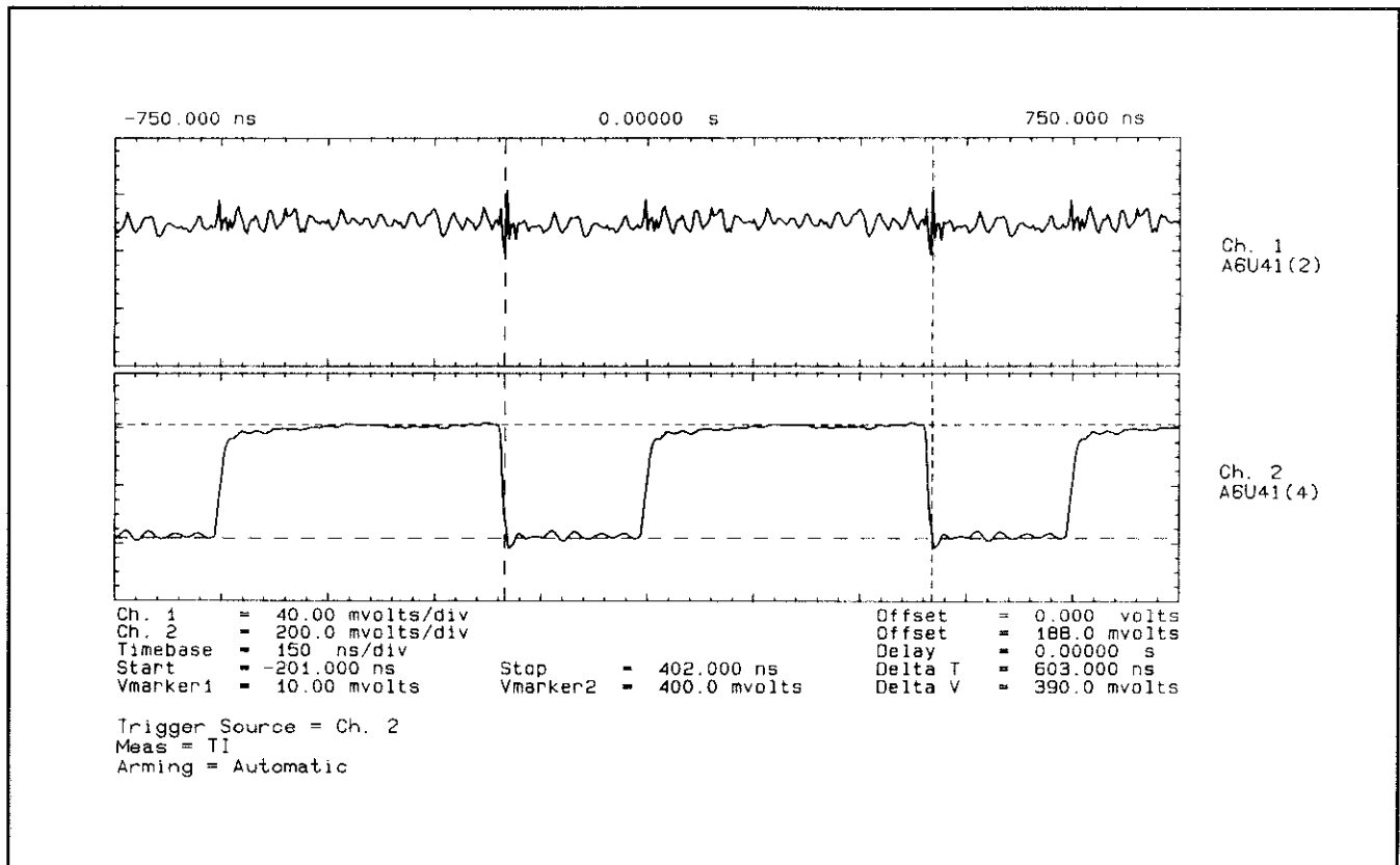
Figure 7F-13. Waveforms at A6U41(2,4) with Arming set to Automatic
