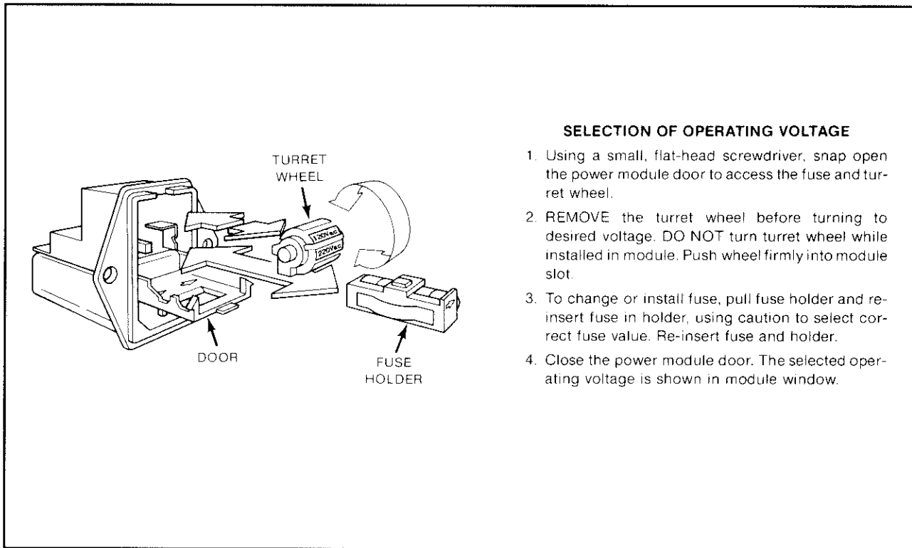
Figure 7-4. Line Voltage Selection Using A16 Power Module Turret Wheel
