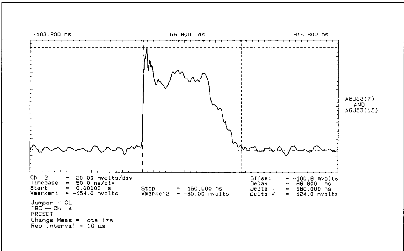
Figure 7F-24. Waveforms at A6U53(7,15) in Totalize Mode
