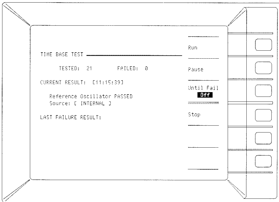
Figure 7A-2. Diagnostic Test Screen
