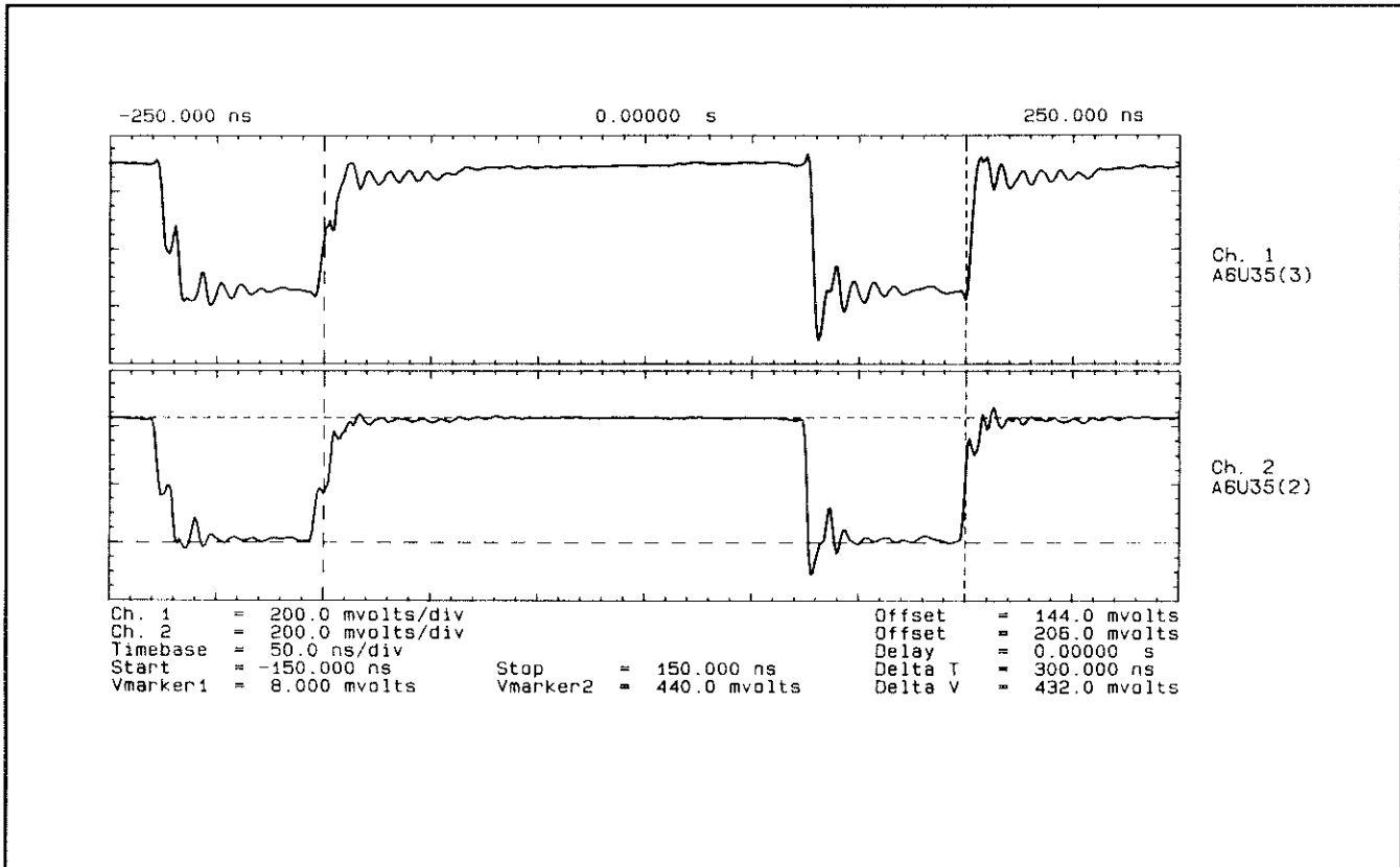
Figure 7F-10. Waveforms at A6U35(2,3)
