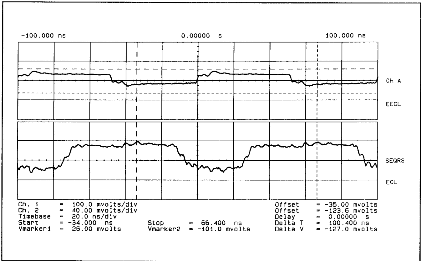
Figure 7E-11. Waveform at A5U29(A4) and A5U29(C11)
