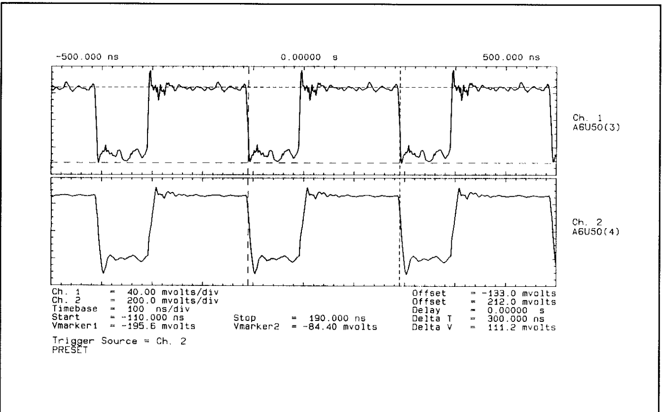
Figure 7F-16. Waveforms at A6U50(3,4)
