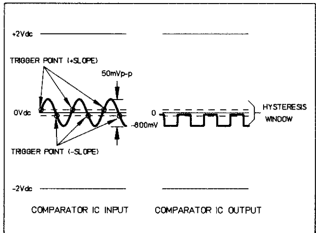
(B) -1 VDC OFFSET
