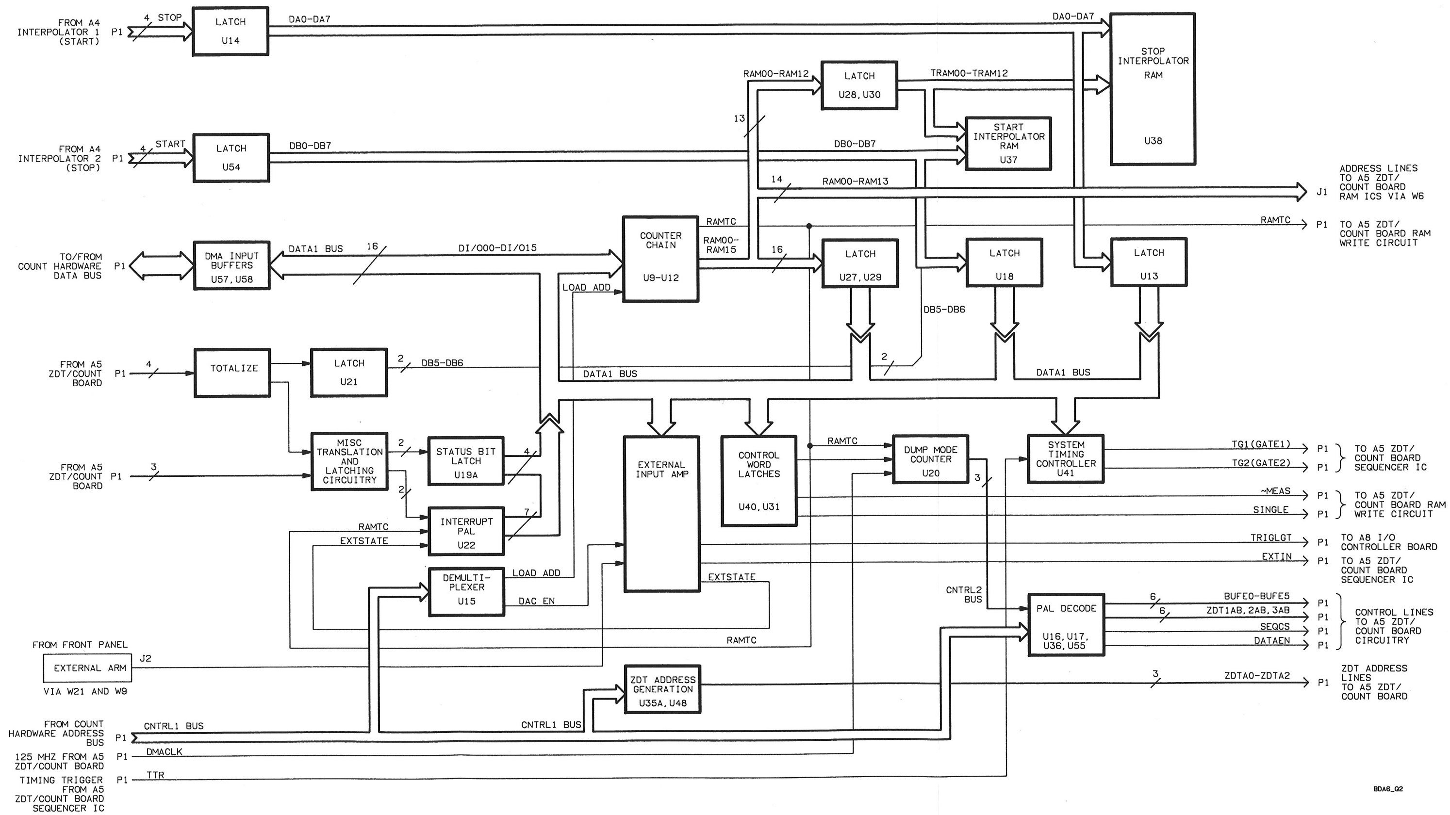
Figure 7F-1. A6 DMA/Gate Board Block Diagram
