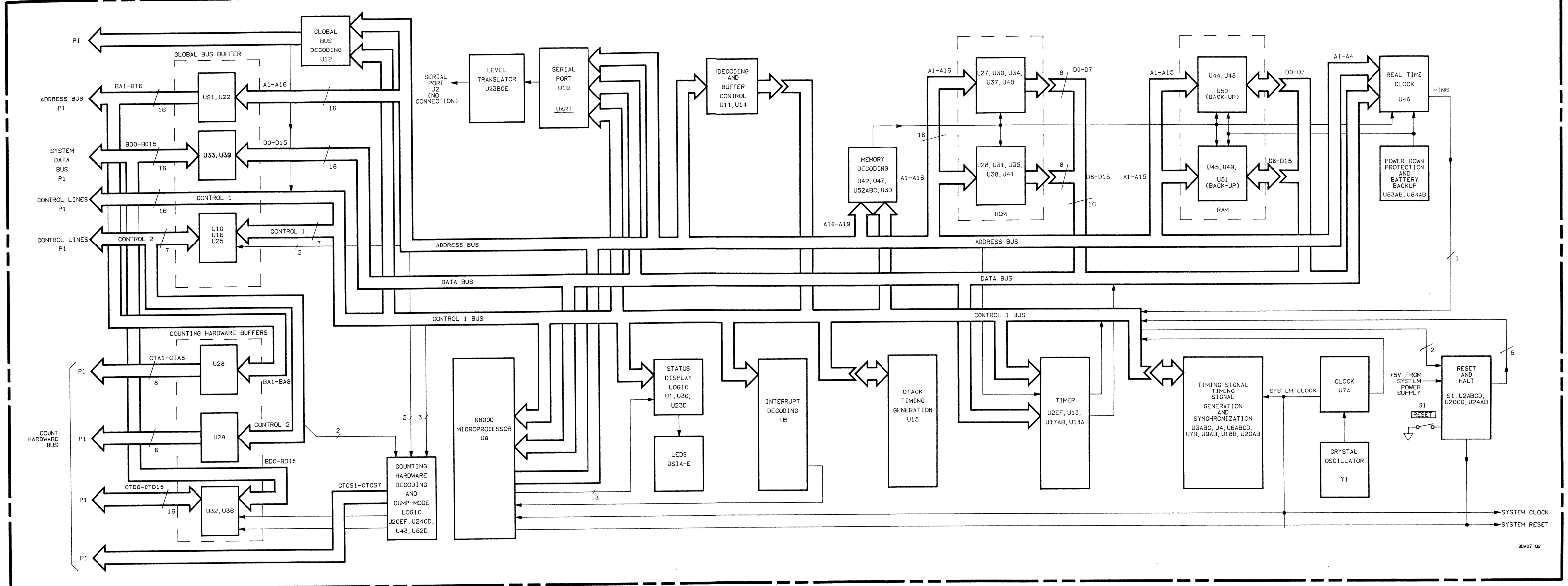
Figure 7G-1. A7 Processor Board Block Diagram
