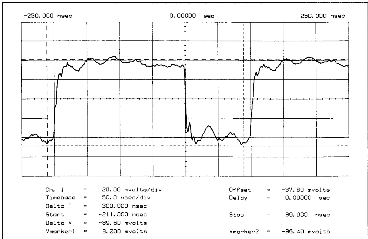
Figure 7D-6. IT1 and IT2 Waveforms
