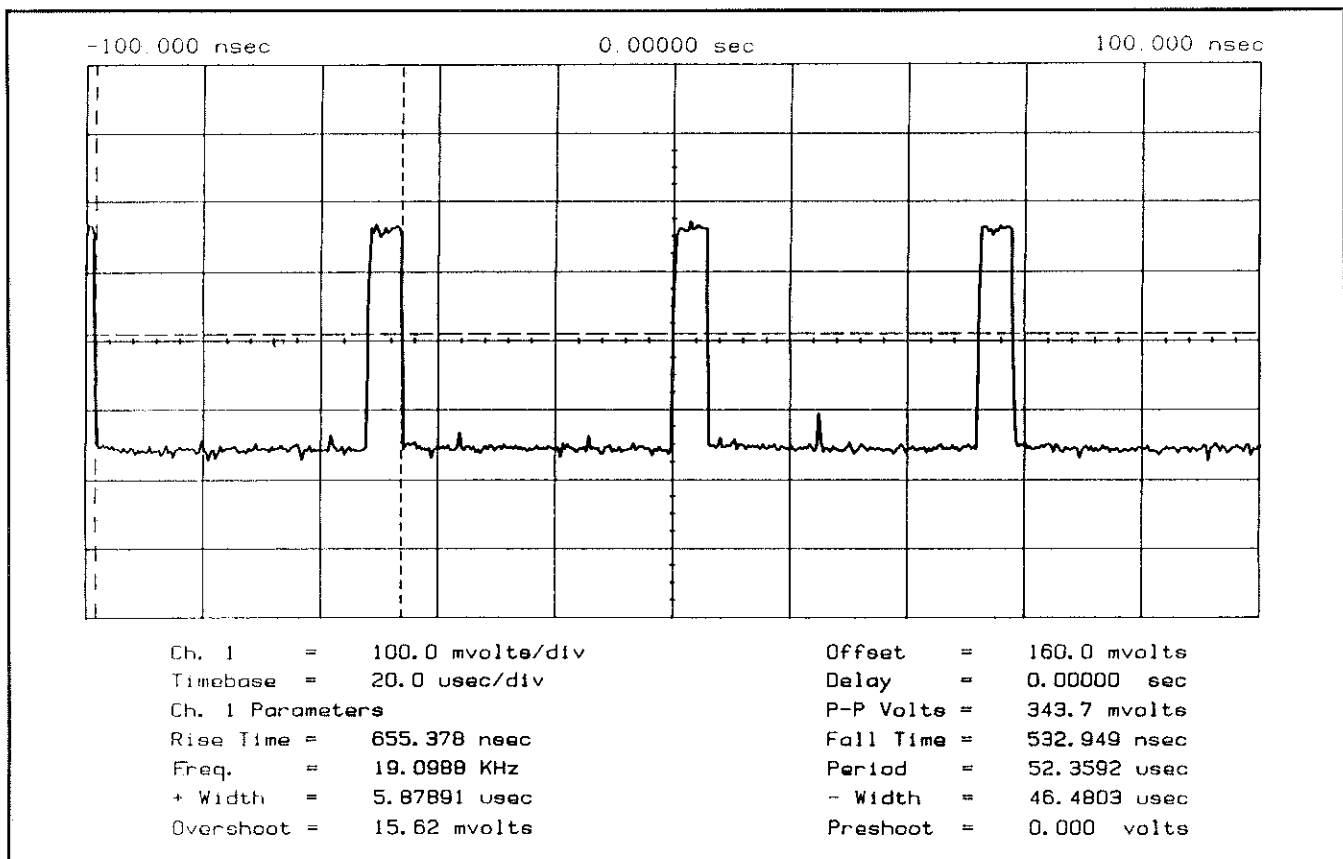
Figure 7H-2. HS Signal at A8U12(25)
