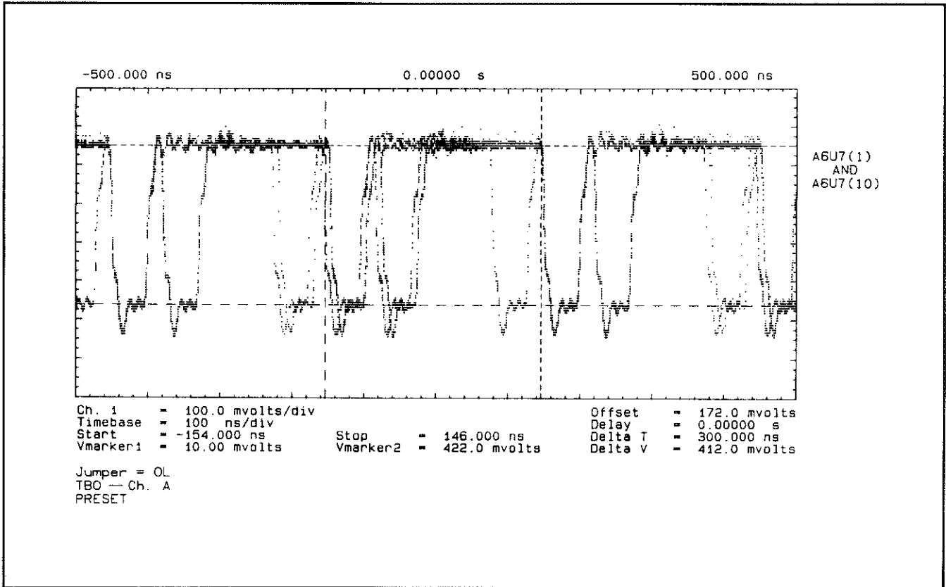
Figure 7F-19. Waveforms at A6U7(1,10)
