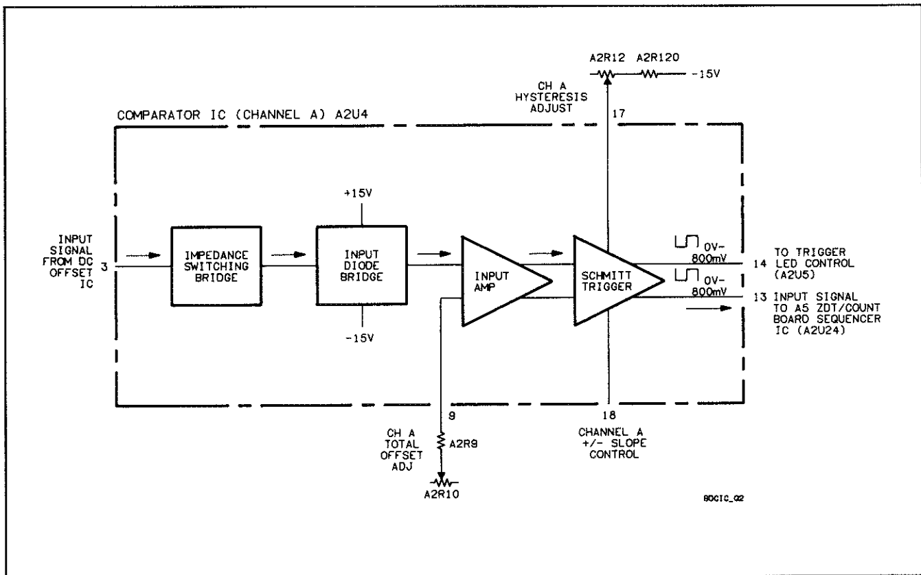
Figure 7C-2. Comparator IC Simplified Block Diagram
