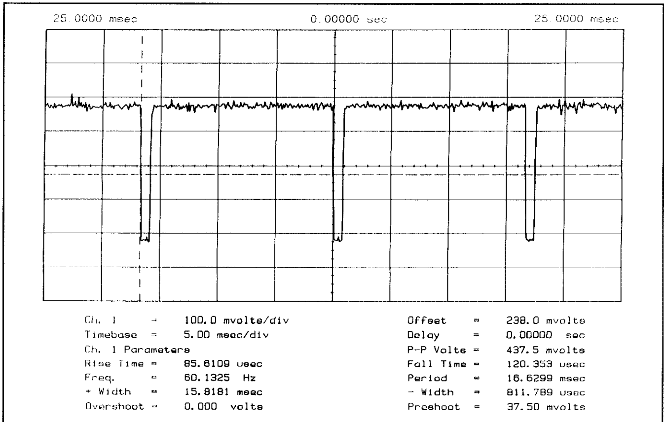
Figure 7H-3. VS Signal at A8U12(40)
