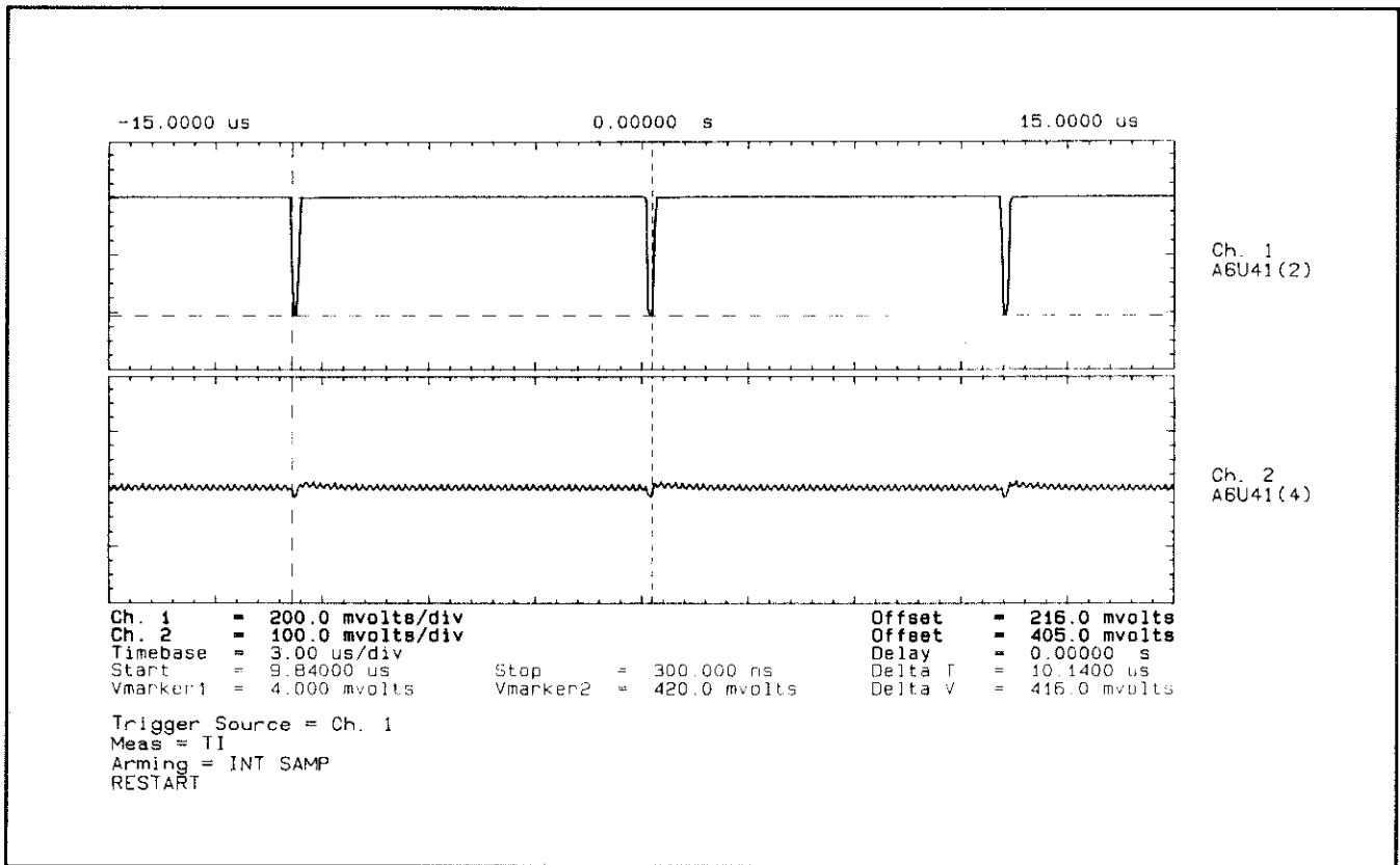
Figure 7F-12. Waveforms at A6U41(2,4)
