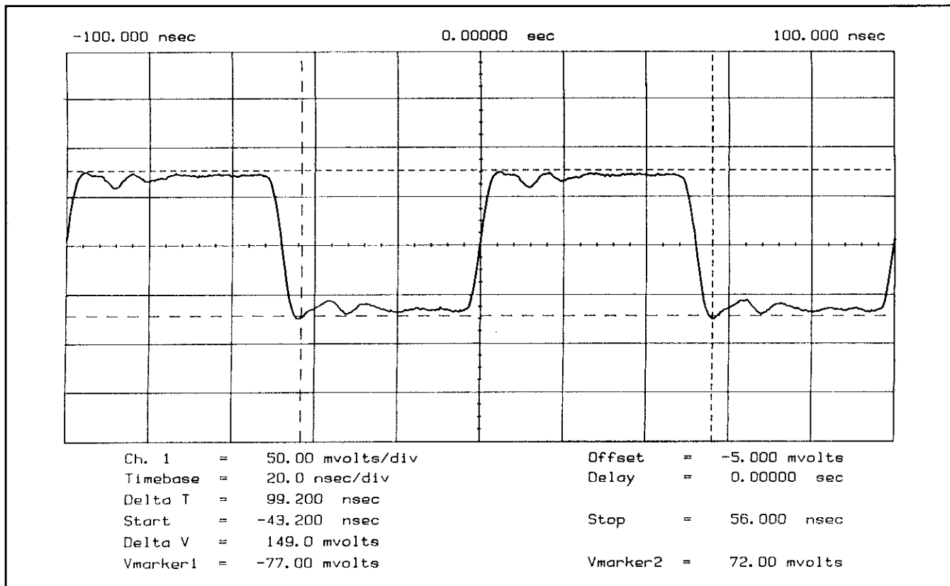
Figure 7C-6. A2U2(2) [A2U14(2)] 10MHz Square Wave
