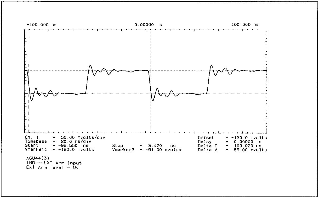
Figure 7F-18. Waveforms at A6U44(3)
