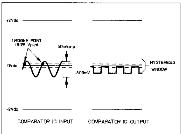
(F) TRIGGER LEVEL SETTING: 80% +SLOPE
