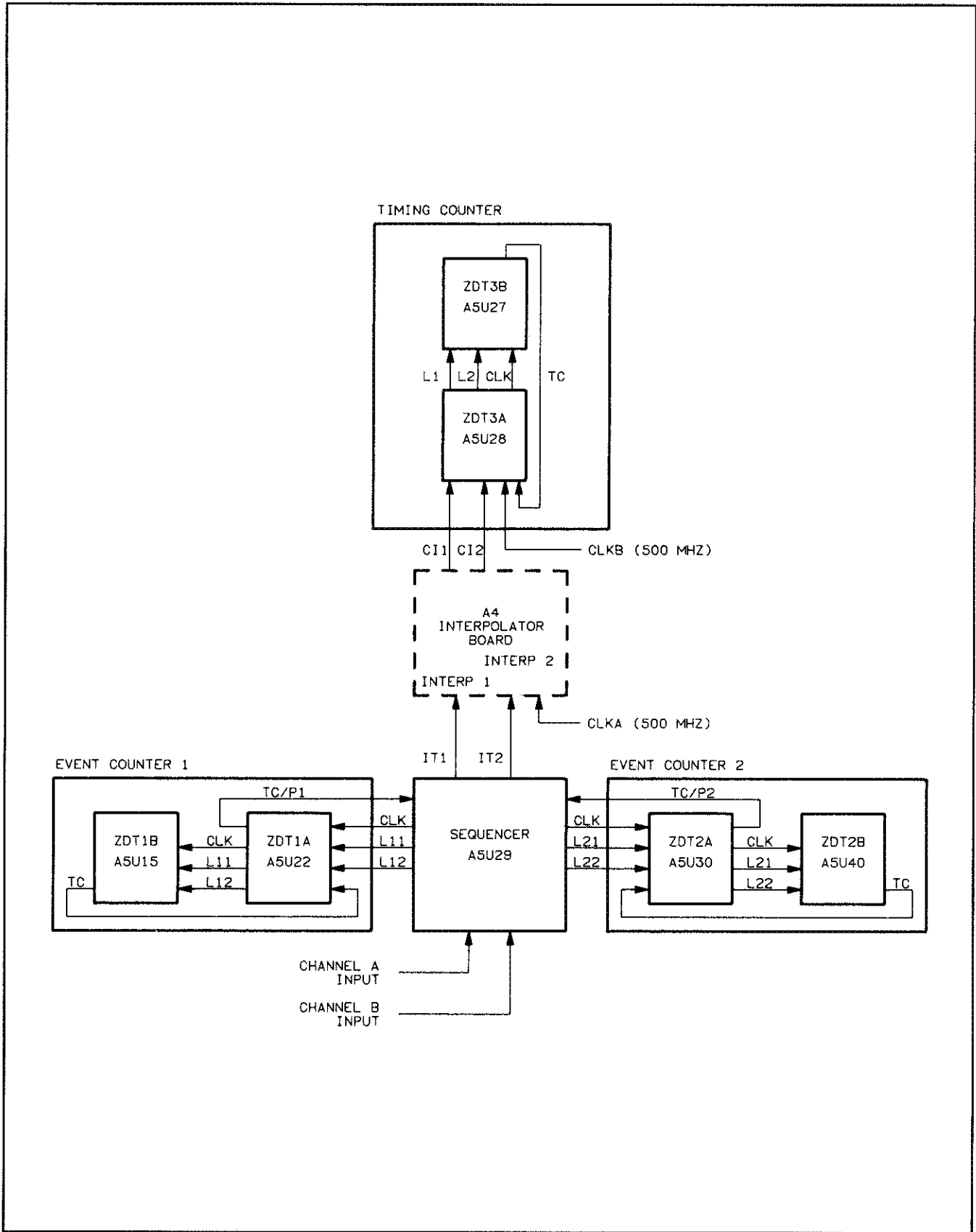
Figure 7E-1. Counting Chains
