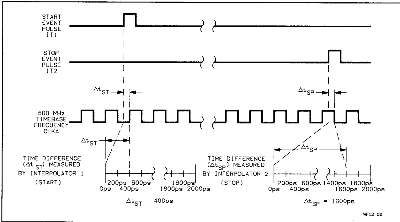
Figure 7D-1. Interpolator Timing Diagram
