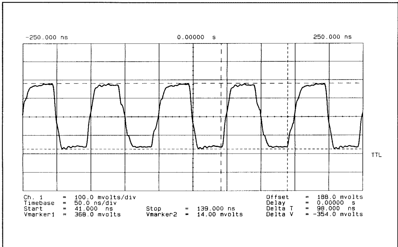
Figure 7E-7. RAM_WR (TIM) Signal at A5U31(27)
