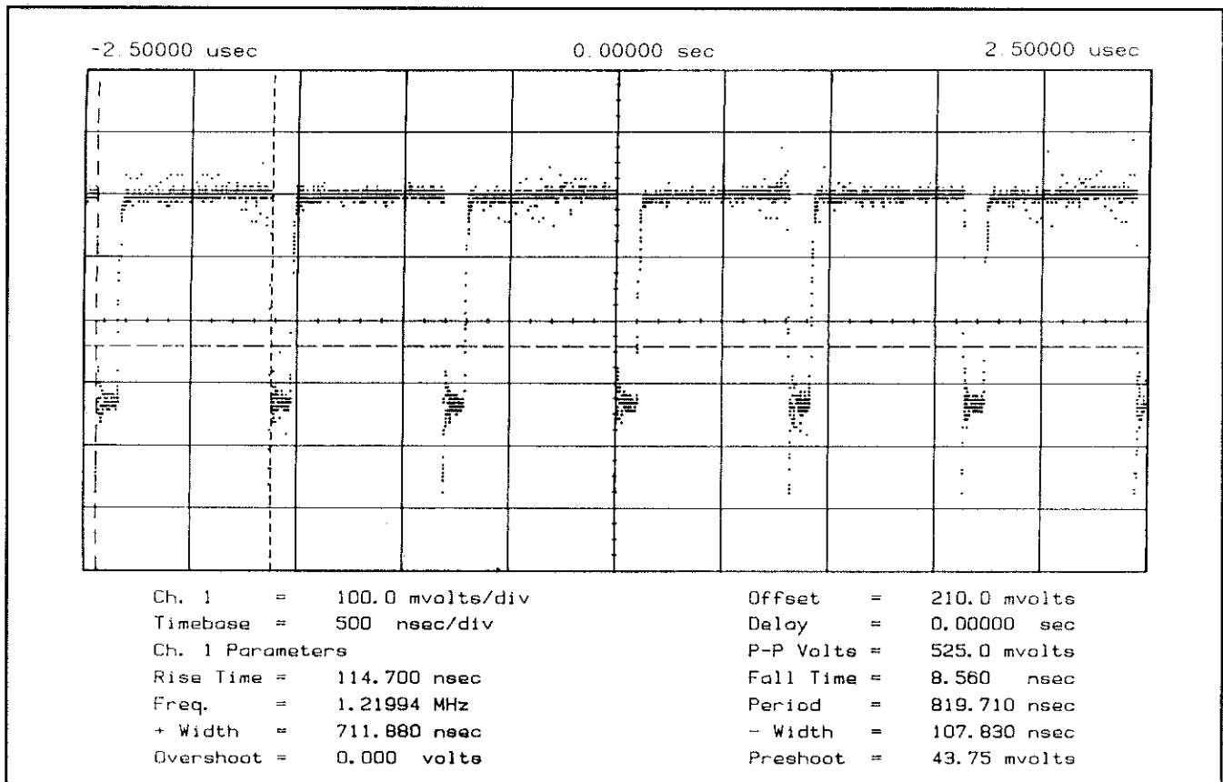
Figure 7H-4. 1MHz Signal at A8U14(15)
