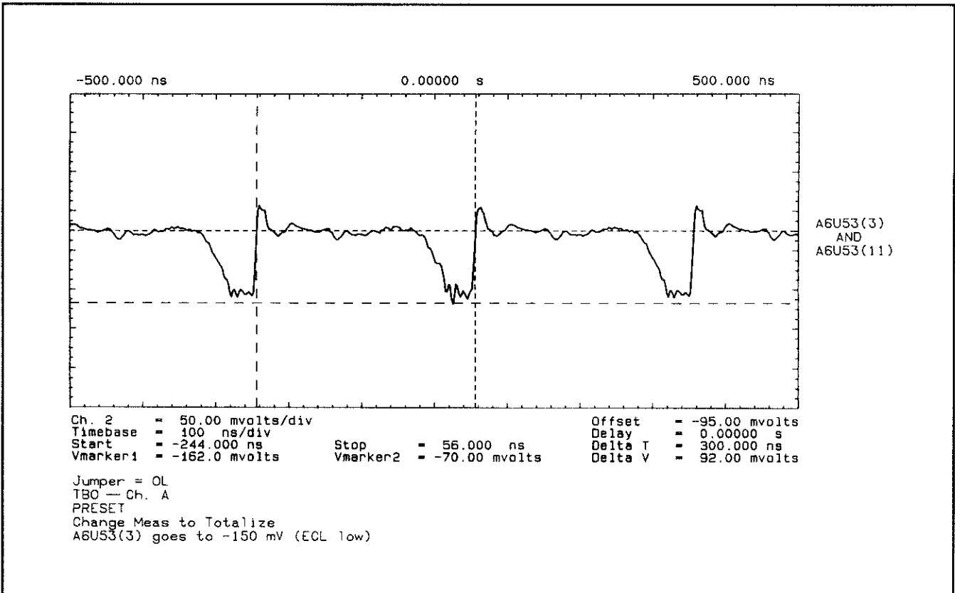
Figure 7F-25. Waveforms at A6U53(3,11)
