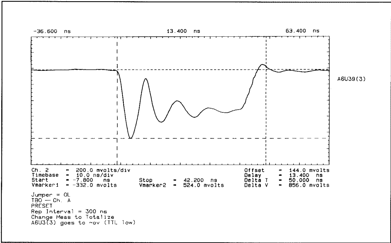
Figure 7F-27. Waveform at A6U39(3)
