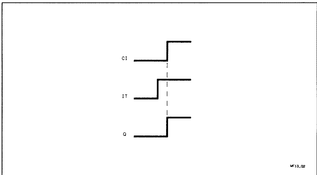
Figure 7D-2. IT Leading CI
