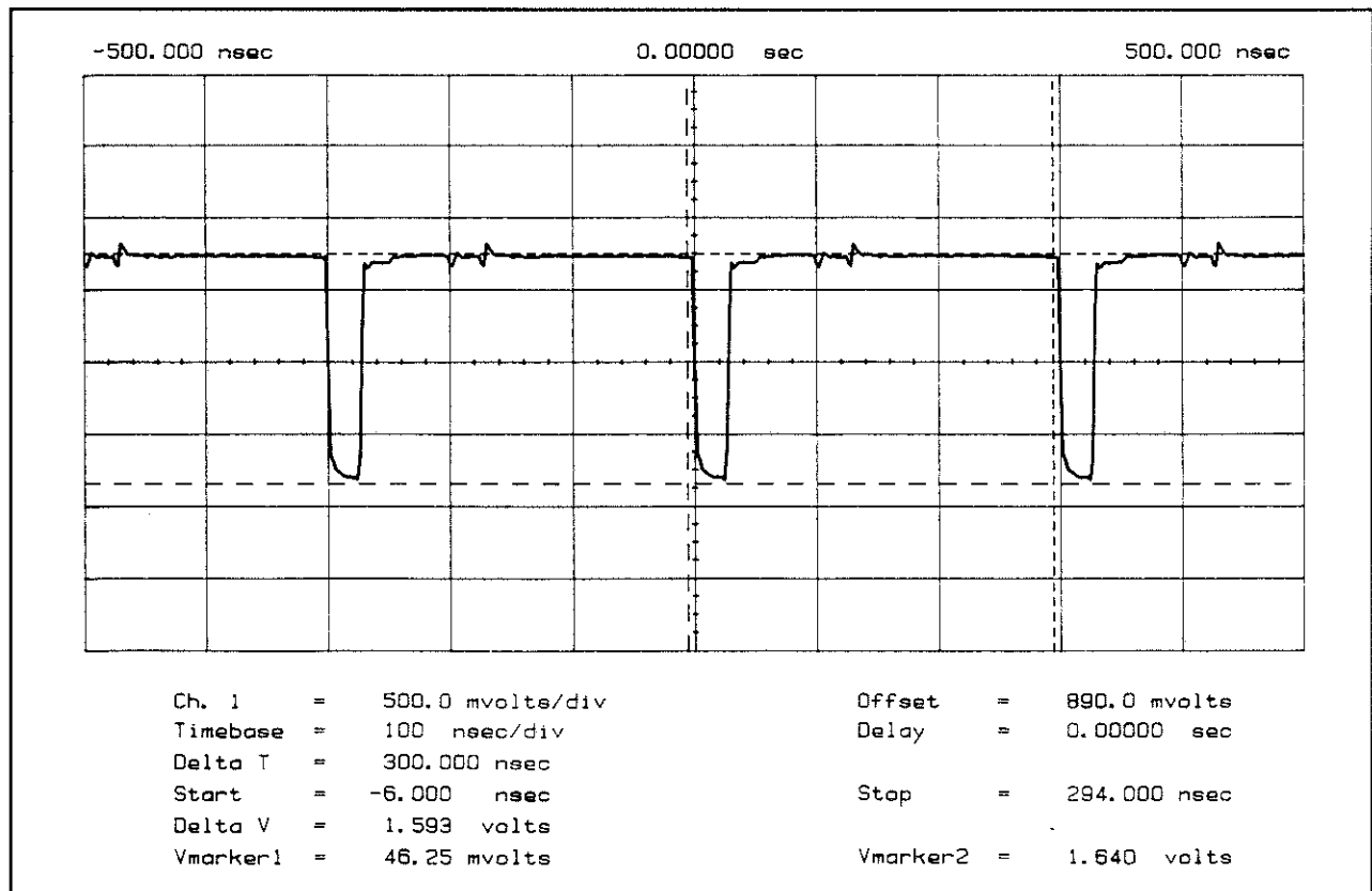
Figure 7D-5. GATE 1 and GATE 2 Signals at Rear Panel
