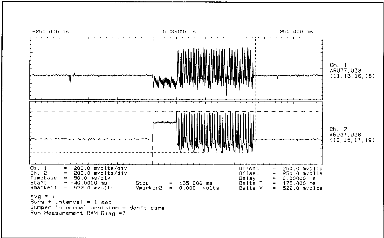
Figure 7F-6. Waveforms at A6U37 and A6U38
