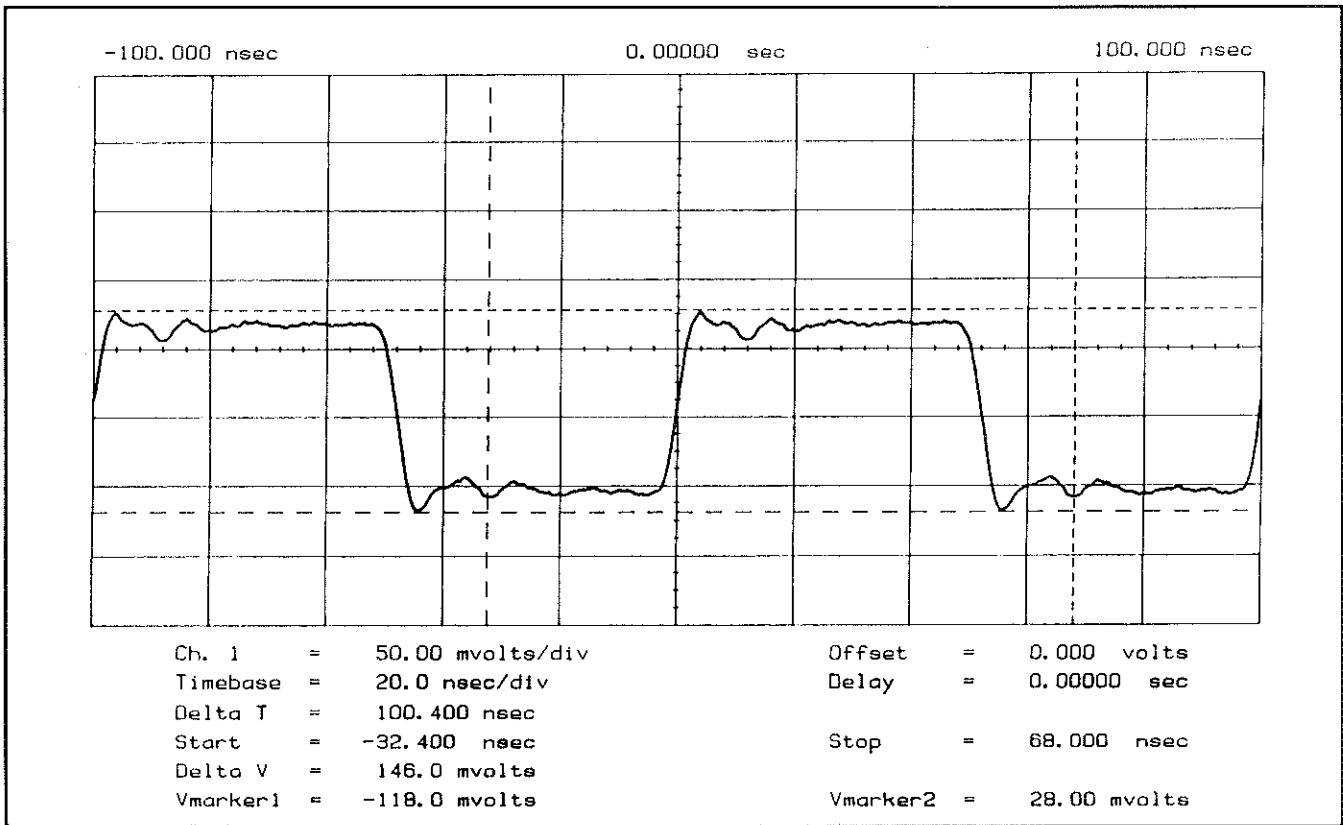
Figure 7C-8. Comparator Input Pin A2U4(3) [A2U15(3)] Waveform
