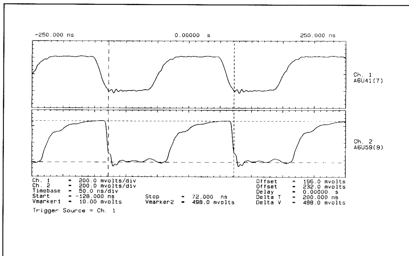
Figure 7F-11. Waveforms at A6U41(7) and A6U59(9)
