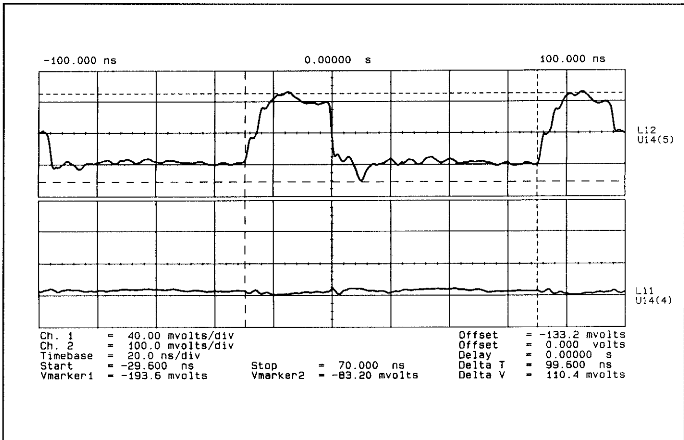
Figure 7E-8. Latch 11 and Latch 12
