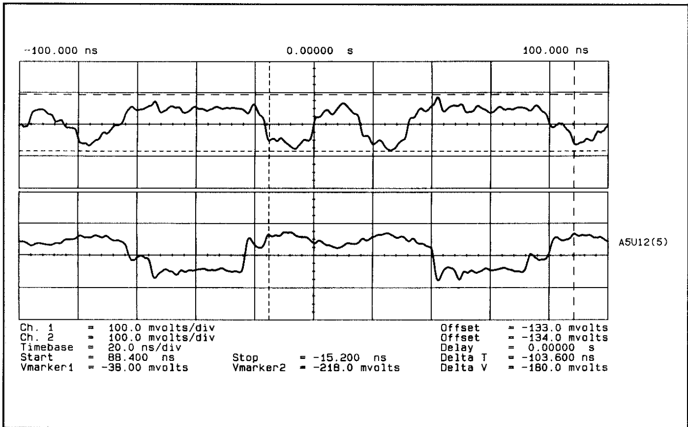
Figure 7E-10. Waveform at A5U12(5)
