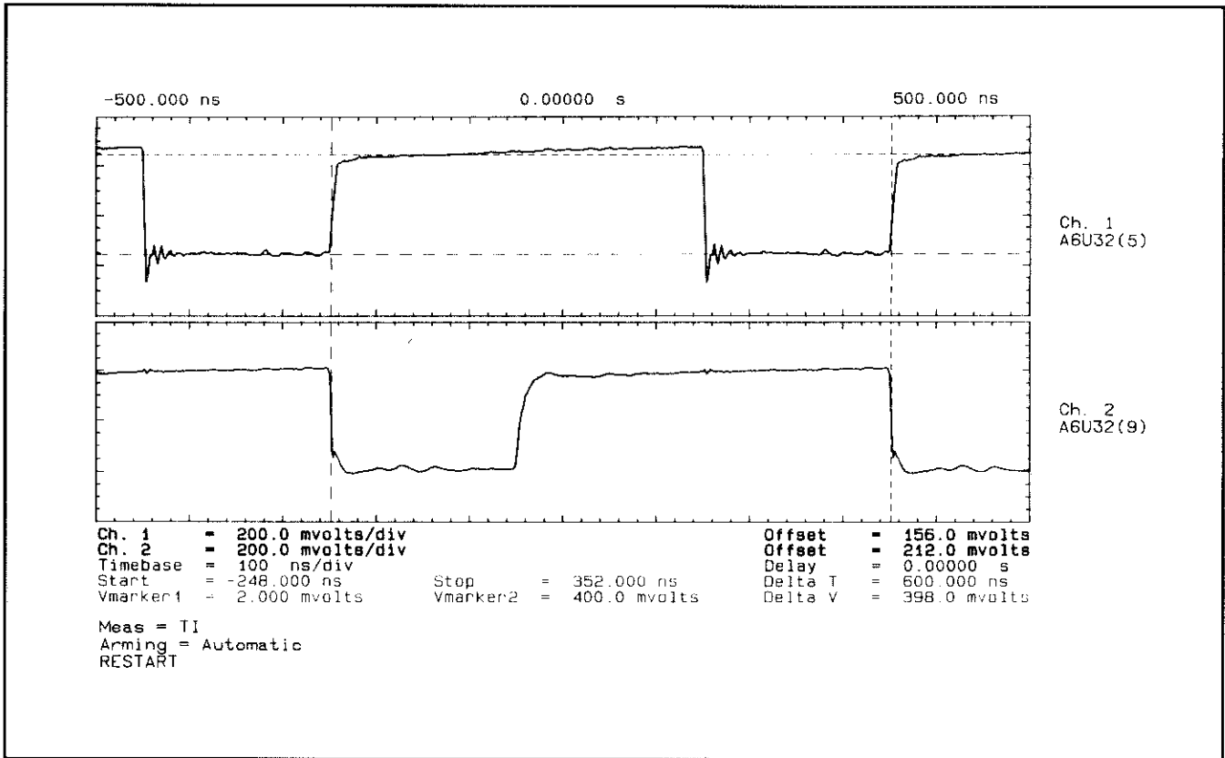
Figure 7F-14. Waveforms at A6U32(5,9)
