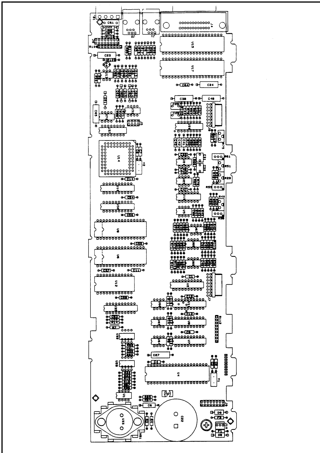
Figure 6-8. HP-IB Board (A8) Component Location
