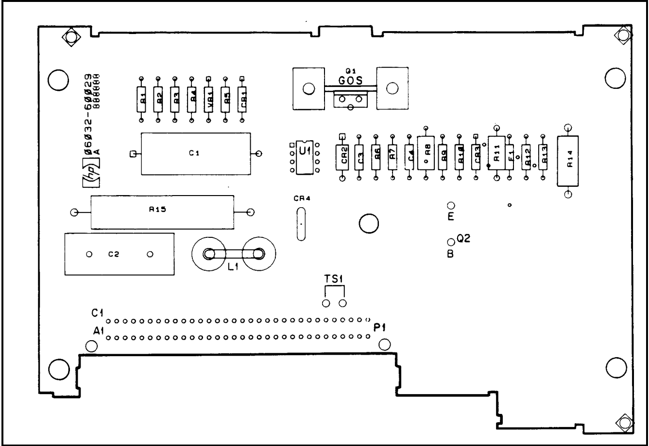
Figure 6-6C. 6032A Diode Board (A5) Component Location
