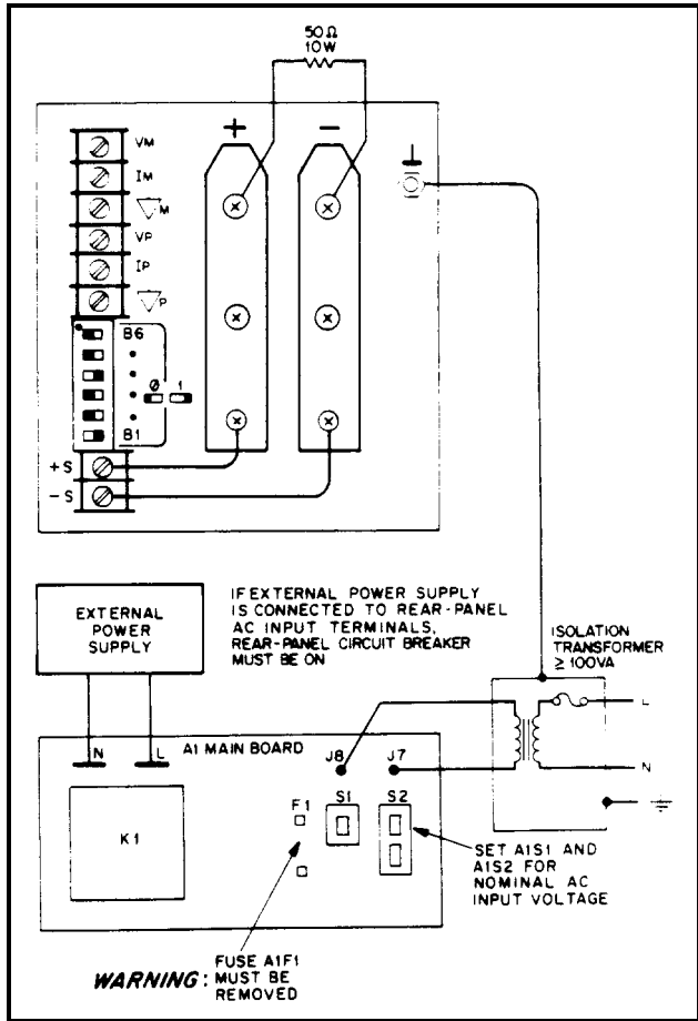
Figure 3 5. Main Troubleshooting Setup
