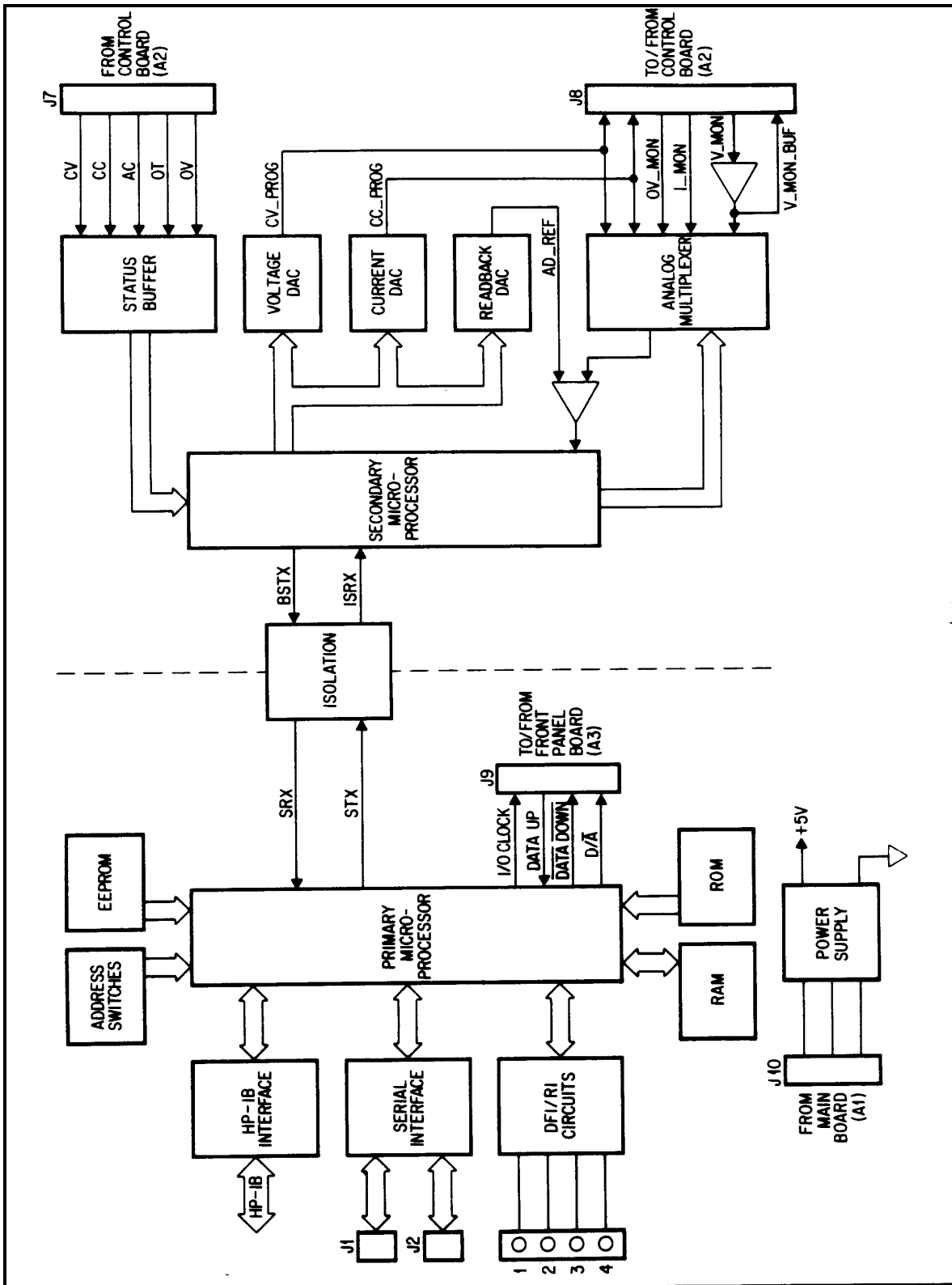
Figure 4-1. HP-IB Block Diagram
