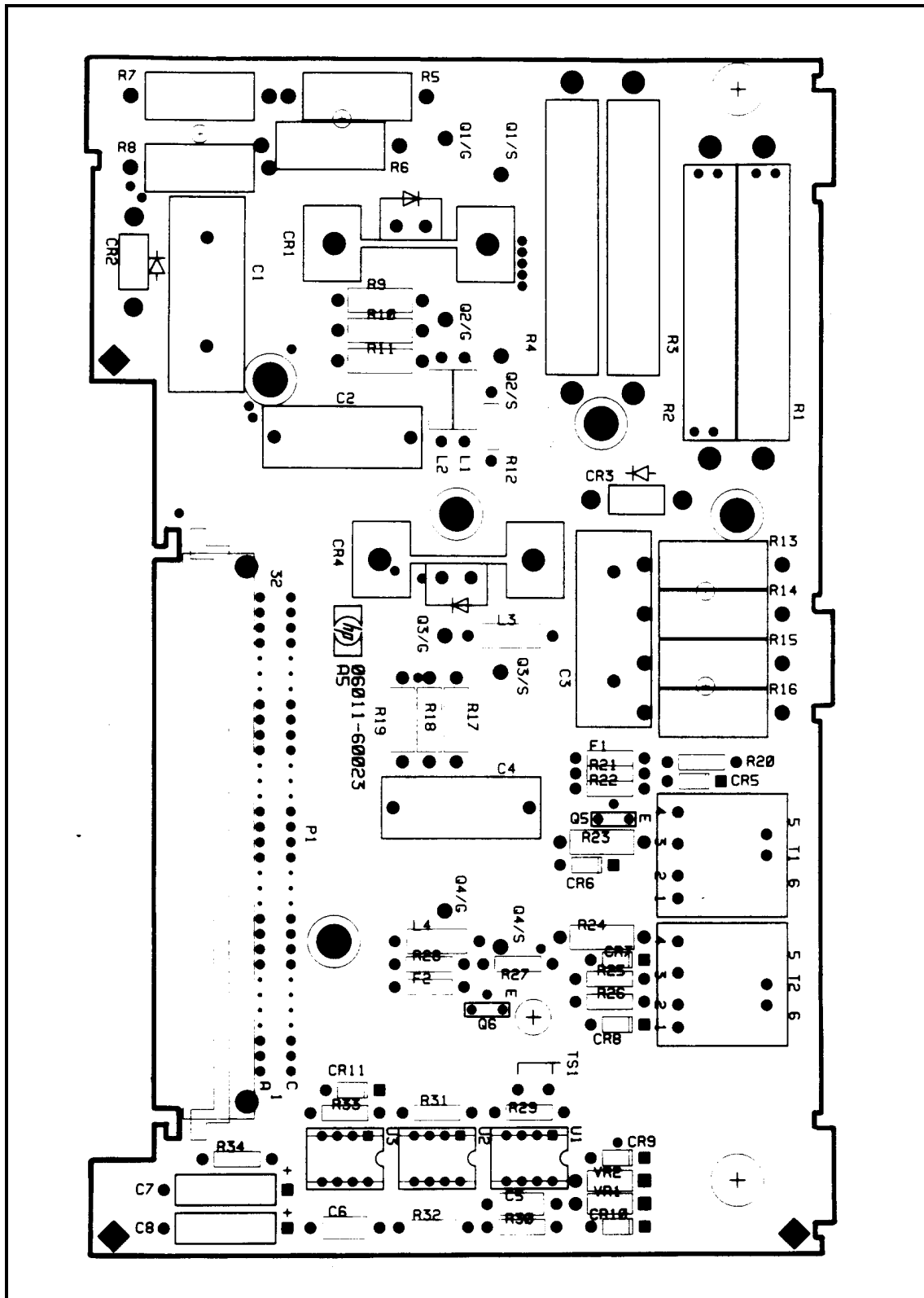
Figure 6-5. FET Board (A4) Component Location
