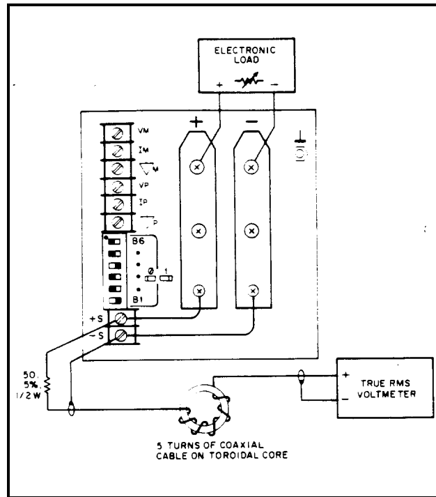
Figure 2-6. RMS Measurement Test Setup, CV PARD Test
