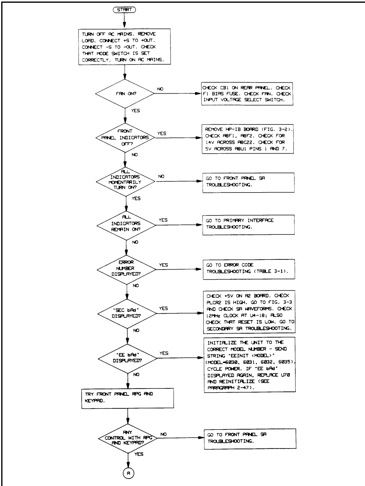
Figure 3-1. Troubleshooting Isolation
