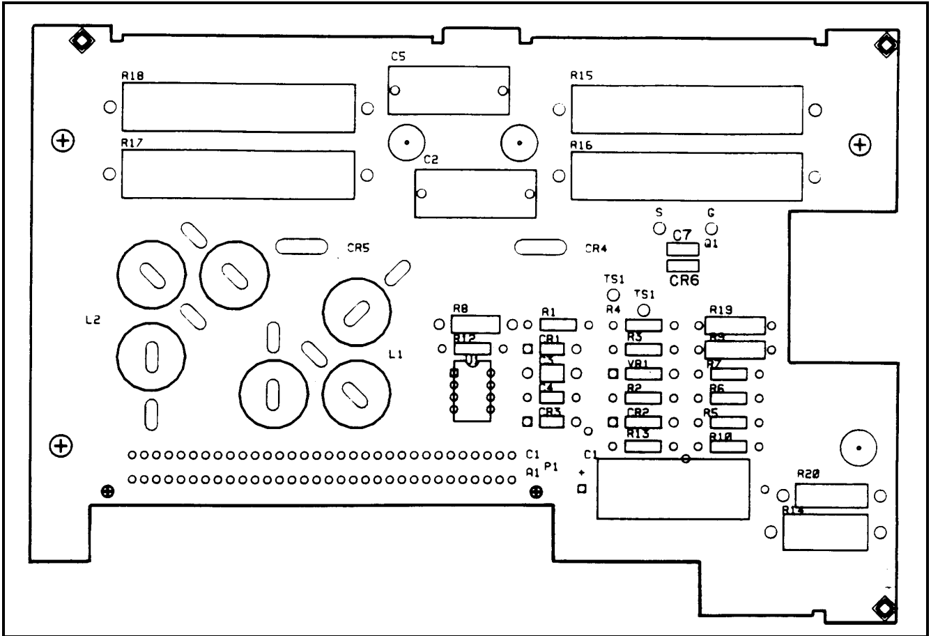
Figure 6-6A. 6030A/35A Diode Board (A5) Component Location
