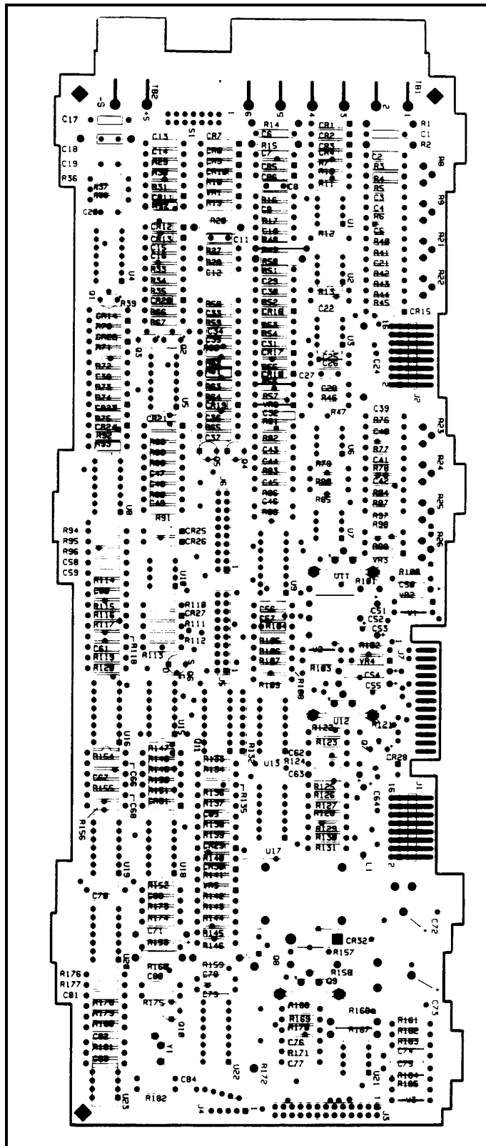
Figure 6-3. Control Board (A2) Component Location
