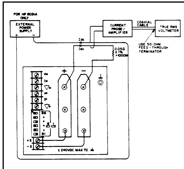
Figure 2-9. CC PARD Test Setup
