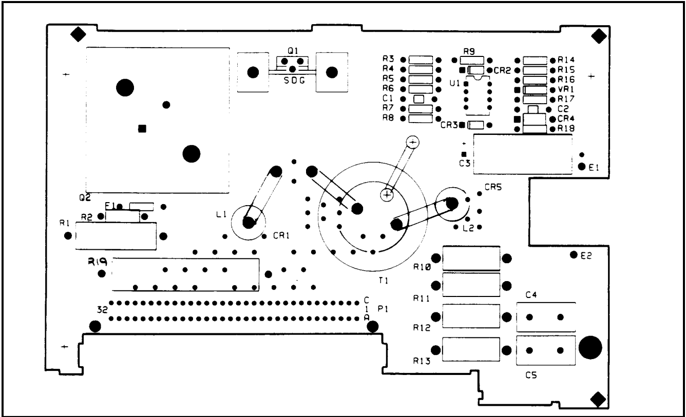
Figure 6-6B. 6031A Diode Board (A5) Component Location
