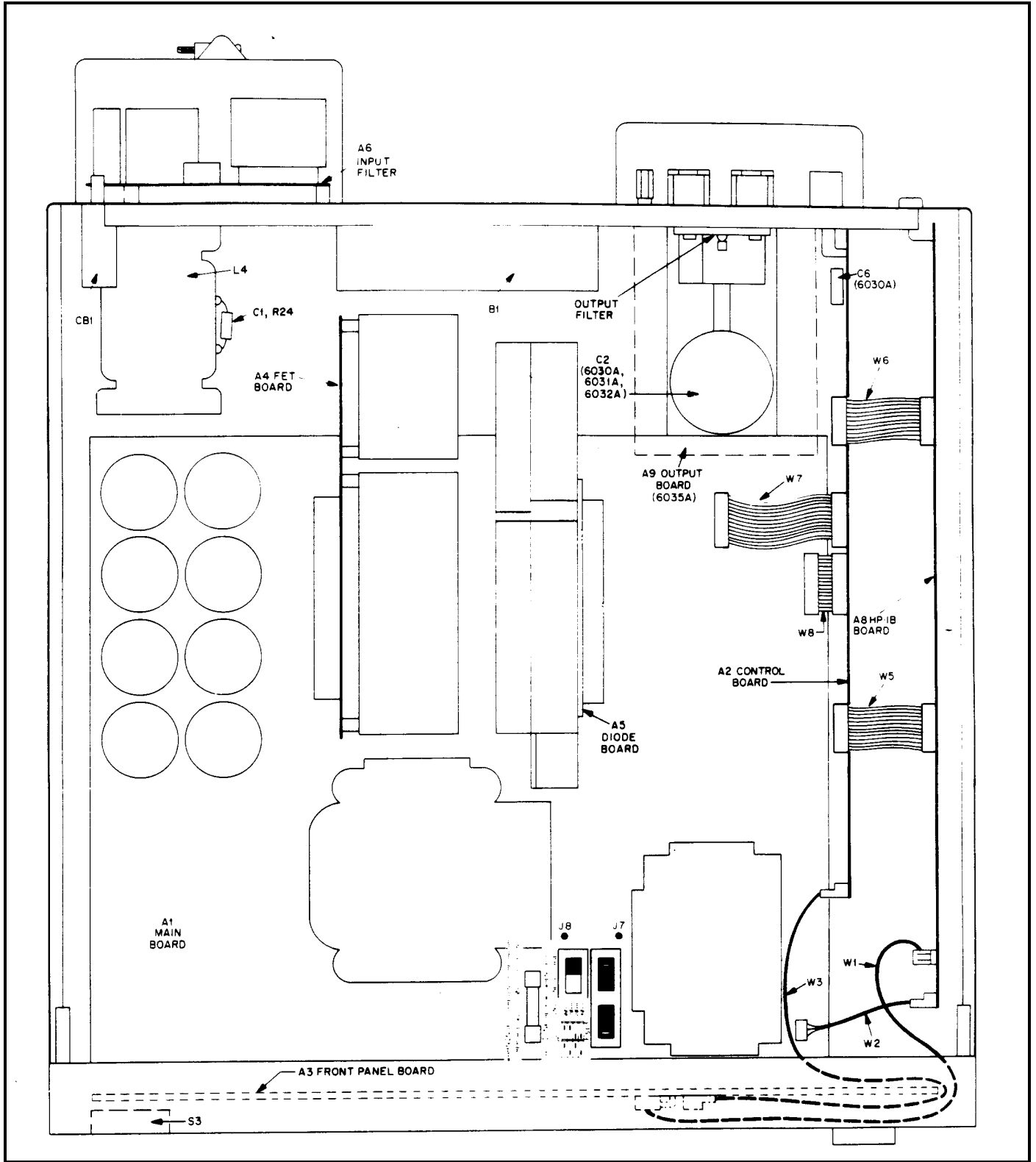
Figure 6-1. Top View, Top Covers Removed
