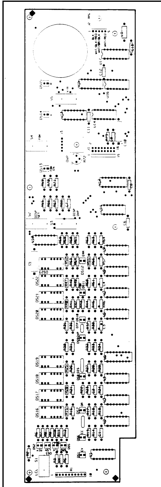
Figure 6-4. Front Panel Board (A3) Component Location
