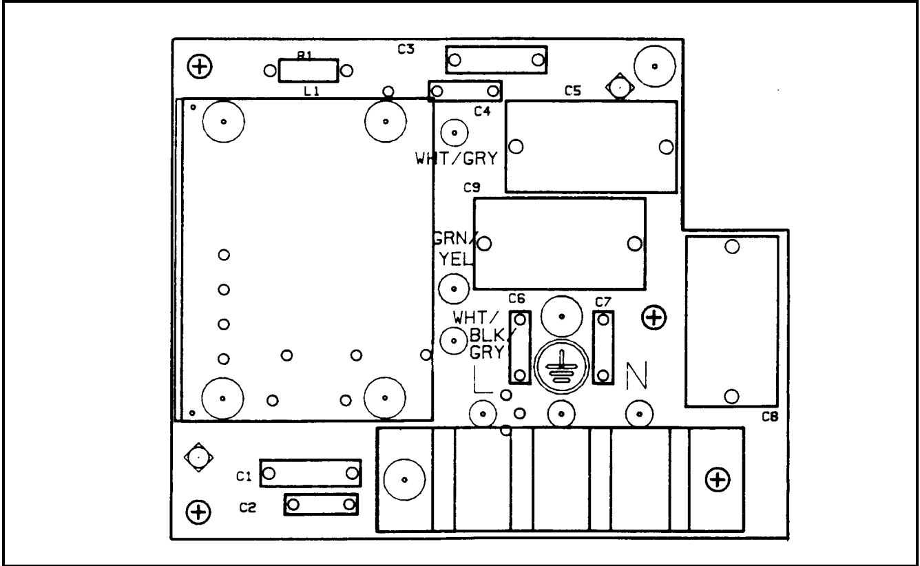
Figure 6-7. AC Input Filter (A6) Component Location
