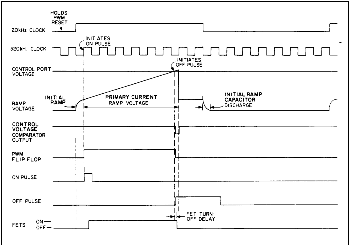
Figure 4-4. FET Control Signals Timing Diagram
