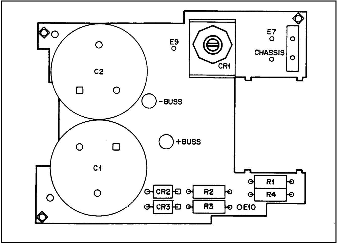
Figure 6-9. 6035A Output Board (A9) Component Location
