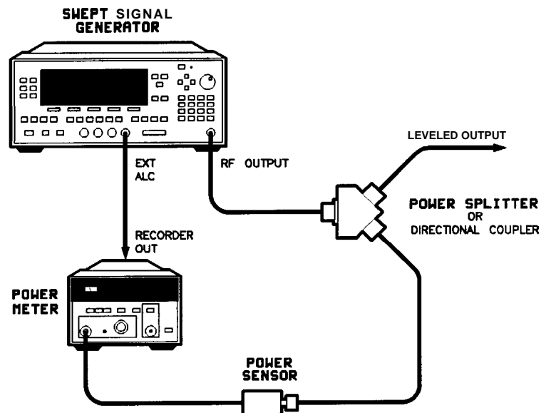
Figure I-13. Leveling with a Power Meter
