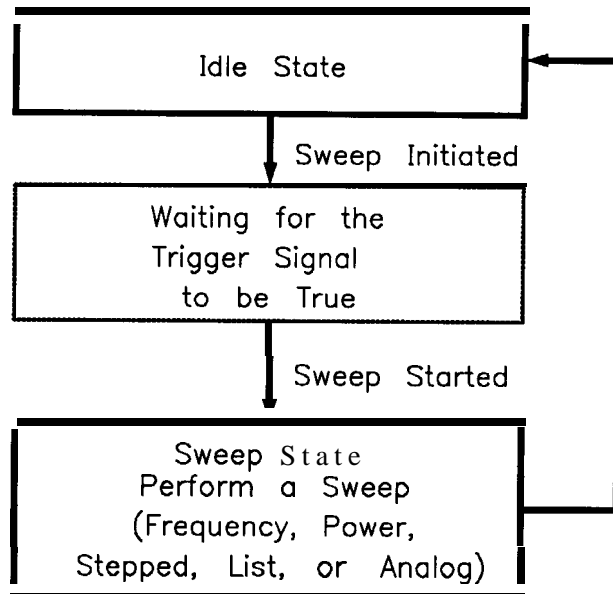
Figure I-42. HP 8380 Simplified Trigger Model
