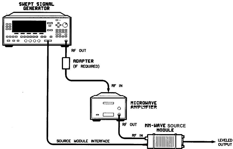
Figure I-15. MM-wave Source Module Leveling Using a Microwave Amplifier
