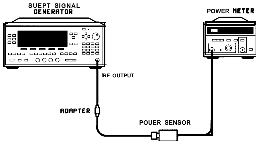
Figure I-10. Power Sweep and Power Slope Operation
