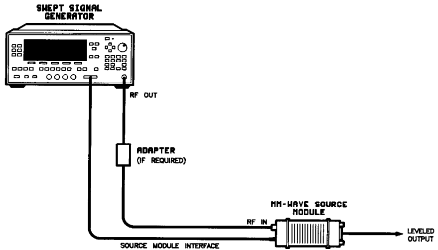
Figure I-14. MM-wave Source Module Leveling
