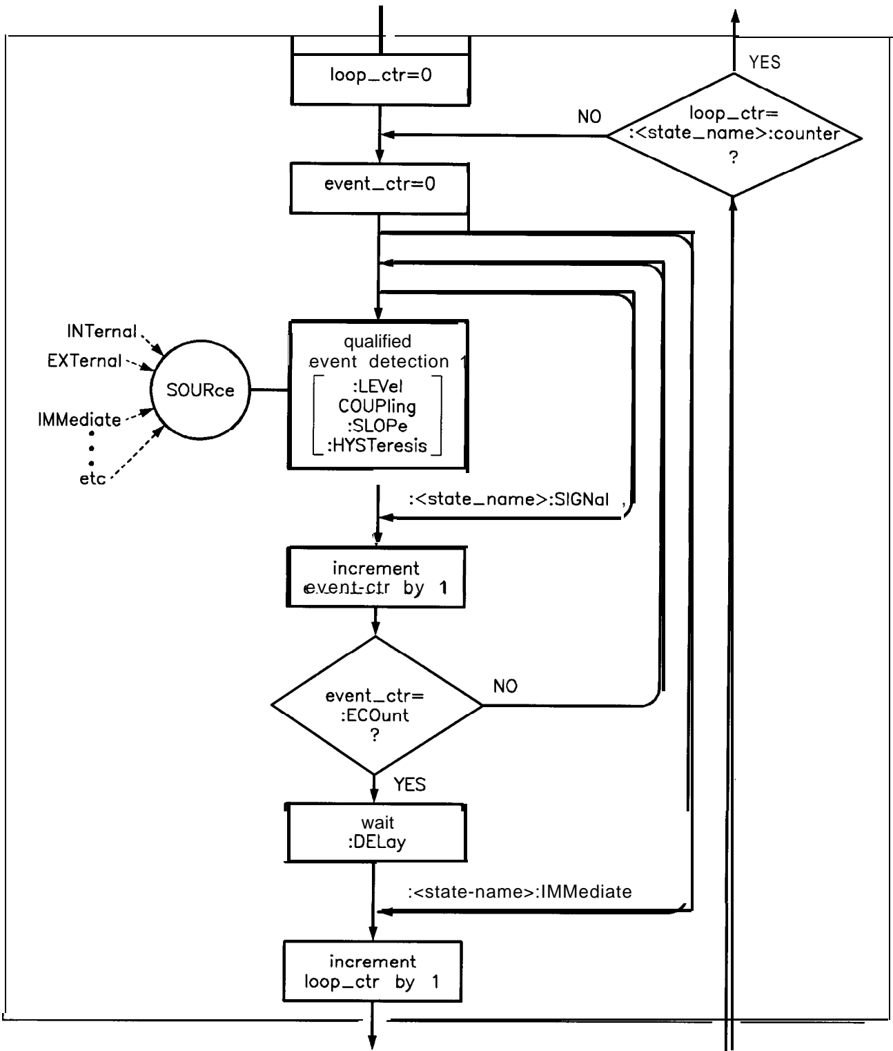
Figure I-38. Inside an Event Detection State
