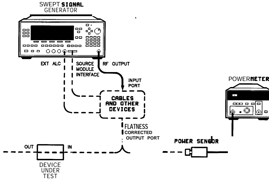
Figure I-19. Creating a User Flatness Array
