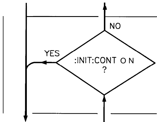
Figure I-37. Inside the Initiate State
