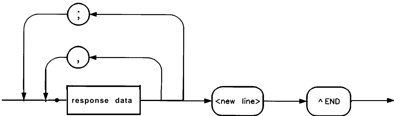
Figure I-32. Simplified Response Message Syntax
