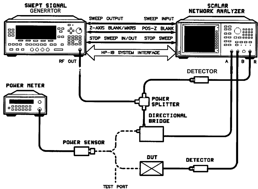
Figure I-2 1. Scalar System Configuration
