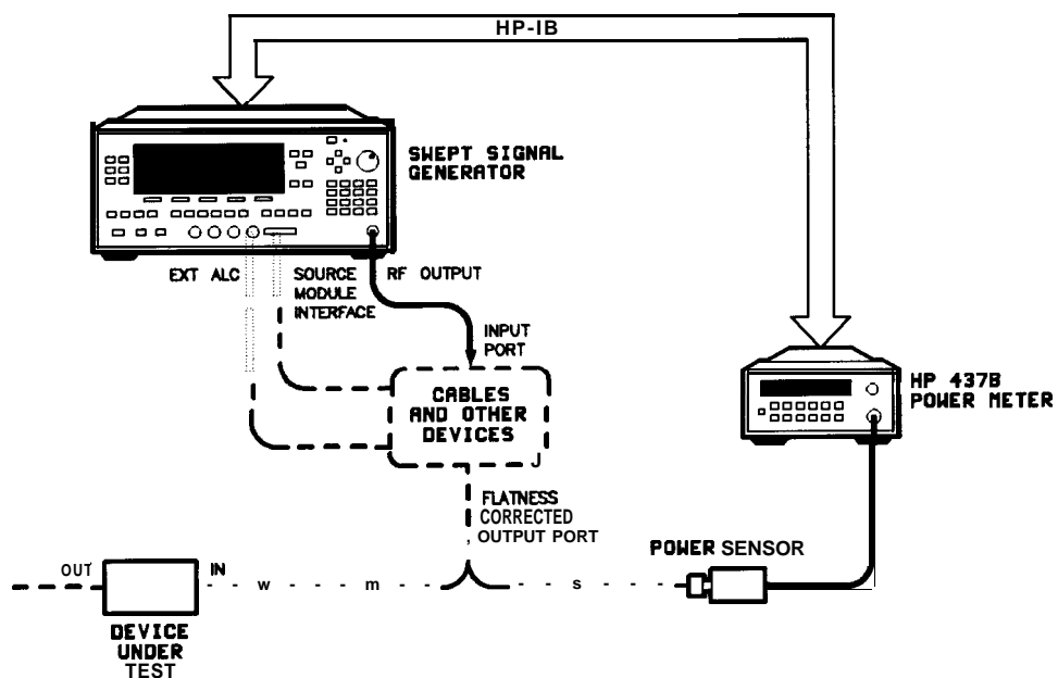
Figure F-1. Basic User Flatness Configuration Using an HP 4378 Power Meter
