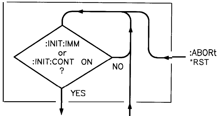
Figure I-36. Inside the Idle State
