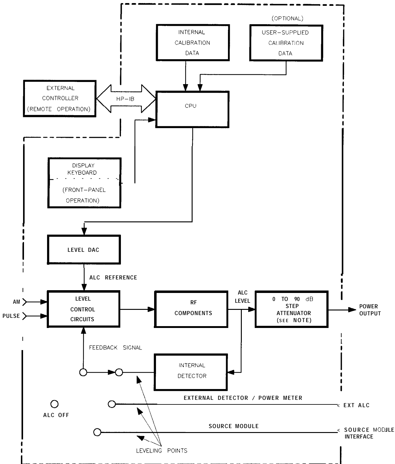
Figure A-1. ALC System Simplified Block Diagram
