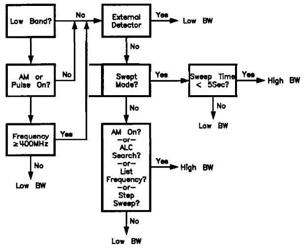
Figure I-23. Decision Tree for ALC Bandwidth Selection
