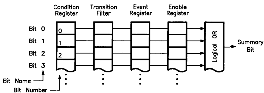
Figure I-33. Generalized Status Register Model
