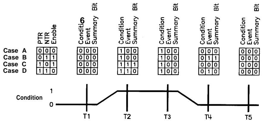
Figure I-34. Typical Status Register Bit Changes
