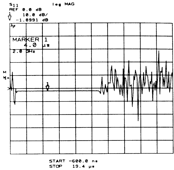
Figure 5-5. Pulse Profile, S_{11}
