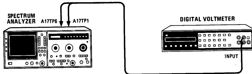
Figure 5-27. +10V Reference and Digital Readout Adjustment Test Setup
