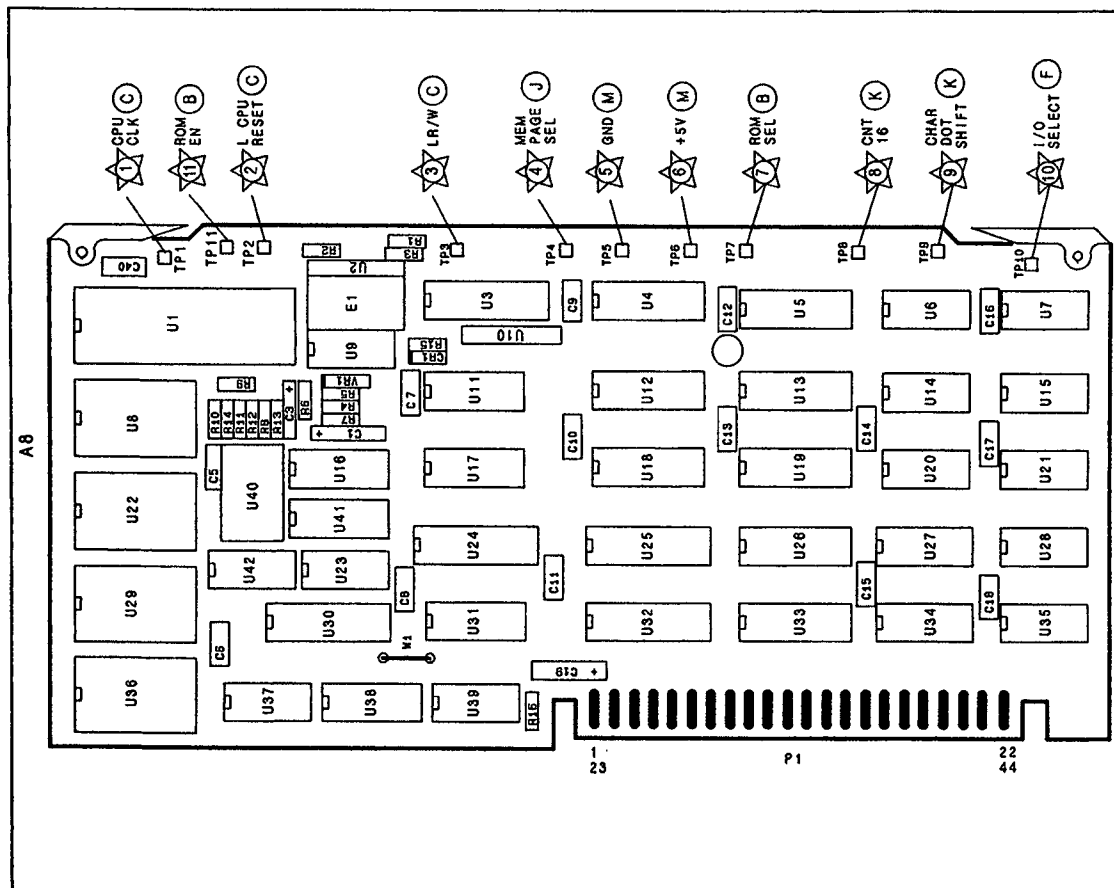
Figure 8-28. A8 Microprocessor Assembly, Component Locations
