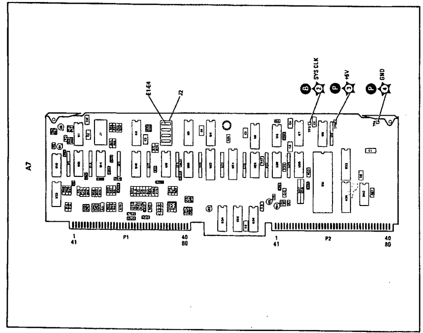
Figure 6-22. A7 Input/Output Assembly, Component Locations
