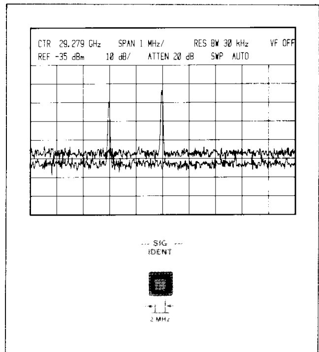
Figure 30. Signal Identifier
