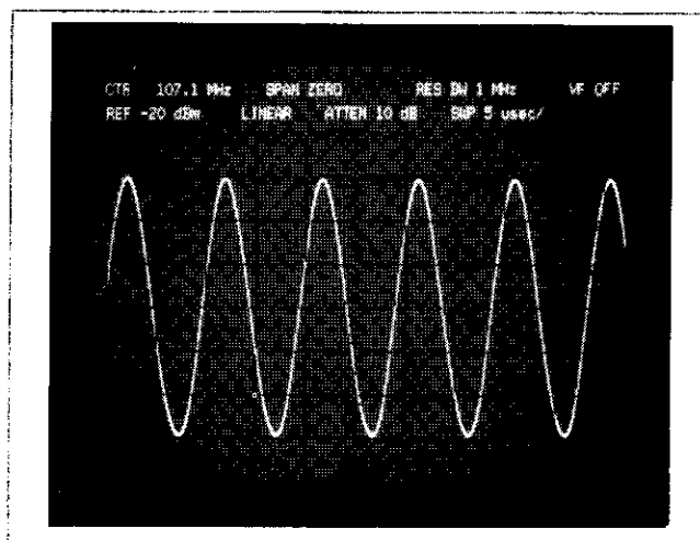
Figure 10. AM Carrier Demodulated in ZERO SPAN
