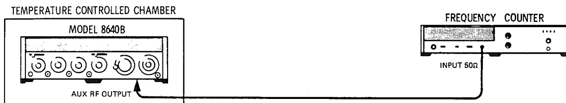
Figure 4-2. Frequency stability vs Temperature Test Setup
