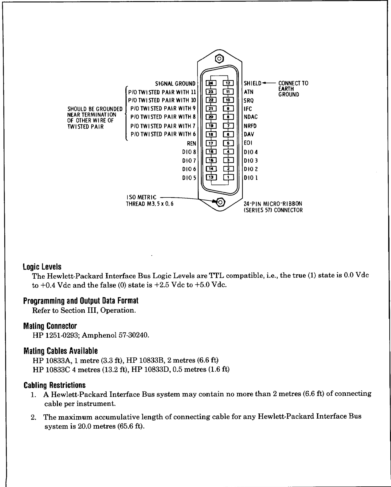
Figure 2-4. Hewlett-Packard Interface Bus Connections
