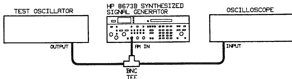
Figure 3-8. AM Functional Check Setup
