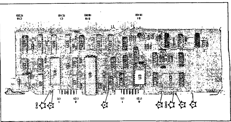
Figure 8-114. Microprocessor Assembly Component and Test Point Locations
