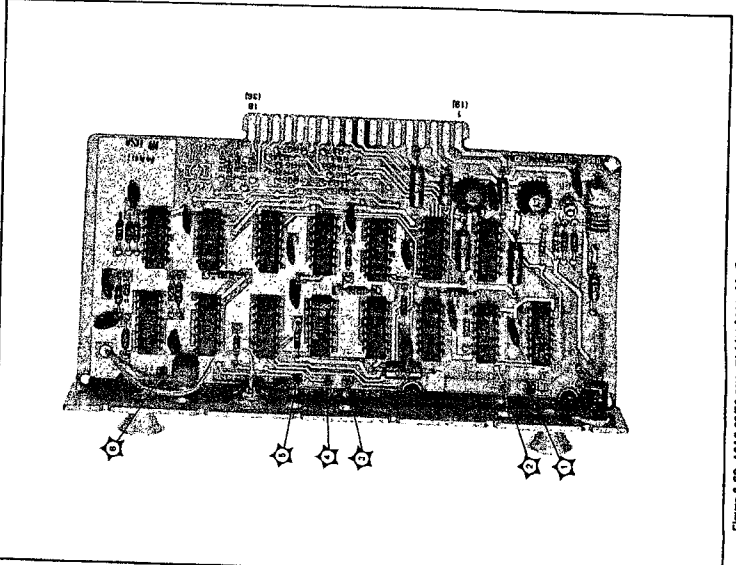
Figure 8-66. AZAS 2030 MHz Divider Assembly Component and Test Point Locations
