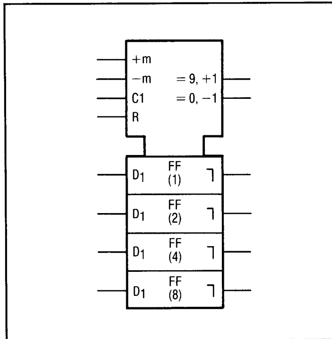
Figure 8-16. UP-DOWN Counter
