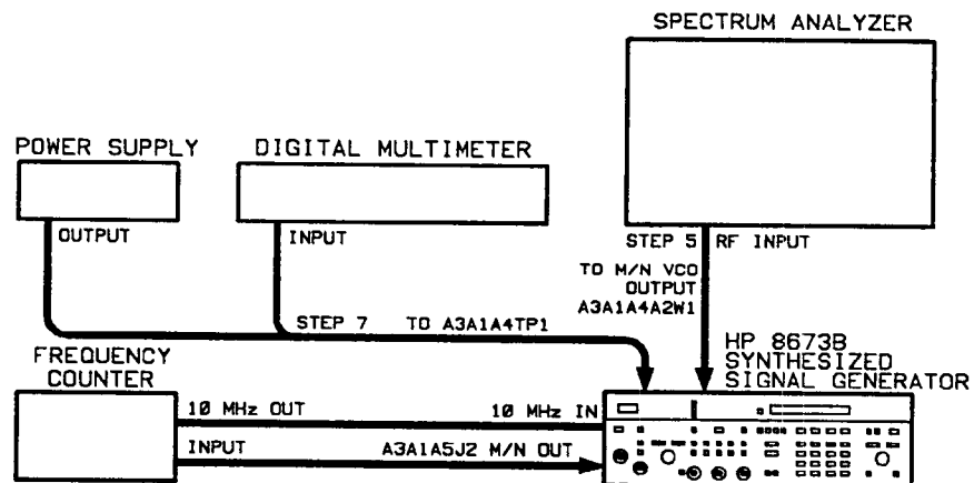
Figure 5-7. M/N Loop Adjustment Test Setup
