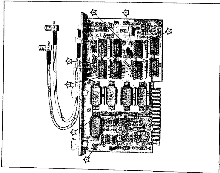
Figure 9-42. A31-1A3 M/N Phase Detector Assembly Component and Test Point Locations
