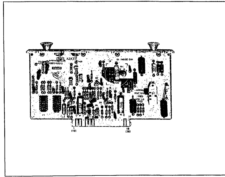
Figure 8-72. AZA3 VCO 160-240 MHz Assembly Component Locations
