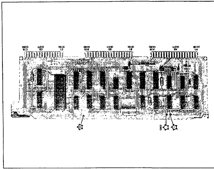
Figure 8-116. AZA8 Frequency Output - HP-IB Assembly Component and Test Point Locations
