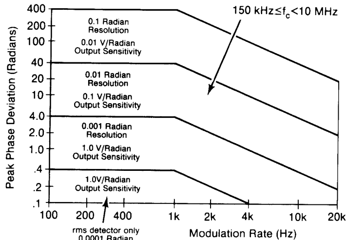
Phase Modulation Deviation and Maximum Resolution
