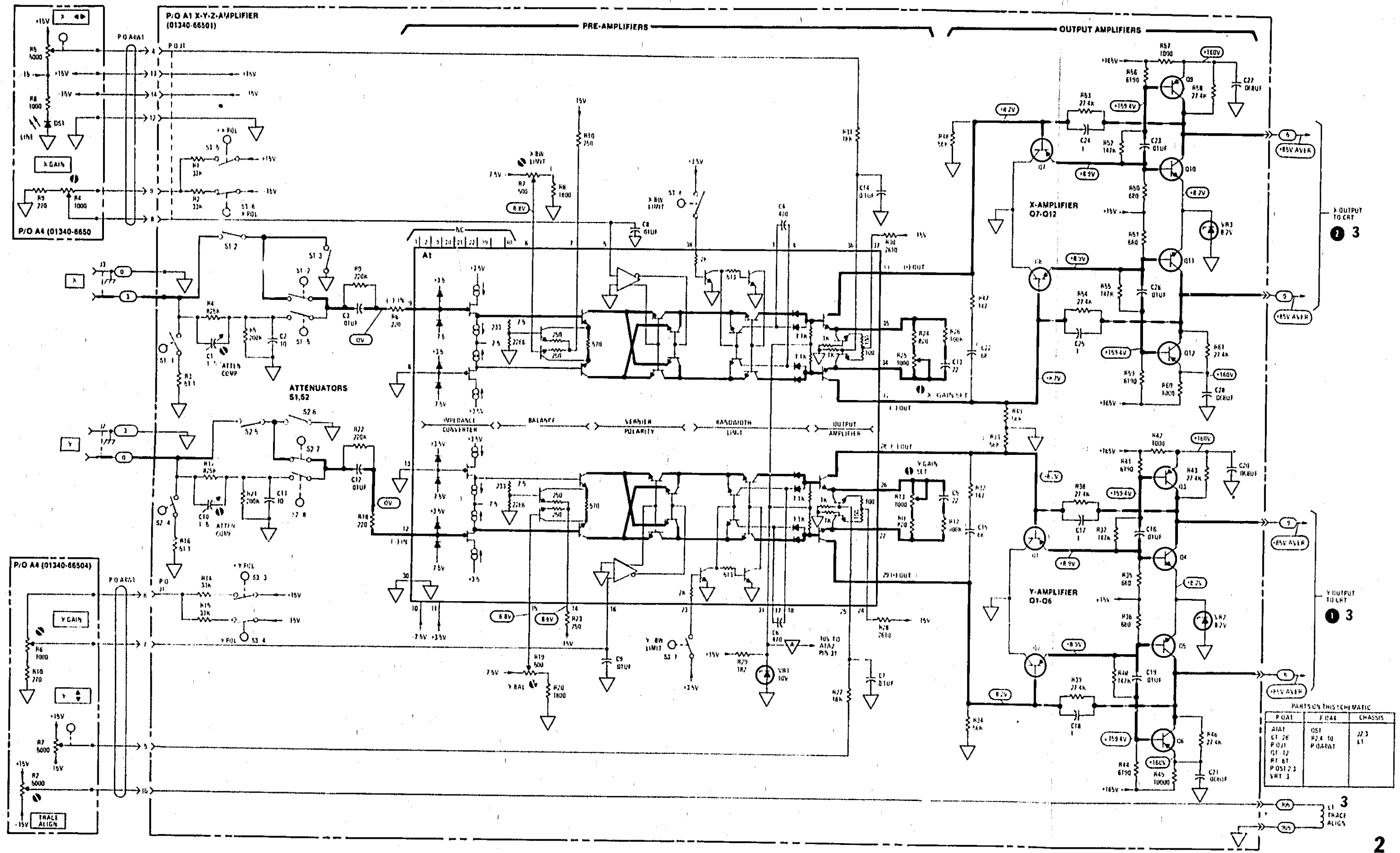
Figure 7-1 Service Sheet 2, X-Y Amplifiers 7-7
