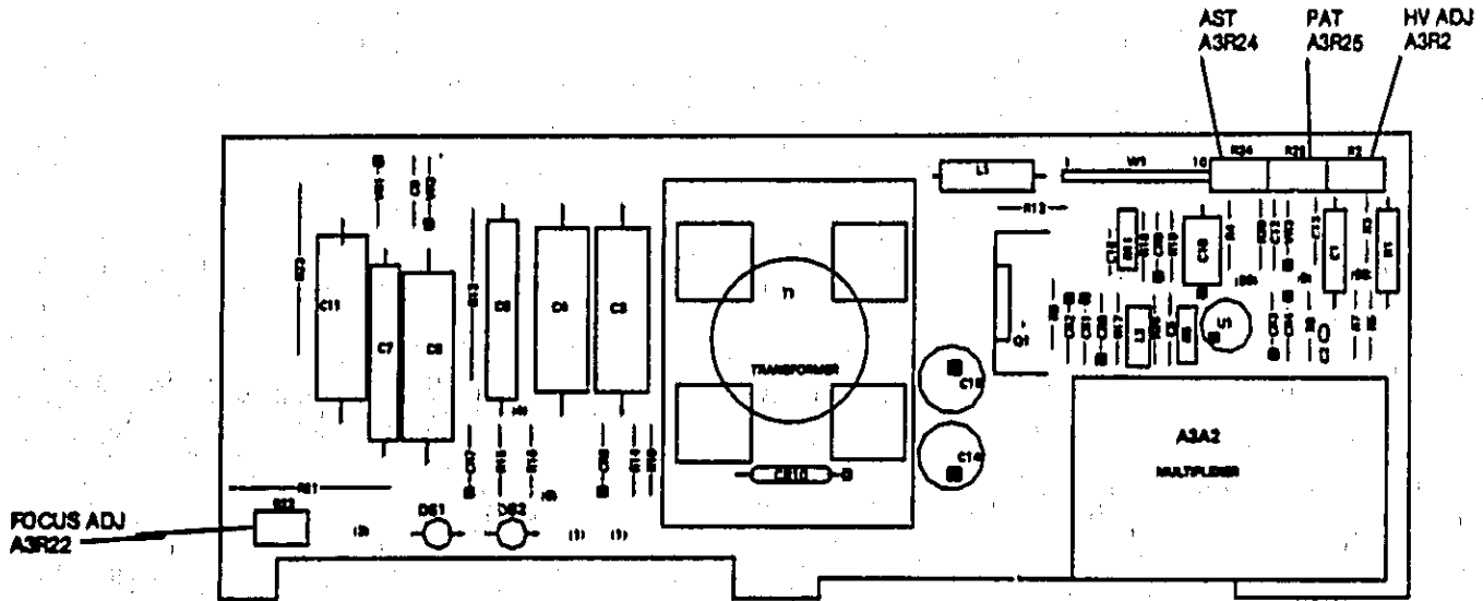
Figure 2. Adjustment Locations for HVPS, Assembly A3
