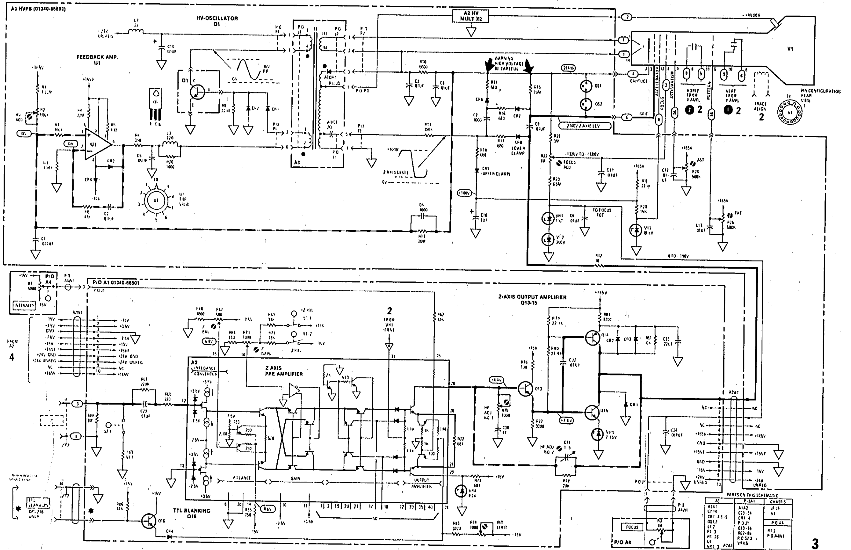
Figure 7-6 Service Sheet 3, HVPS and Z-Axis Amplifier 7-9
