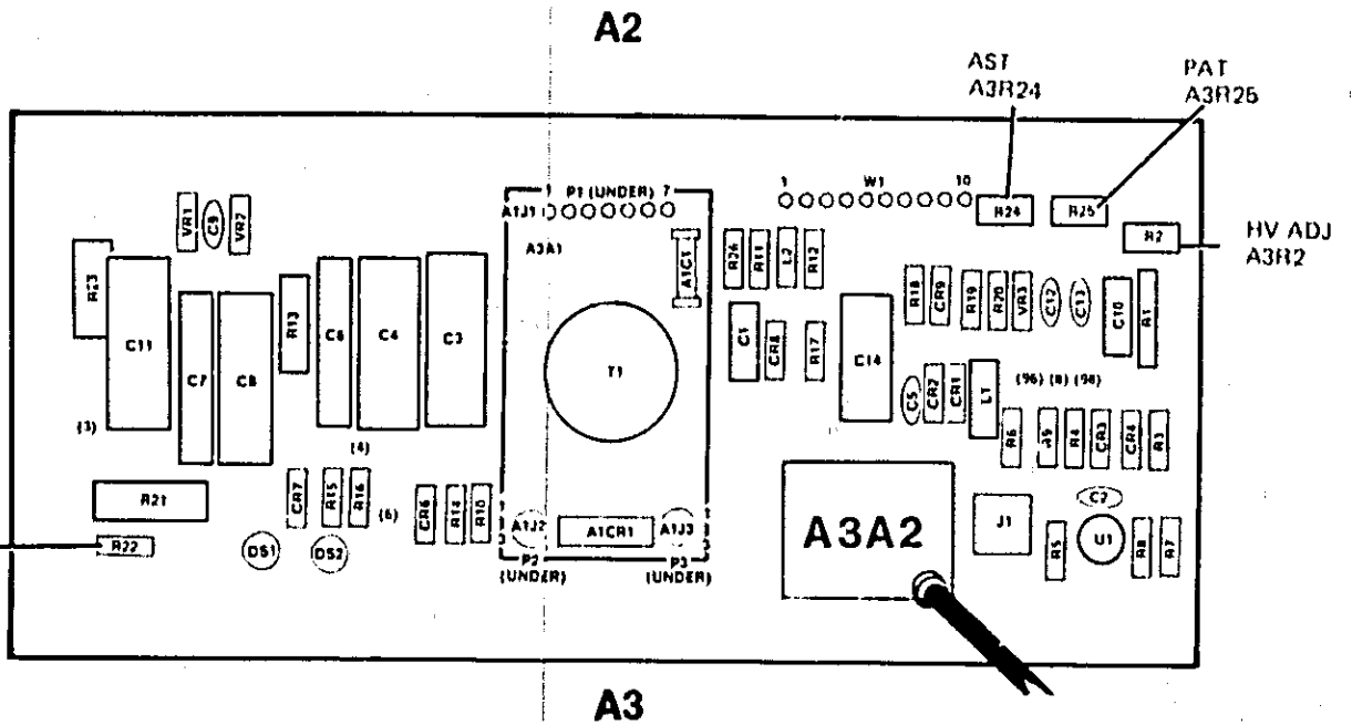
Figure 8-11. Service Sheet 6, Adjustment Locations 8-15
