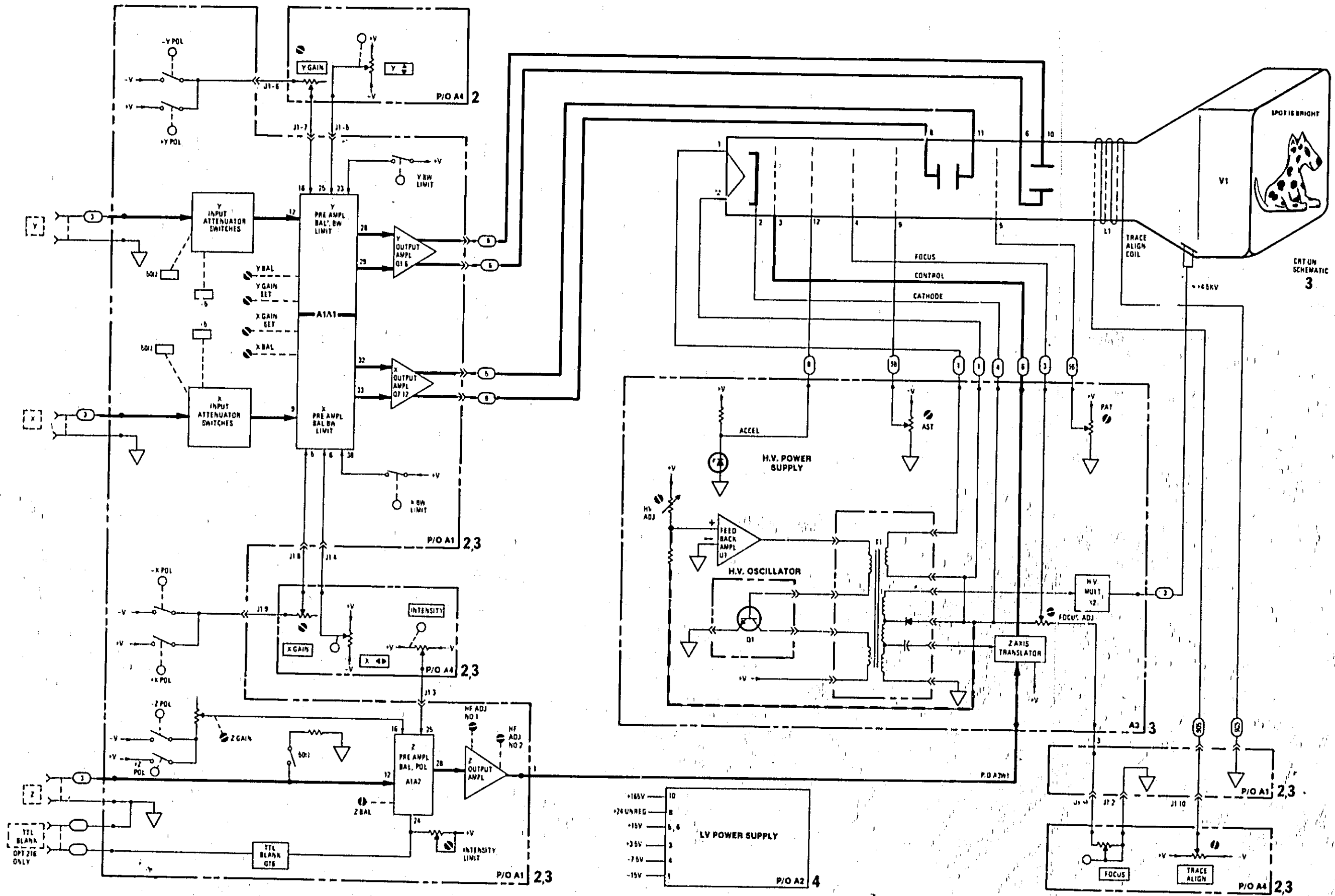
Figure 8-1. Service Sheet 1, Model 1340A Overall Bloch Diagram 8-5
