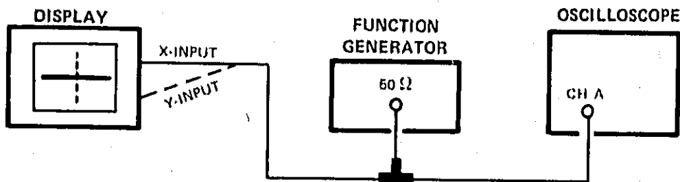
Figure 5-2. Gain Set Adjustment Test Setup
