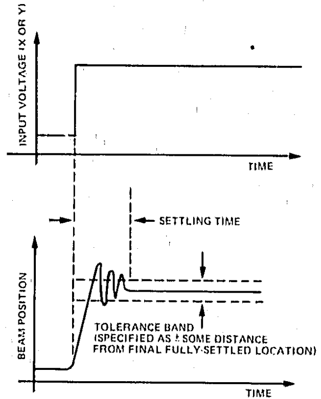
Figure 3-4. Settling Time
