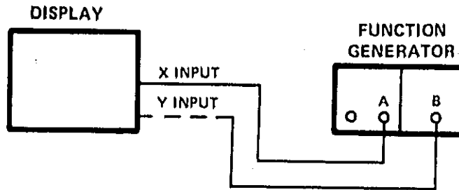
Figure 5-1. Pattern Adjustment Test Setup
