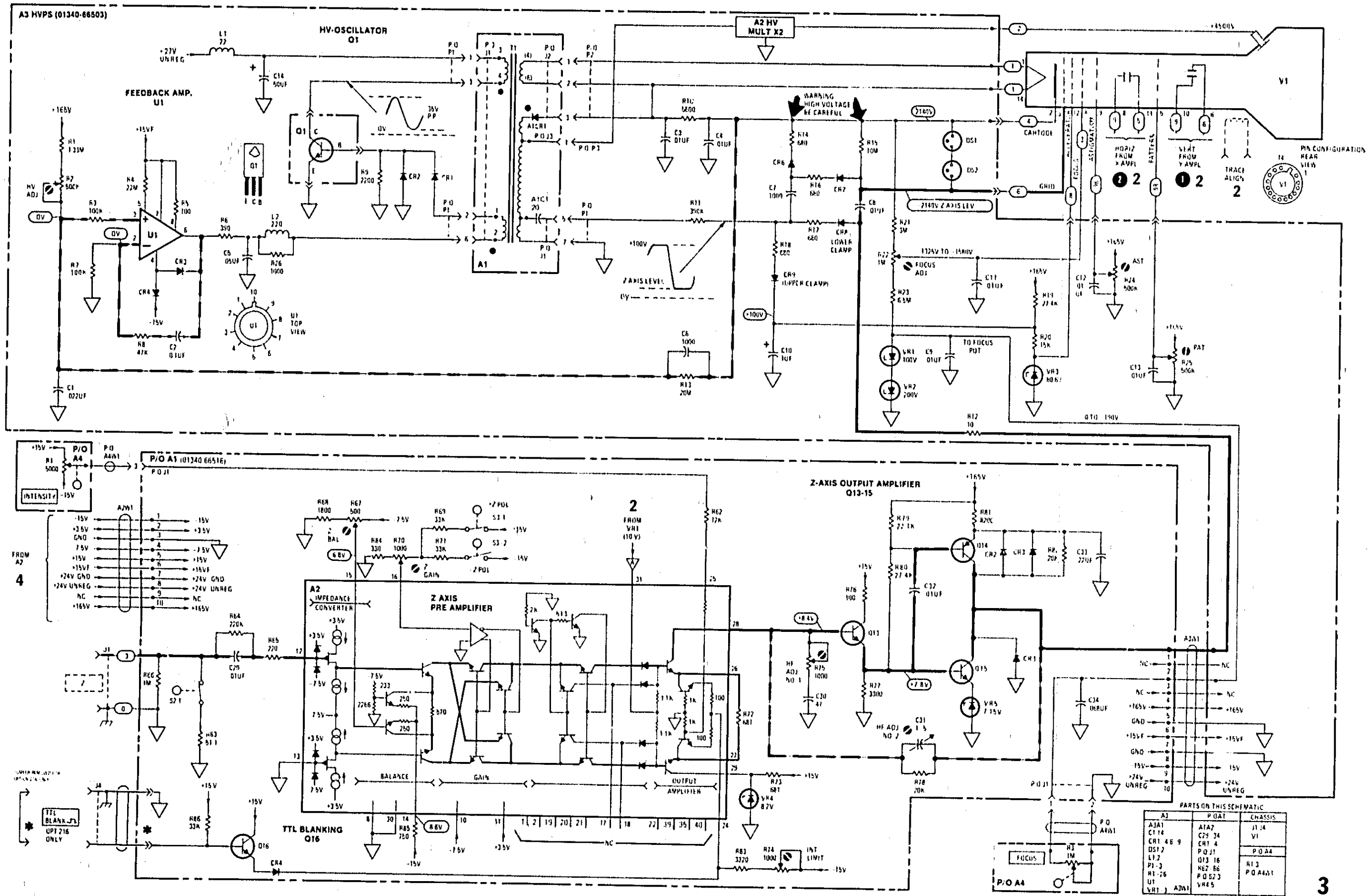
Figure 8-6 Service Sheet 3, HVPS and Z-Axis Amplifier 8-9
