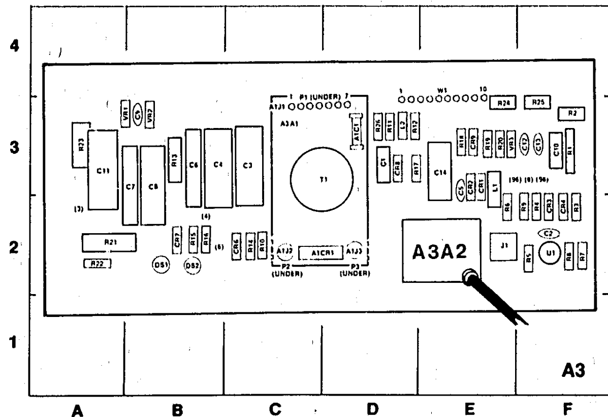
Figure 7-5. Component Identification, HVPS Assembly, A3
