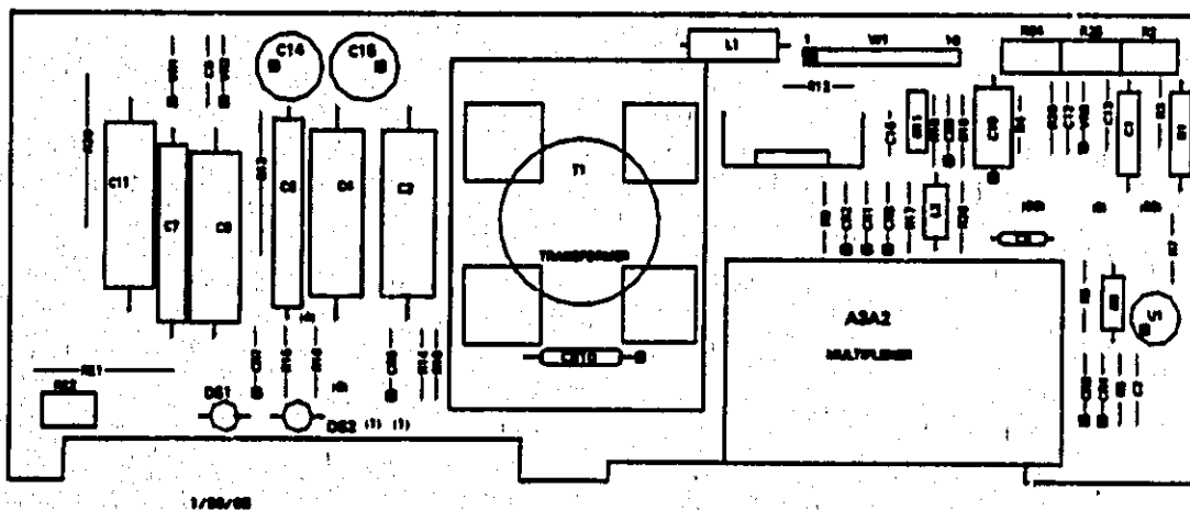
Figure 4. Component Identification for HVPS A3
