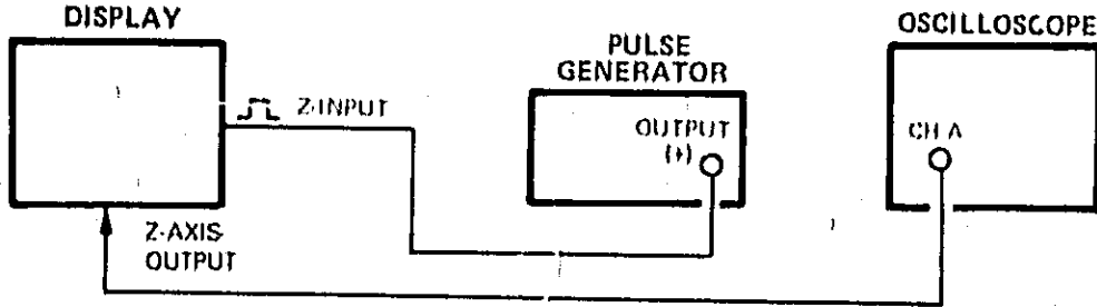
Figure 5-3. Z-amplifier Gain and High Frequency Adjustment Test Setup
