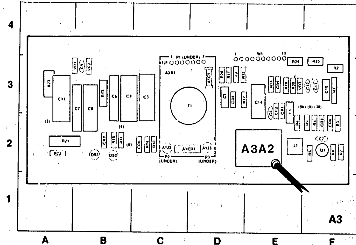
Figure 8-5. Component Identification, HVPS Assembly, A3
