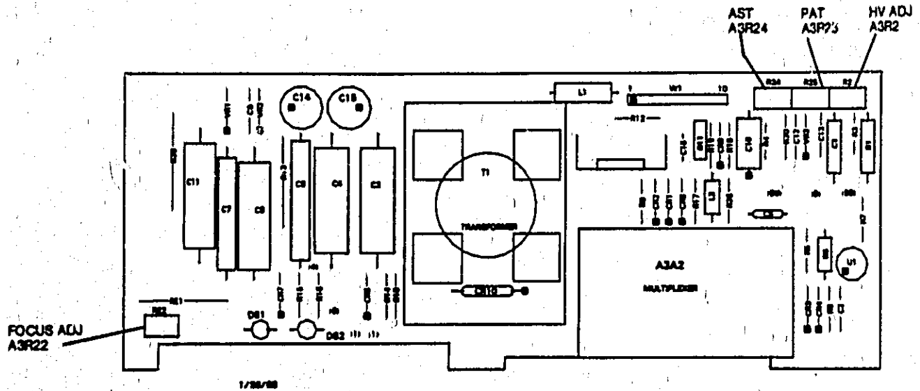
Figure 5. Adjustment Locations for HVPS Assembly A3
