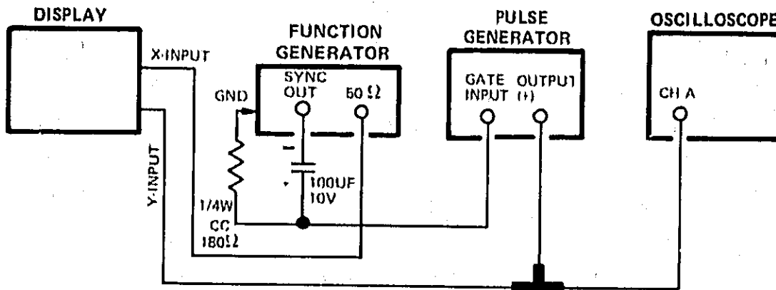
Figure 4-1. Dynamic Range Test Setup
