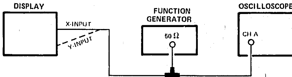
Figure 4-2. Bandwidth and Rise Time Test Setup
