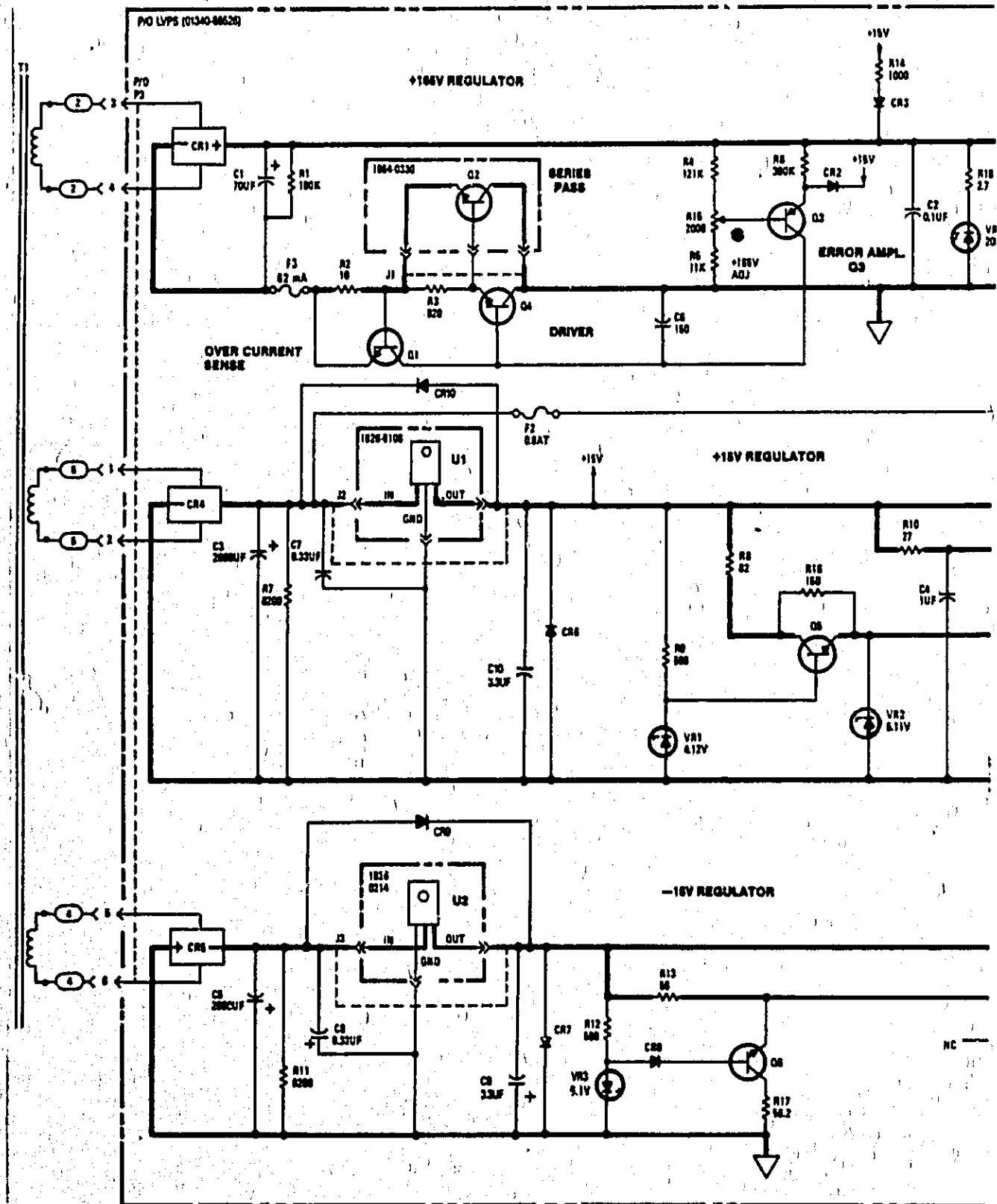
Figure 6. Component Additions to LVPS Assembly, A2.
