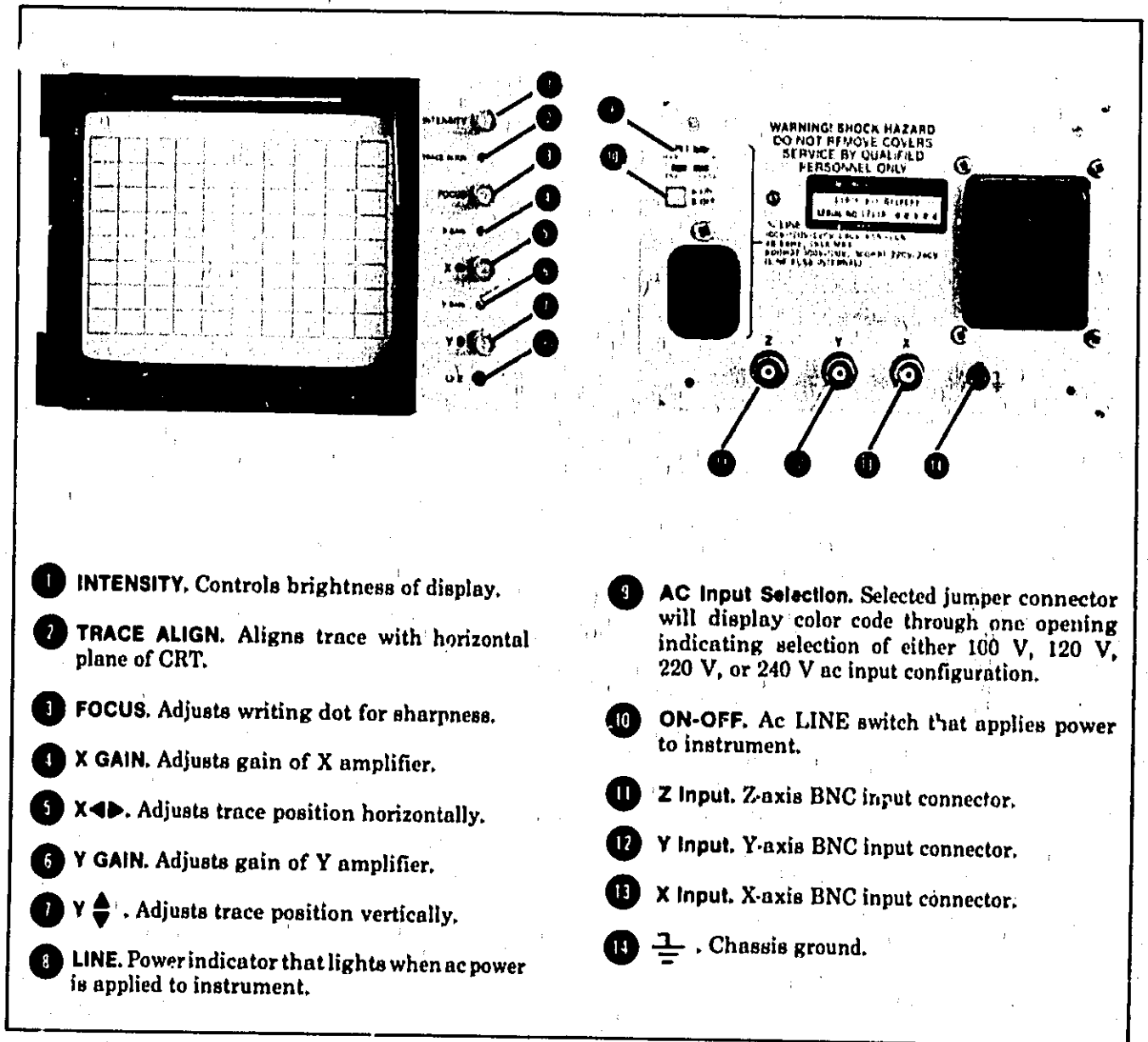
Figure 3-7. Controls and Connectors
