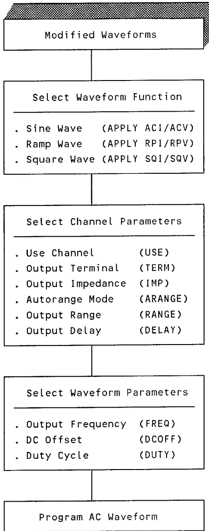
Figure 11-7. Modified AC Waveforms - Selection Steps
