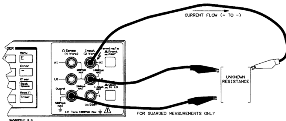
Figure 3-3 2-Wire ohms measurement connections
