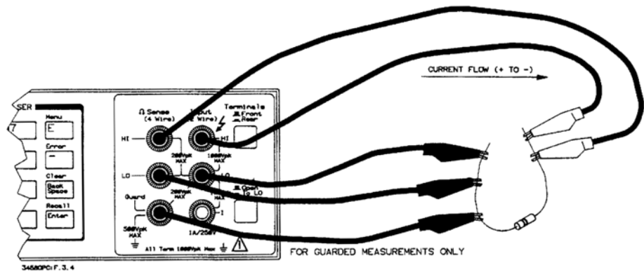
Figure 3-4 4-Wire ohms measurement connections
