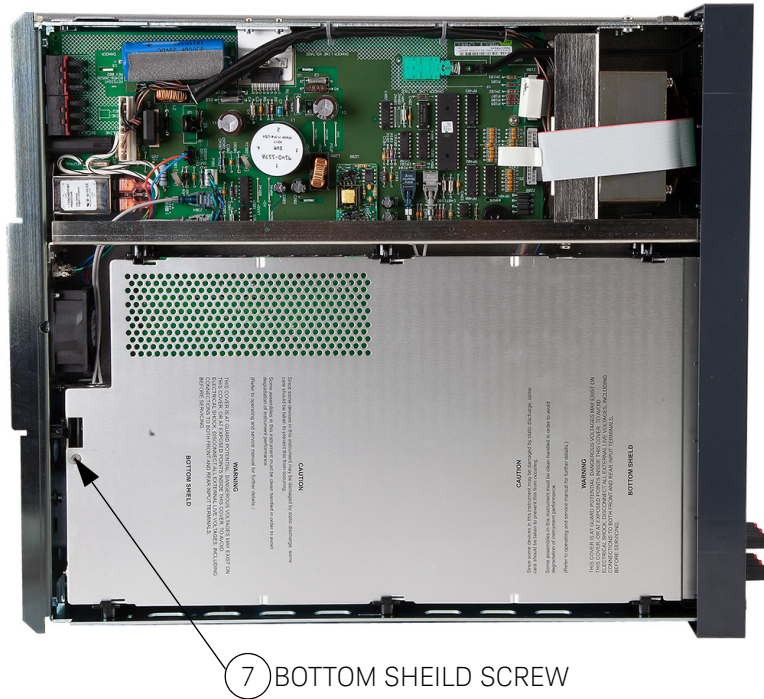
Figure C-5 3458A inside bottom view
