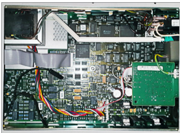
Figure 1. Picture of a Printed Circuit Assembly (PCA) under test.
