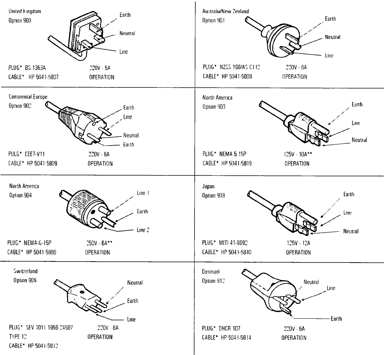
Figure 2-2. Power Cables
