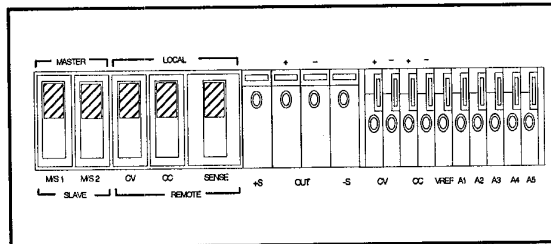
Figure 4. Switch Settings of Rear-Panel Control for Turn-On Checkout
