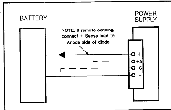
Figure 17. Recommended Protection Circuit for Battery Charging
