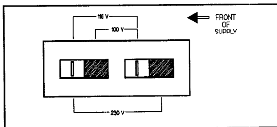
Figure 2. Line Voltage Selector (set for 115 Vac)
