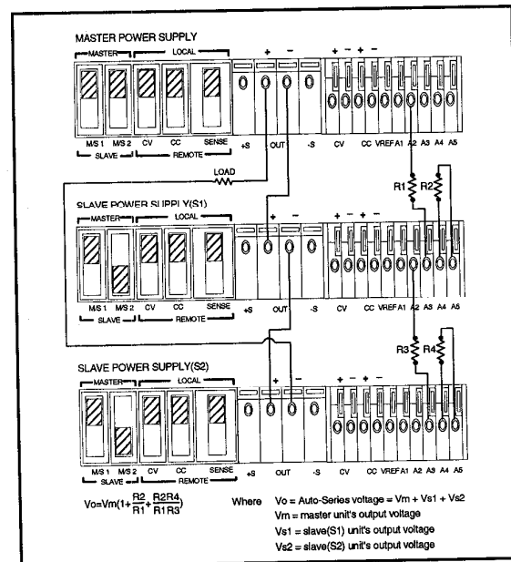
Figure 13. Auto-Series Operation of Three Supplies
