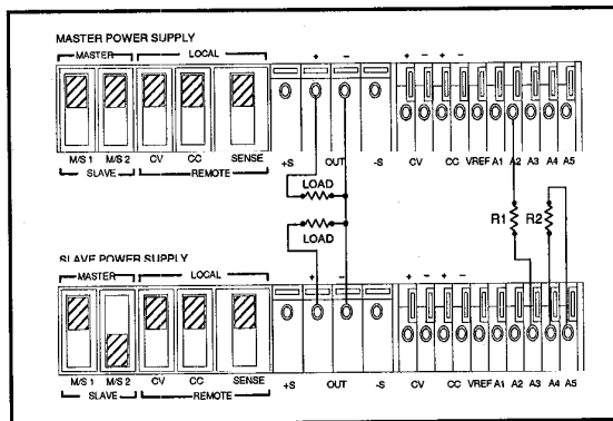
Figure 14. Auto-Tracking Operation of Two Supplies
