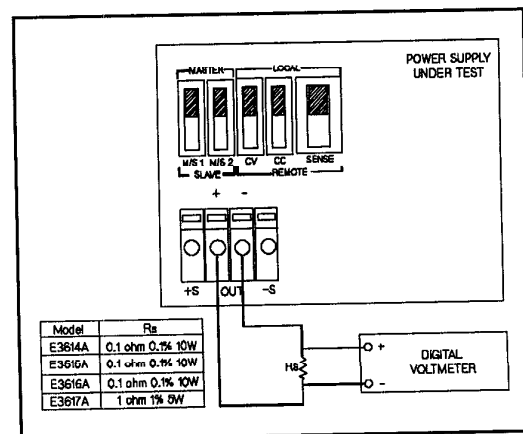
Figure A-9. Calibration Test Setup
