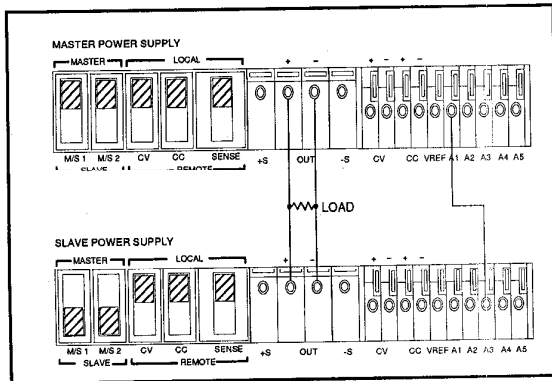
Figure 9. Auto-Parallel Operation of Two Supplies
