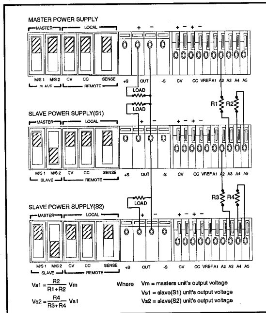
Figure 15. Auto-Tracking Operation of Three Supplies
