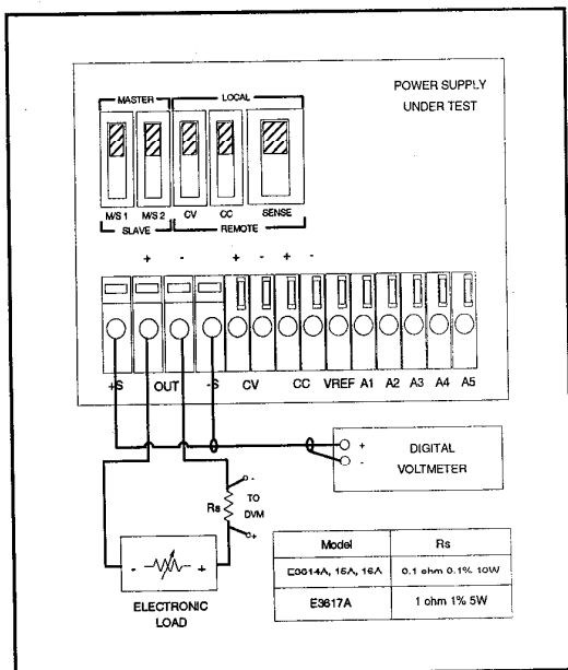
Figure A-4. Basic Test Setup
