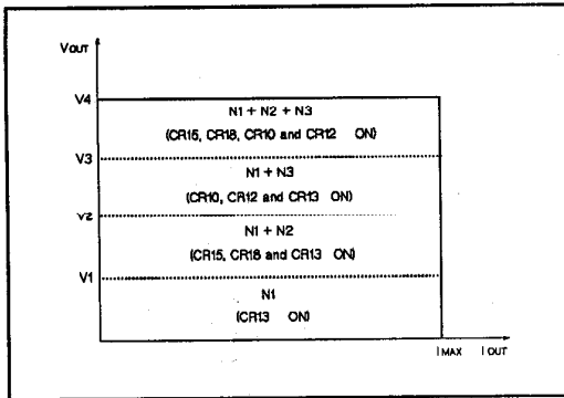
Figure A-2. Output Power Plot
