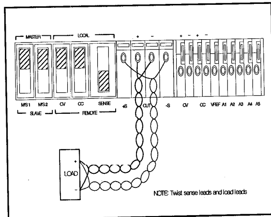
Figure 5. Remote Voltage Sensing
