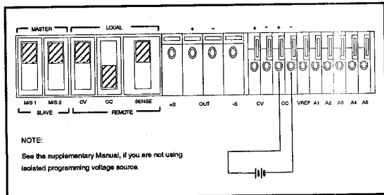
Figure 7. Remote Voltage Programming, Constant Current
