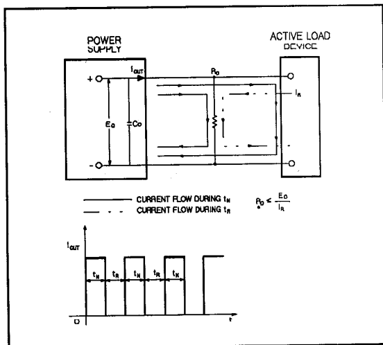
Figure 16. Reverse Current Loading Solution
