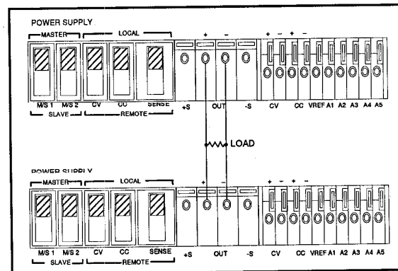
Figure 8. Normal Parallel Operation of Two Supplies
