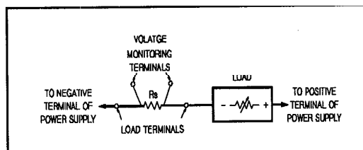
Figure A-3. Current Monitoring Resistor Connections
