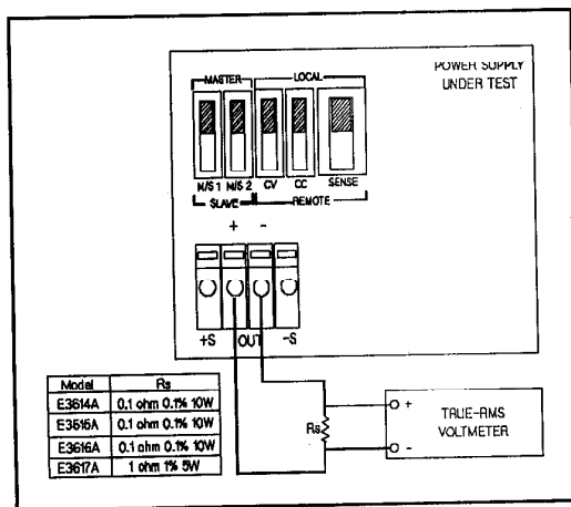
Figure A-8. CC PARD RMS Measurement Test Setup
