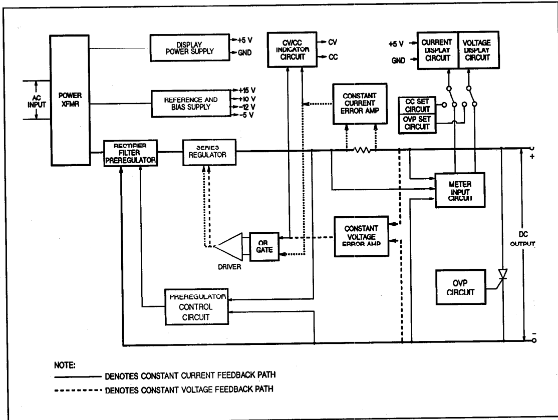
Figure A-1. Block Diagram
