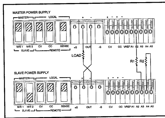
Figure 12. Auto-Series Operation of Two Supplies
