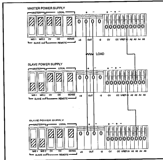
Figure 10. Auto-Parallel Operation of Three Supplies
