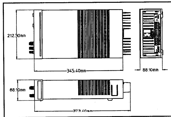
Figure 1. Outline Diagram
