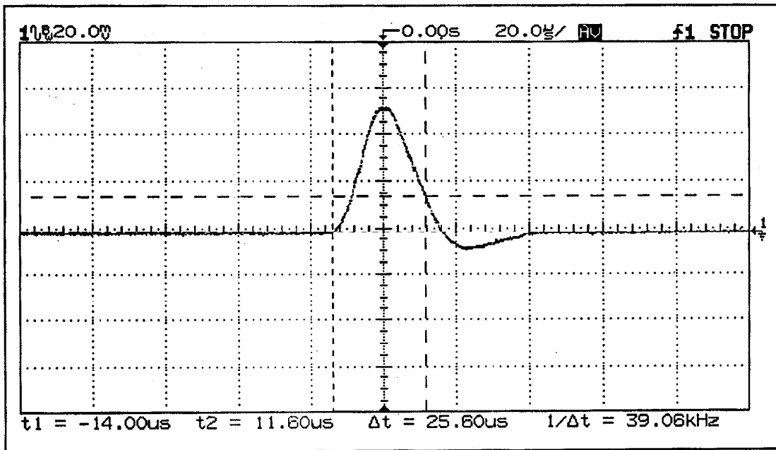
Figure A-5. Load Transient Response Time Waveform
