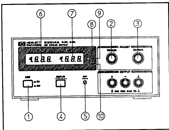
Figure 3. Front-Panel Controls and Indicators
