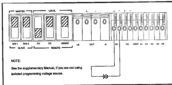
Figure 6. Remote Voltage Programming, Constant Voltage
