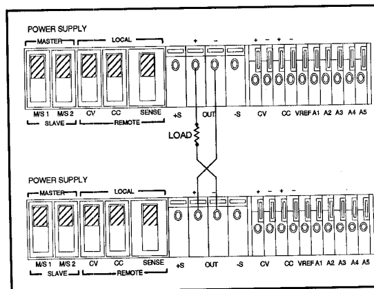
Figure 11. Normal Series Operation of Two Supplies
