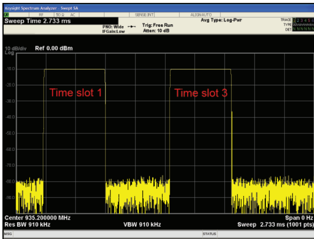
Figure 2-36. A zero span (time domain) view of the GSM signal with only time slots 1 and 3 "on".
