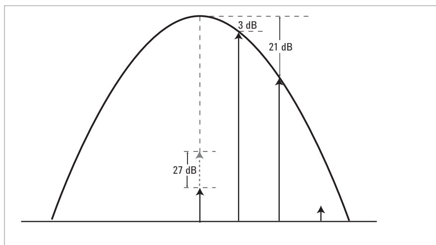
Figure 7-13. Improved third-order intermodulation distortion; test tone separation is significant relative to preselector bandwidth
