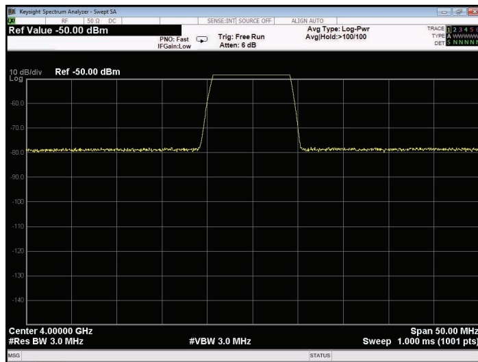
Figure 6-8. Display range and measurement range on the PXA spectrum analyzer
