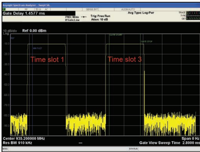
Figure 2-38. Time gating is used to look at the spectrum of the GSM time slot 3.
