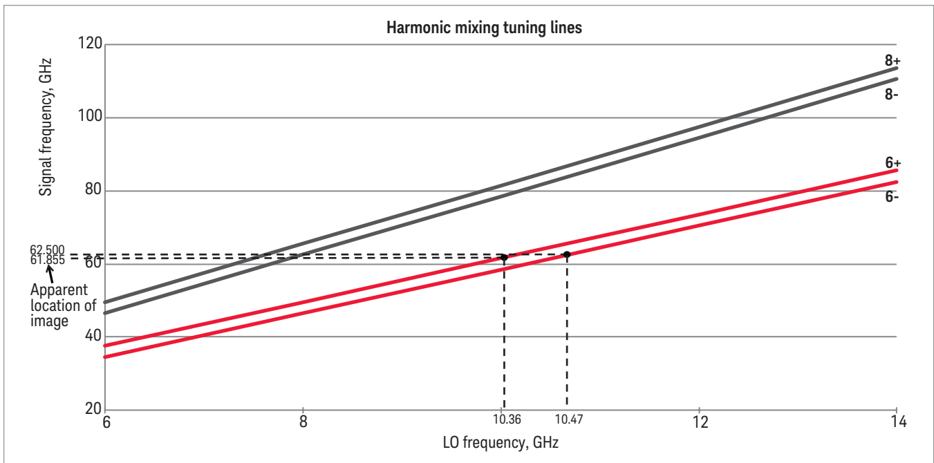
Figure 7-16 Harmonic tuning lines for the X-Series analyzers using the M1970 Series mixers
