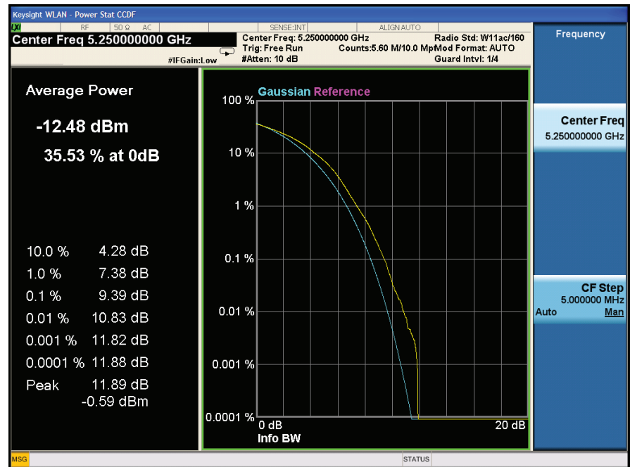
Figure 8-1. CCDF measurement
