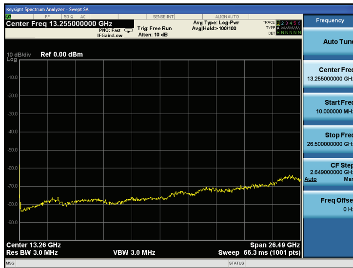
Figure 7-10. Rise in noise floor indicates changes in sensitivity with changes in LO harmonic used
