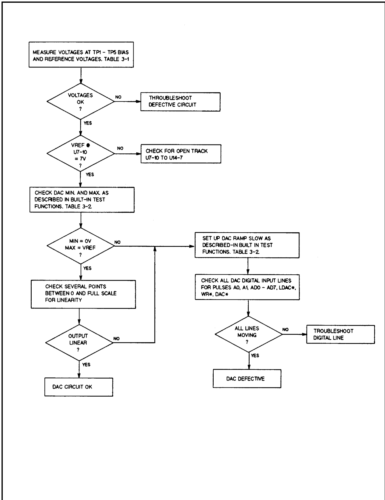
Figure 3-11. Troubleshooting DAC Circuit
