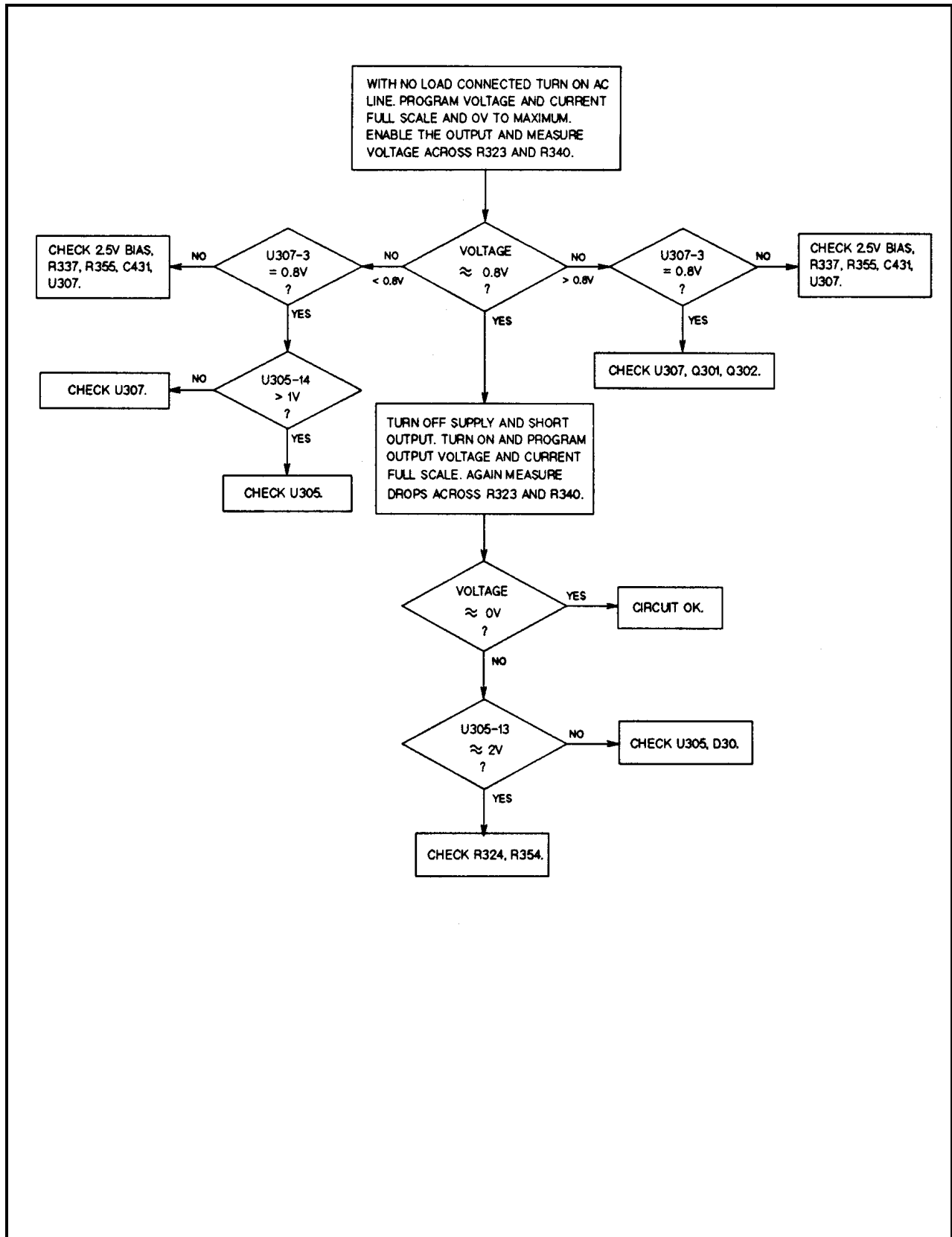
Figure 3-10. Troubleshooting Downprogrammer
