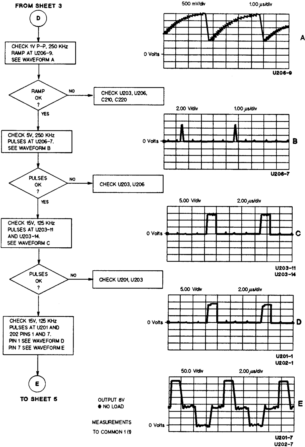
Figure 3-5. Troubleshooting No Output (Sheet 4 of 5)
