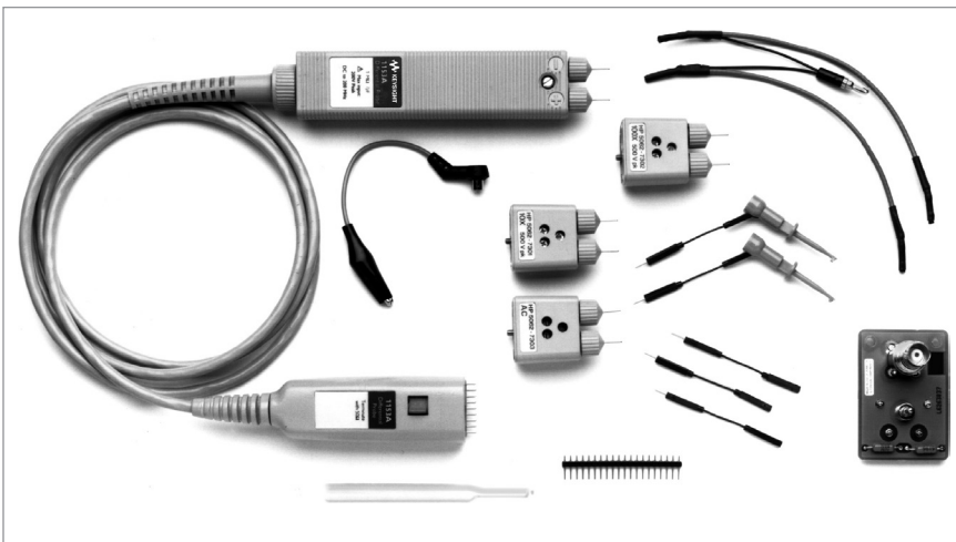
Keysight 1153A 1:1 FET differential probe with 200 MHz bandwidth.
