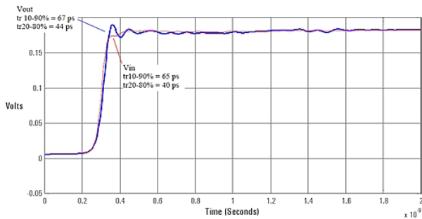
Graph of Vin and Vout of 1169A and N5381A solder-in head with a 25 Ω 58 psec step generator
