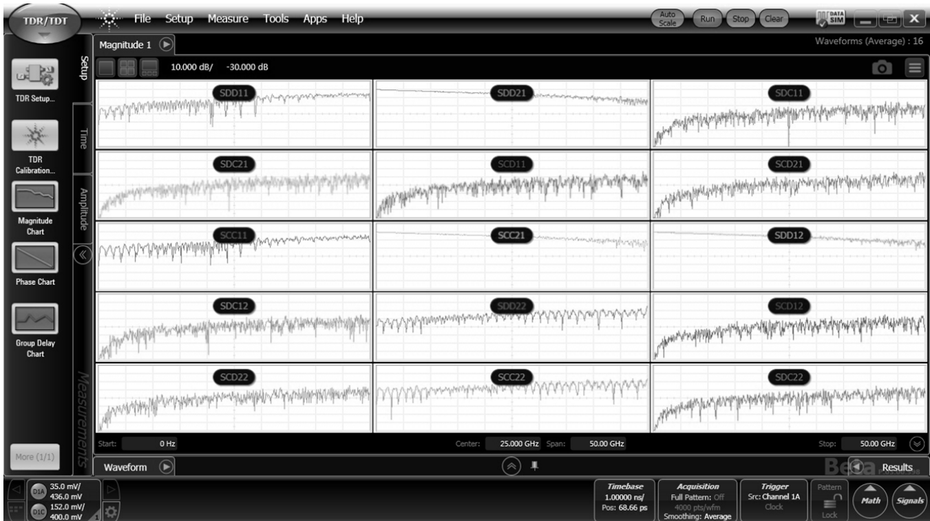
Figure 22: Live on-board frequency domain results on the 86100 TDR showing all 32 S-Parameters for a 2 port differential DUT
