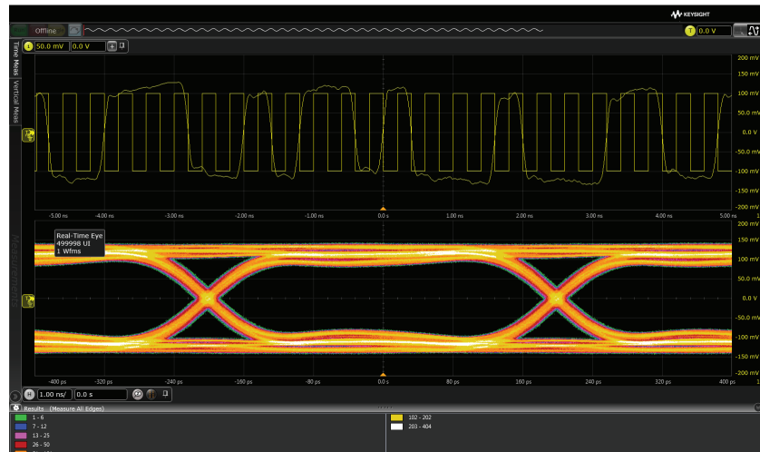
Figure 11. The display shows a data signal superimposed with a recovered clock.
