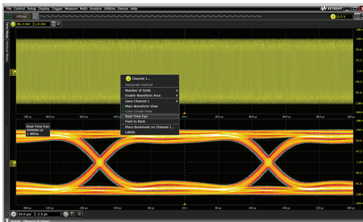
Figure 7. Real-time eyes can be created by a single click of the mouse.
