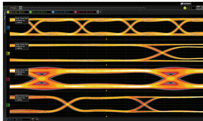
Figure 12. SDA lets you look at many real-time eyes at once.
