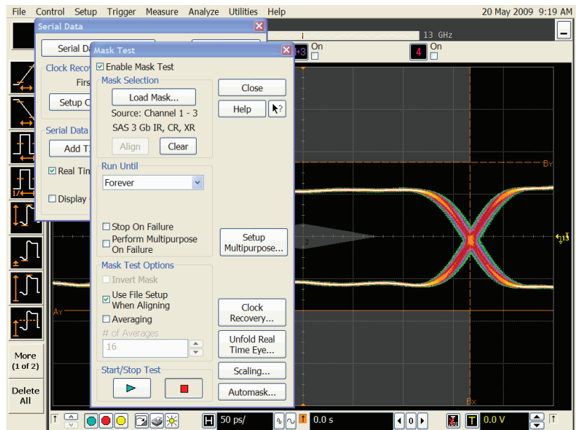
Figure 3. An example of leading a mask through SDA software.
