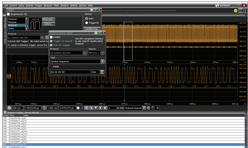
Figure 8. Configuring a serial data trigger in the 8b/10b protocol
