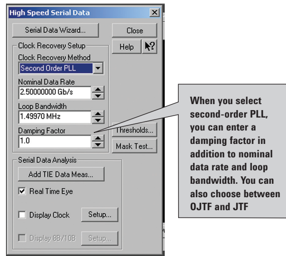
Figure 10. Second-order PLL selections.
