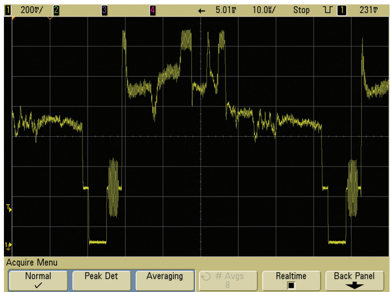
Figure 4. Zoomed-in display of a single line of video using a Keysight InfiniiVision Series scope
