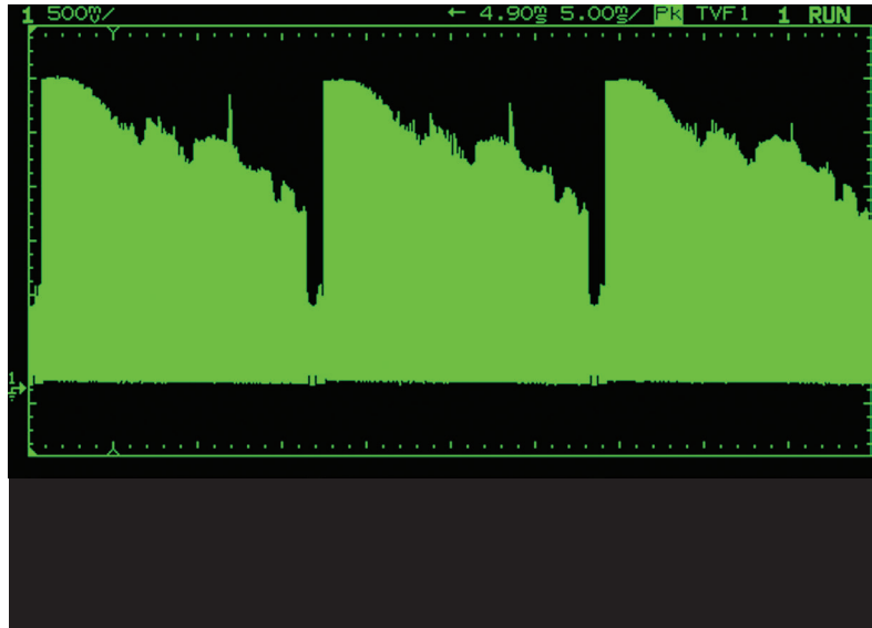
Figure 2. Full frame of composite video displayed on an older digital oscilloscope without intensity gradation capability
