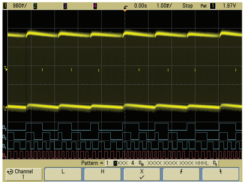
Figure 6. A Keysight InfiniiVision Series scope reveals "bright spots" buried within each digital burst
