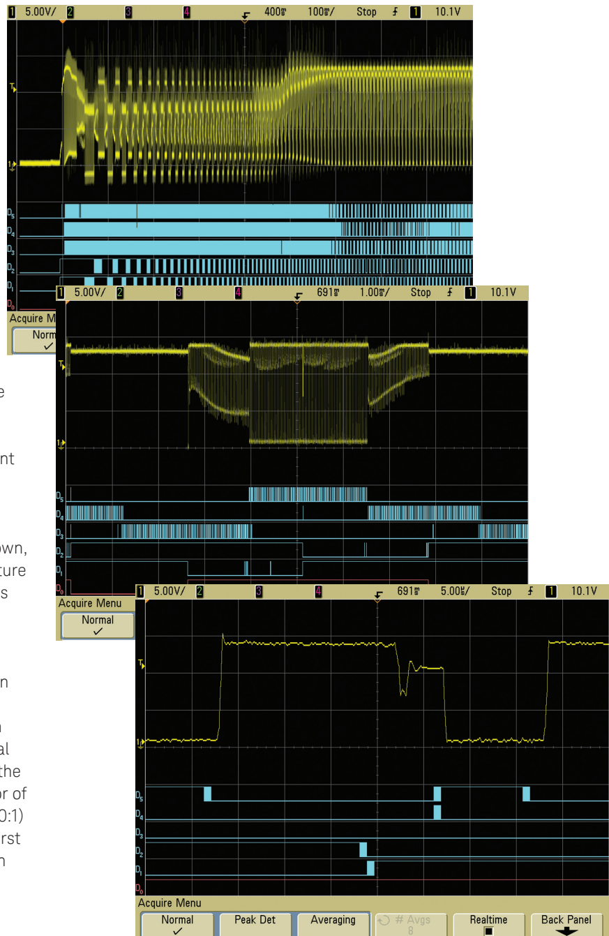
Figure 5. Motor drive signal start-up sequence with digital control signal triggering and various levels of zoom to reveal a "runt" pulse using a Keysight InfiniiVision Series MSO
