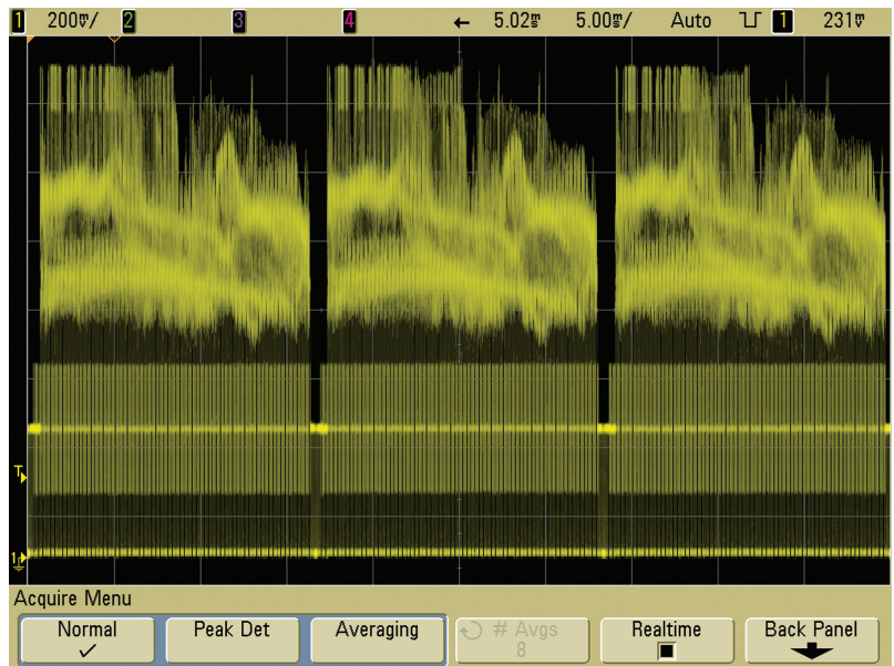
Figure 3. Full frame of composite video displayed on a Keysight InfiniiVision Series scope
