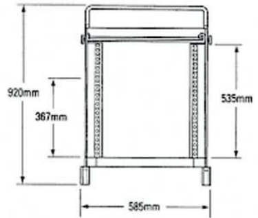
Figure 12. Keysight 1181BZ testmobile cart dimensions.
