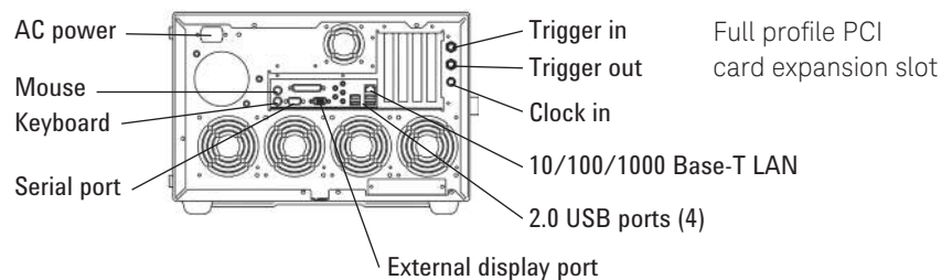
Figure 9. 16800 Series back panel.
