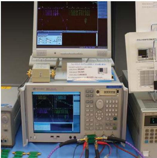
DC-biased measurement setup
