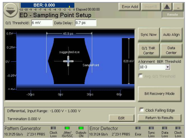
Figure 11. Auto alignment (center) simplifies correct sampling
