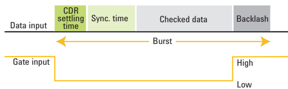
Figure 28. Burst mode allows recirculation loop testing
