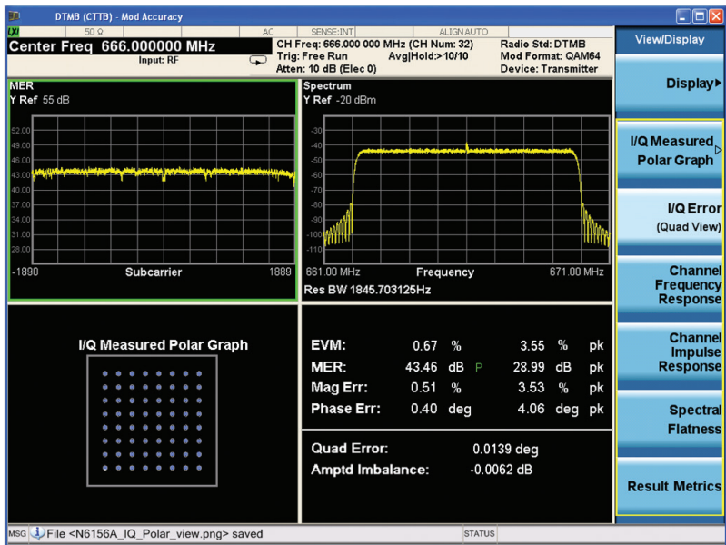
Figure 3. DTMB (CTTB) IQ quad view
