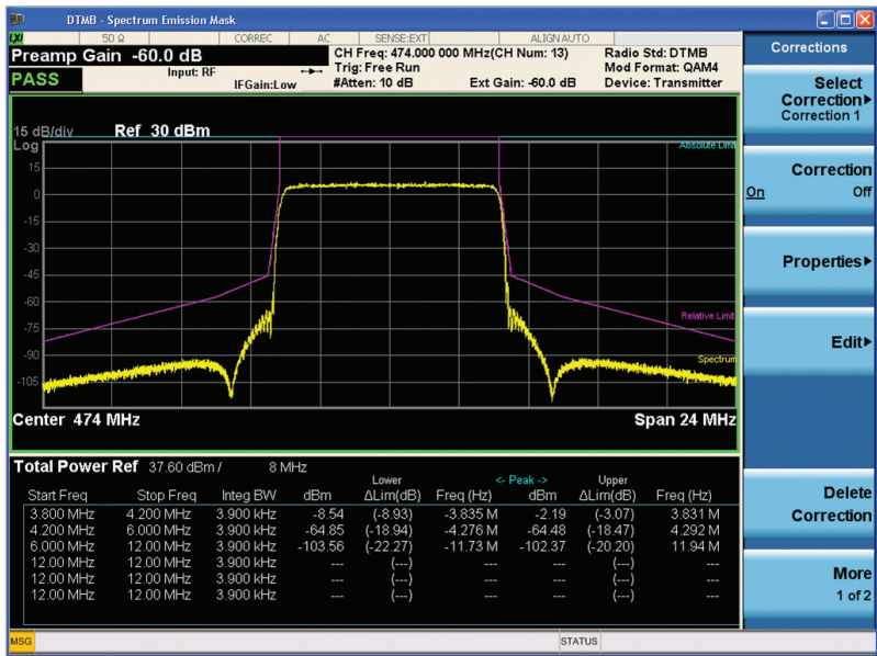
Figure 6. DTMB (CTTB) spectrum emission mask
