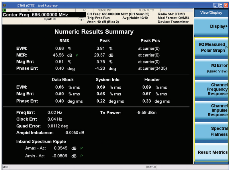
Figure 4. DTMB (CTTB) result metrics view
