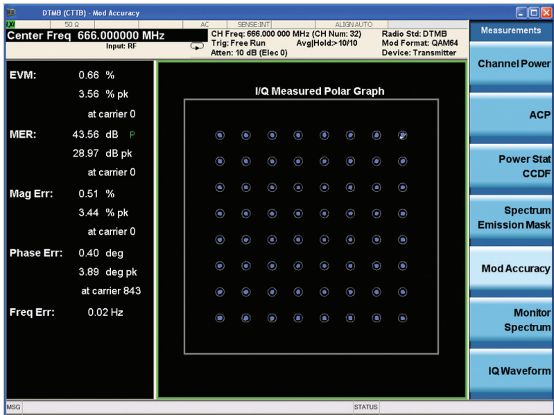
Figure 2. DTMB (CTTB) constellation and MER results
