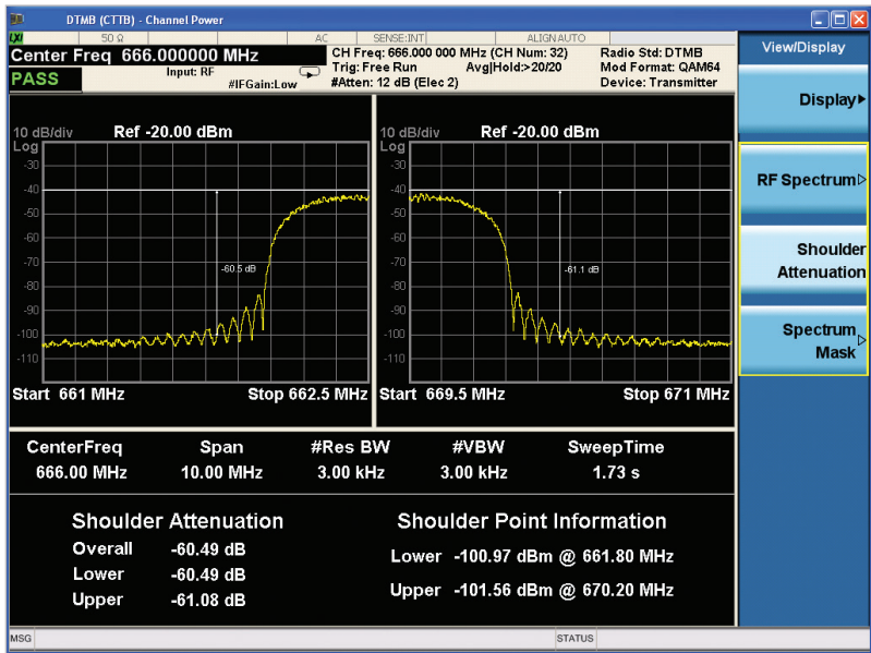
Figure 5. DTMB (CTTB) shoulder attenuation
