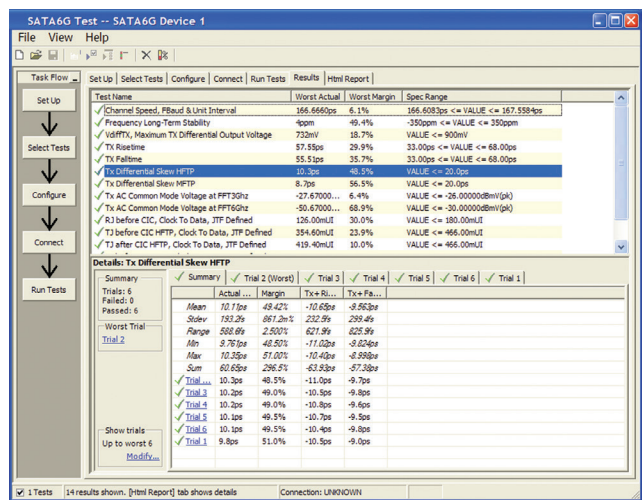
Figure 6. The Keysight SATA report can be customized to show only the user-selectable repetitive run data, and filtered to show only the relevant data and statistics desired in the final report.
