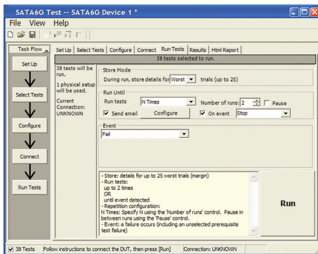
Figure 5. The Keysight SATA software allows for user-selectable repetitive test execution.
