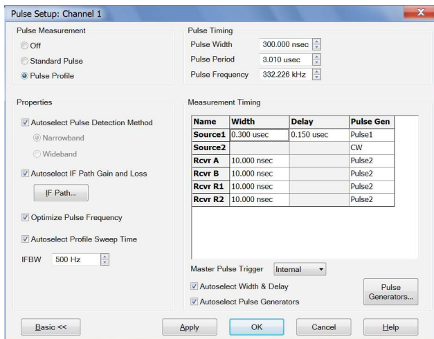
Pulsed-RF measurement application automatically optimizes internal hardware configuration for specified pulse conditions to dramatically simplify test setups. Alternately, users can choose to manually set up the hardware for unique test requirements.
