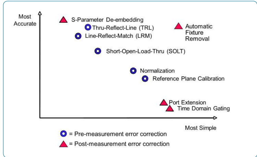
A relative comparison of various fixture error-correction methods
