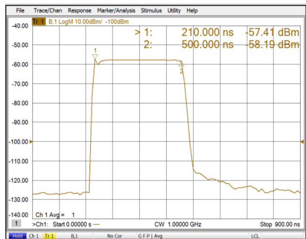
Pulse profile measurement using narrowband detection technique allows 30 measurement points within 300 ns pulse, with 10 ns timing resolution.
