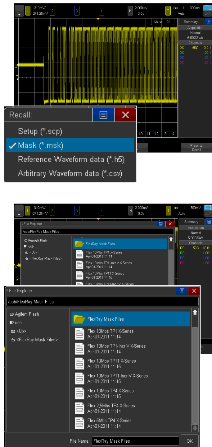
Figure 5. Recalling a FlexRay eye-diagram mask test file.
