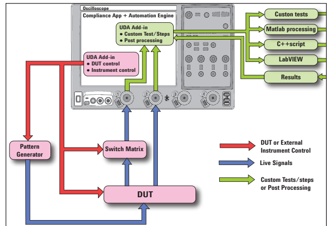
Figure 16. Combine the power of built-in automation and extensibility to transform your application into a complete test suite executive.
