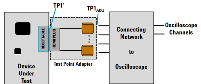
Figure 3: Test point adapter breaking out signals to the oscilloscope through cable network.
