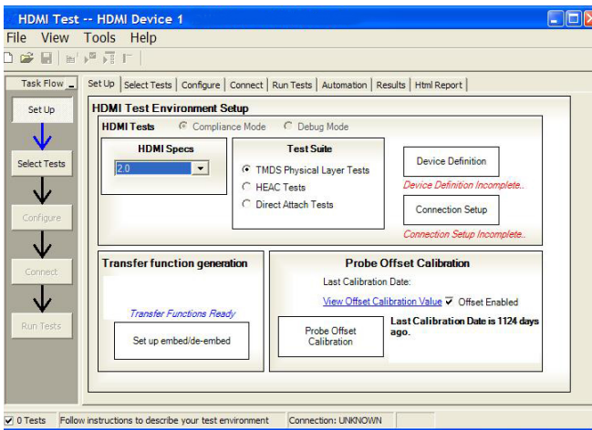
Figure 5: Entry screen for HDMI software.
