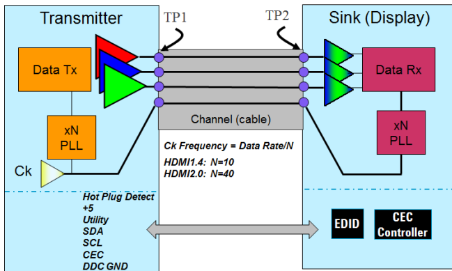
Figure 1: HDMI Interface.
