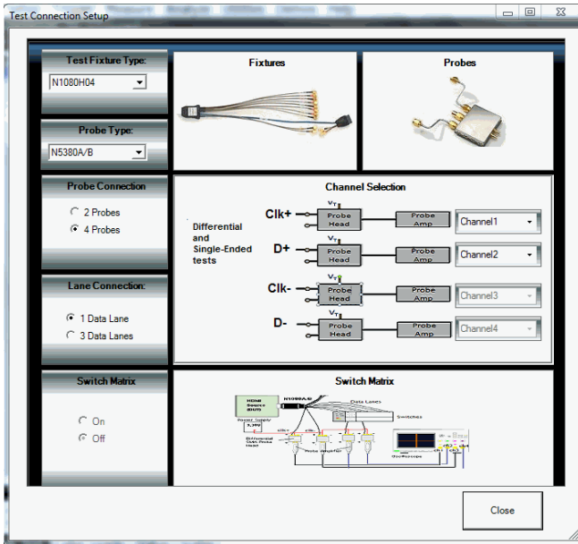
Figure 7: Test connection setup screen.
