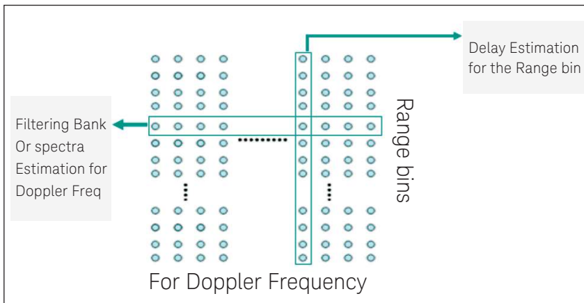
Figure 6-8. Signal Processing in MTD
