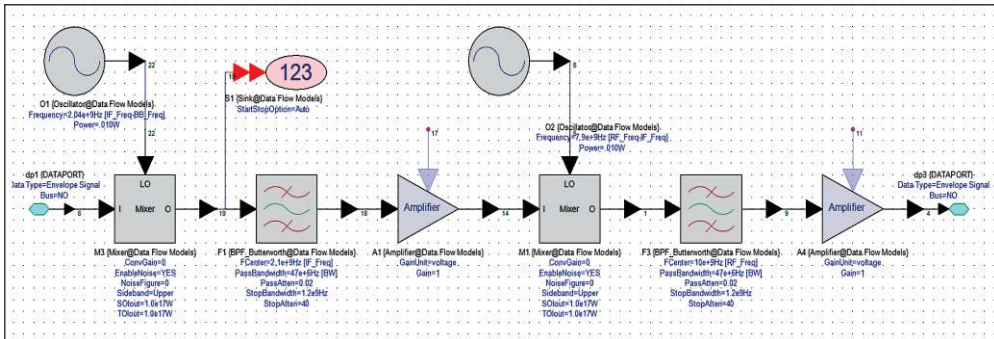
Figure 6-2. RF transmitter
