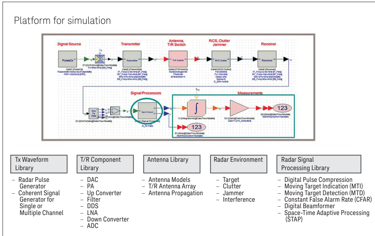
Figure 3-1. SystemVue as a platform for simulation
