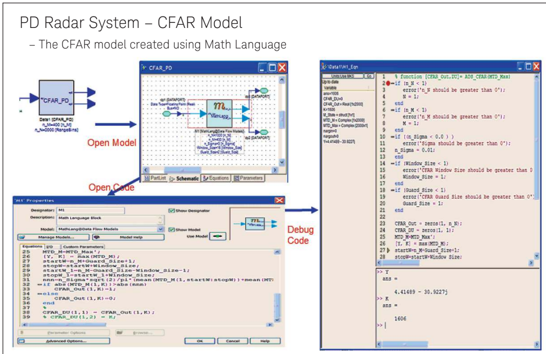
Figure 6-10. Cell averaging CFAR processor
