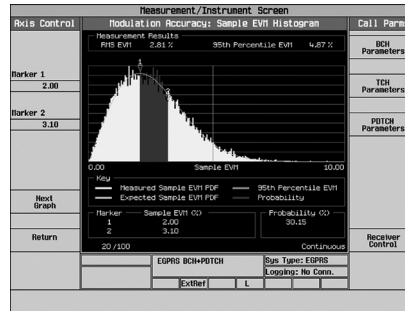
Figure 2: EGPRS modulation accuracy measurement includes a graphical sample EVM histogram to observe your device's statistical EGPRS performance.
