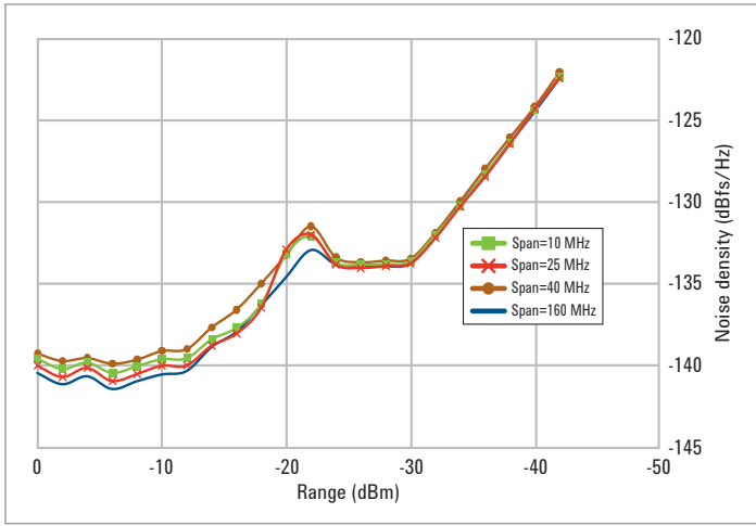
PXA noise density (nominal, 1.8GHz)
