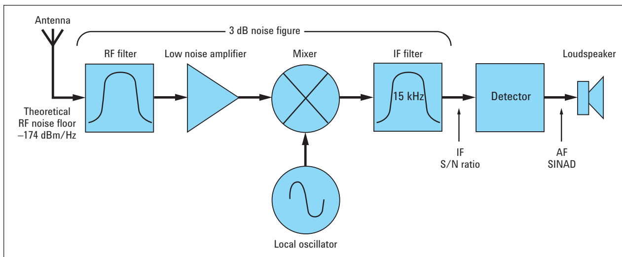
Figure 3. Basic receiver block diagram
