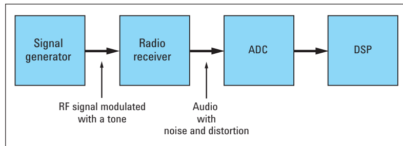
Figure 2. Block diagram showing the sampling of an audio signal and computation in DSP
