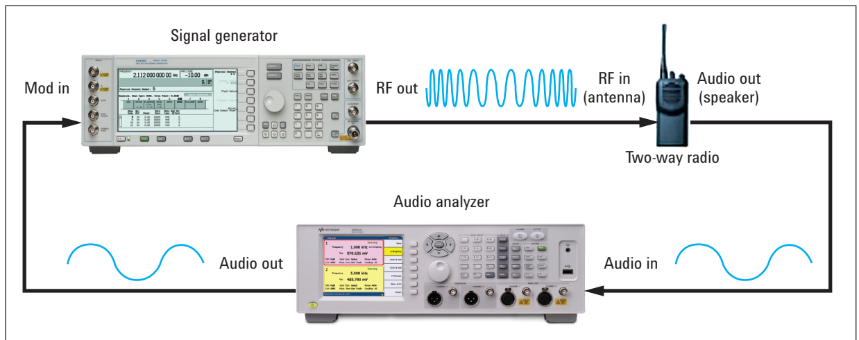
Figure 4. General SINAD measurement setup
