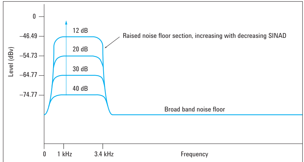
Figure 11. SINAD increases as the shaped noise floor area decreases in amplitude
