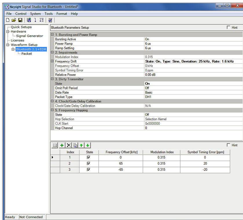
Figure 4. Configure impairments such as dirty transmitter and frequency drift for Bluetooth EDR transceiver test.
