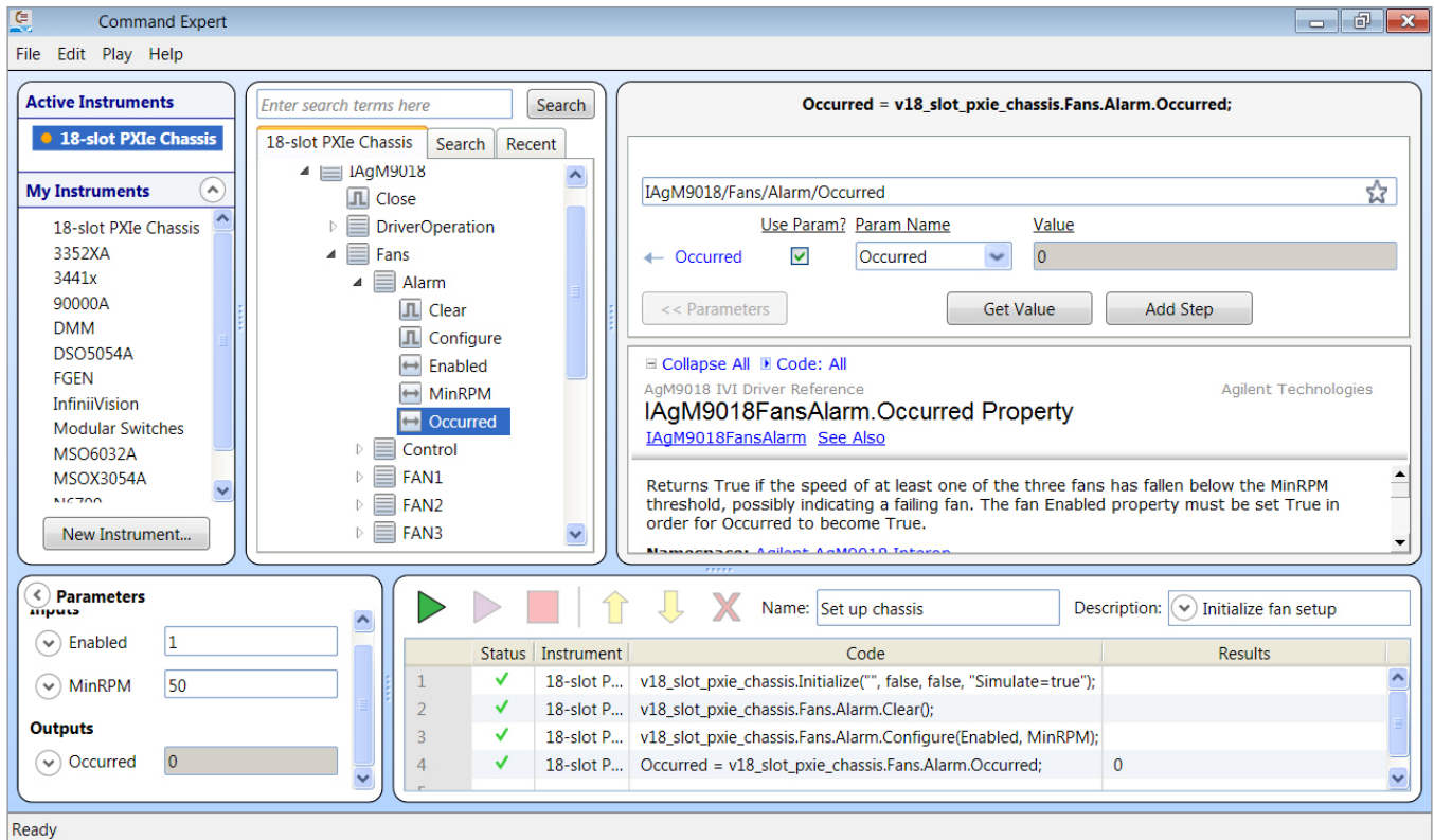
Figure 1. GUI for Keysight Command Expert example for PXI chassis fan control.
