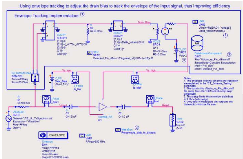
ADS Amplifier Design guide based envelope tracking example with 1 tone non-linear simulation
