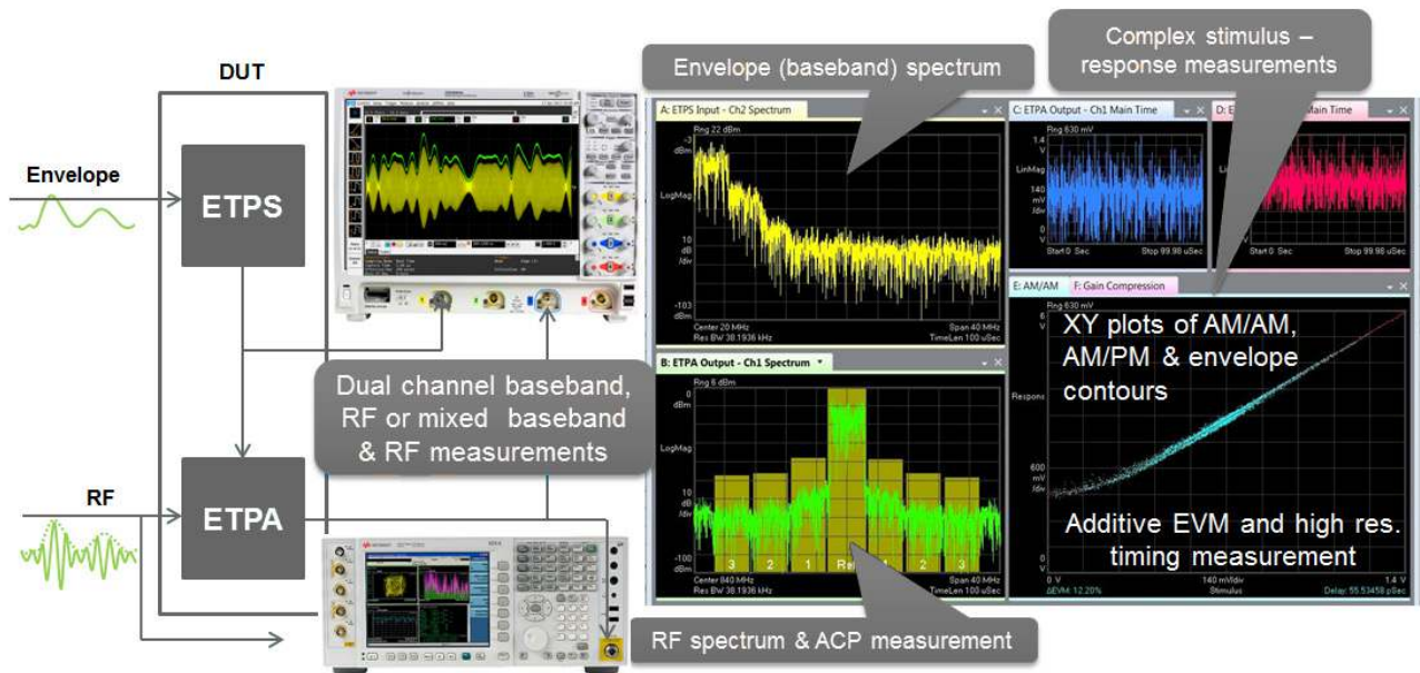
Analyze both RF and envelope signals using the 89600 VSA software
