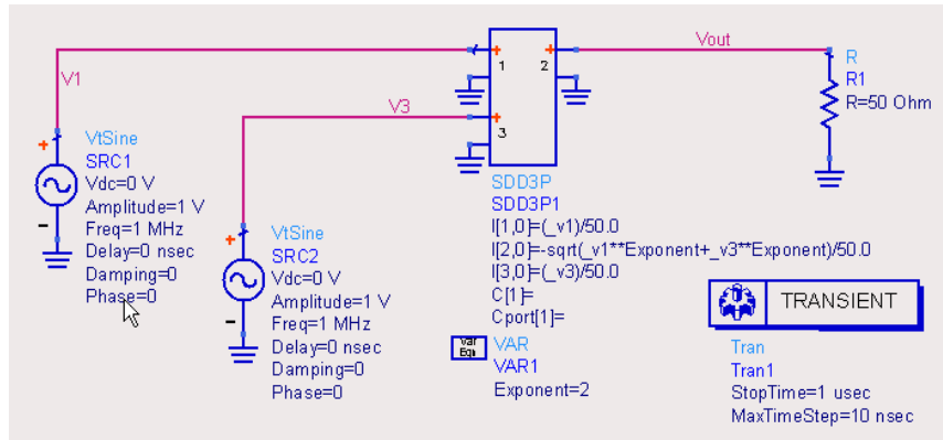
The diagram shows an example using a Symbolically Defined Device which allows you to very quickly and easily implement non-linear models without having to write code.
