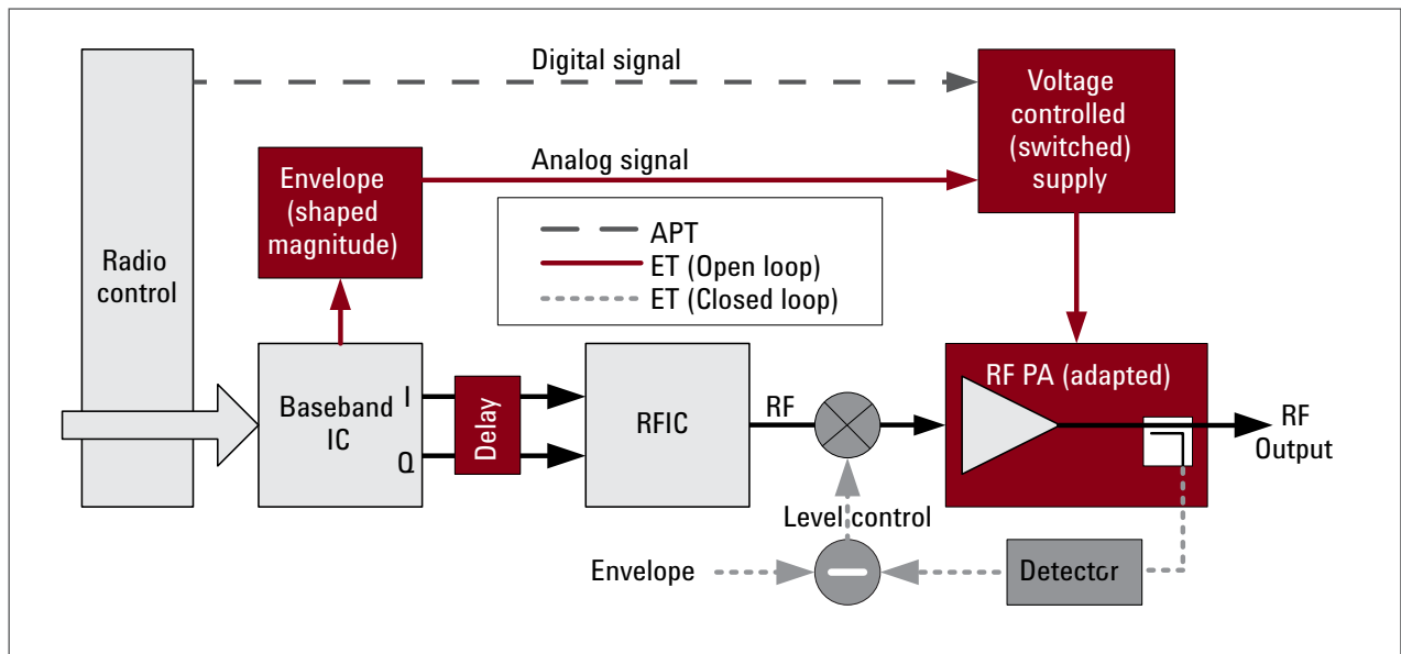
In a practical system, the envelope signal may be generated in the RFIC.
