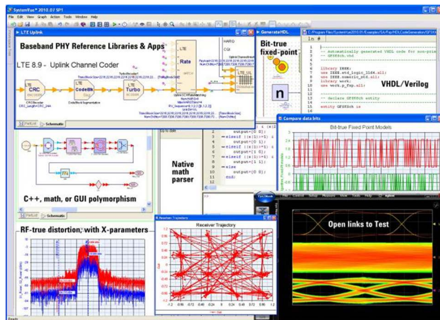
W1461 SystemVue communications architect core platform
