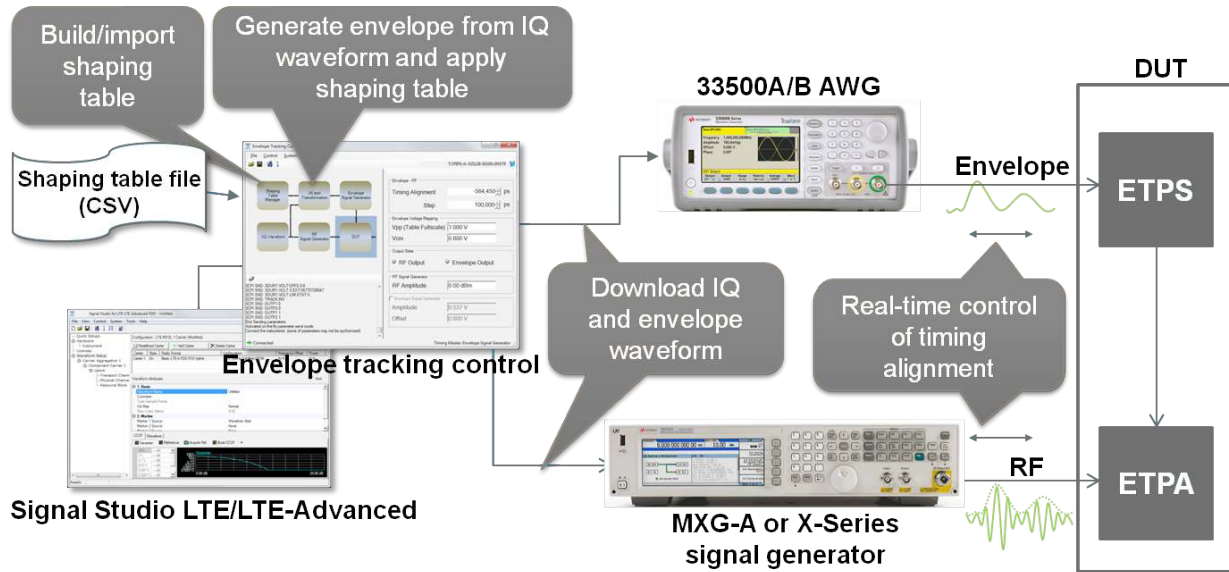
Synchronous envelope and RF signal generation
