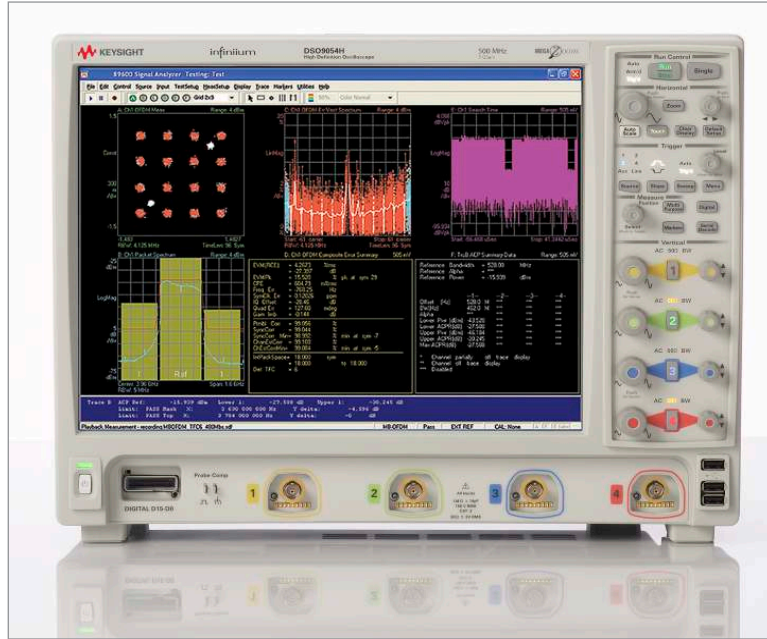
The 9000 series of oscilloscopes can be used standalone or in conjunction with the 89600 VSA for mixed RF and envelope measurements.
