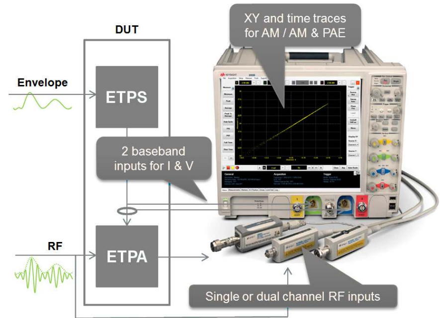
8990B peak power analyzer with combined power sensor and oscilloscope functions
