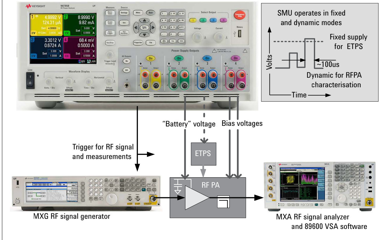
Use of the N6781A SMU in pulsed mode operation for PA characterisation
