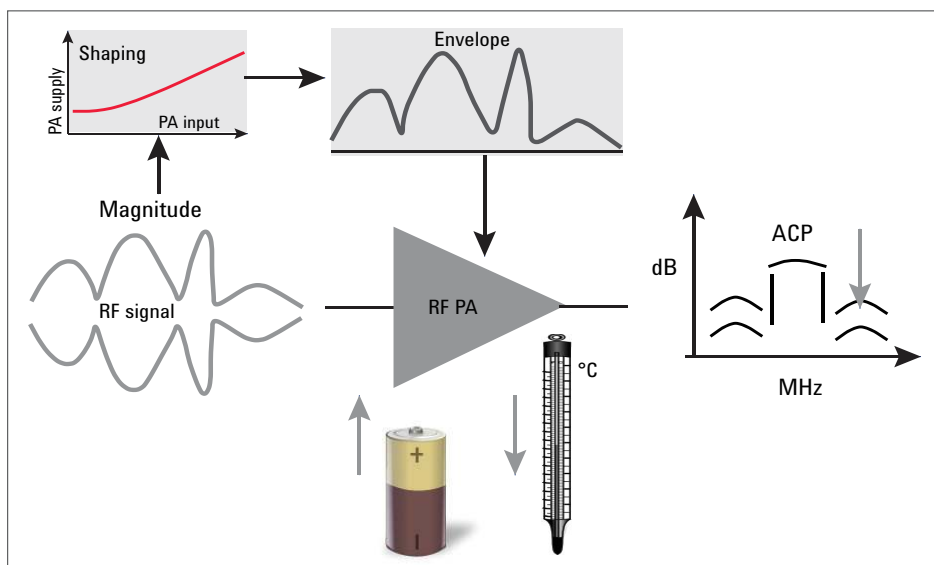
A high level view of envelope tracking operation and the benefits
