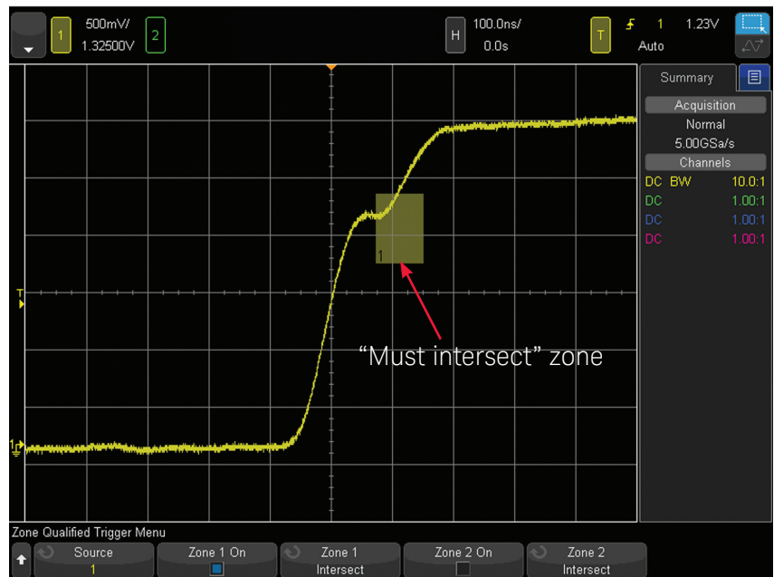
Figure 2: Capturing and displaying just waveforms with an anomaly (non-monotonic edge) using InfiniiScan Zone Trigger.
