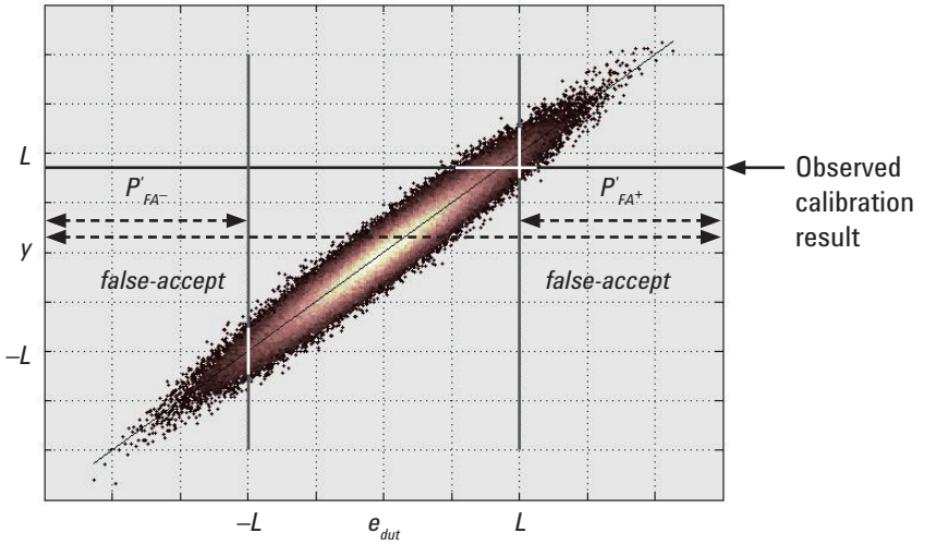
Figure 6. False-accept regions for Case C risk.
