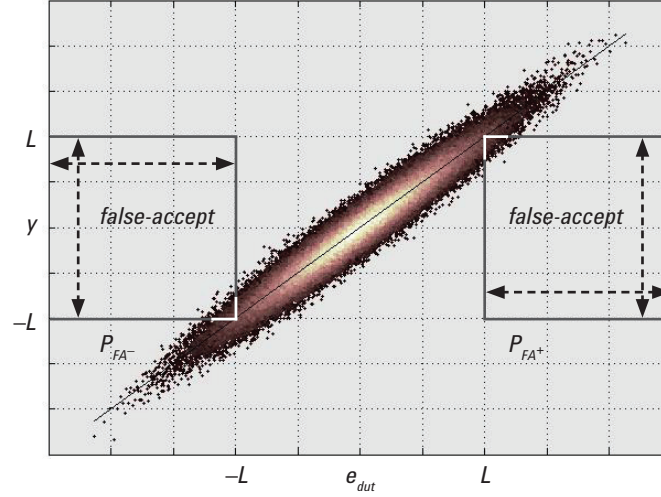
Figure 4. False-accept regions for Case A risk.
