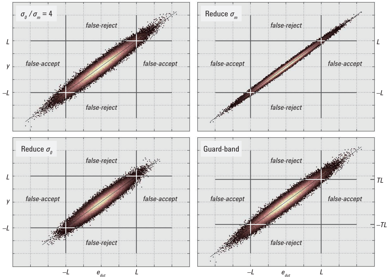
Figure 7. Reducing false-accept risk.
