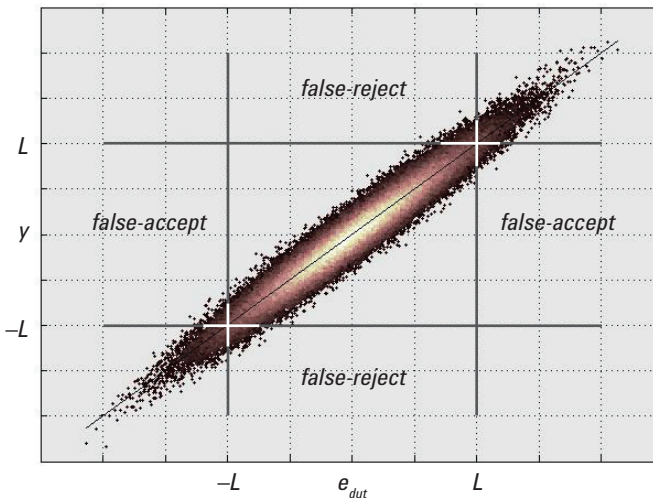
Figure 2. Tolerance limits defining false-accept and false reject regions.
