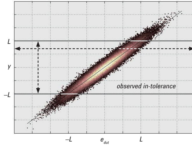
Figure 5. Observed in-tolerance region for Case B risk.
