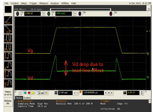
Effect of 50 Ω load line on Id-Vg measurement (conventional PG based solution)
