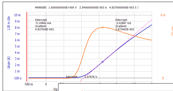
Sweep measurement
