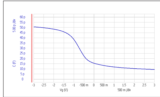
High frequency CV curve
