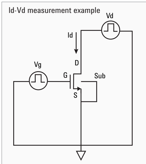
Source and measurement values of Id-Vd sweep are plotted
