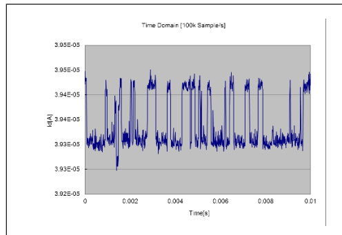
Random telegraph signal noise (RTN) measurement
