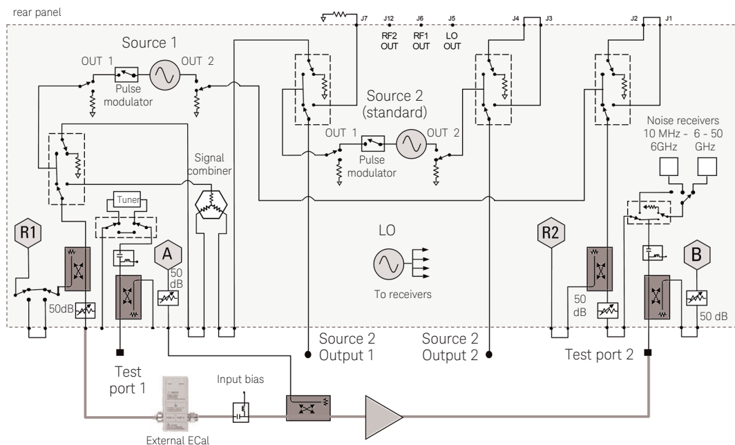
Figure 11. As an enhancement to using an external ECal for an optimal spready of source impedances, adding an external coupler and positioning it close to the DUT helps preserve raw directivity.
