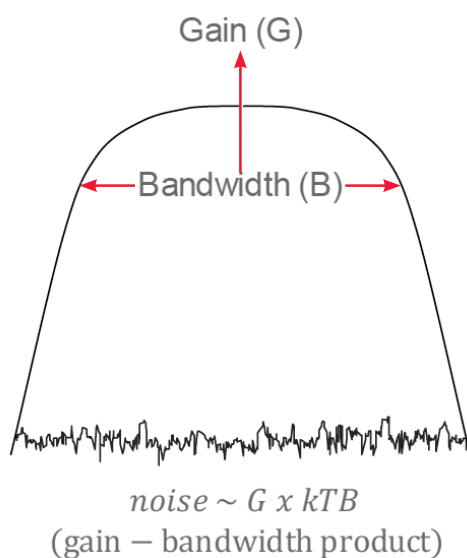
Figure 5. Characterizing the gain-bandwidth product of the noise receiver helps determine the internal noise contribution, which is used as a correction factor to provide calibrated measurements.
