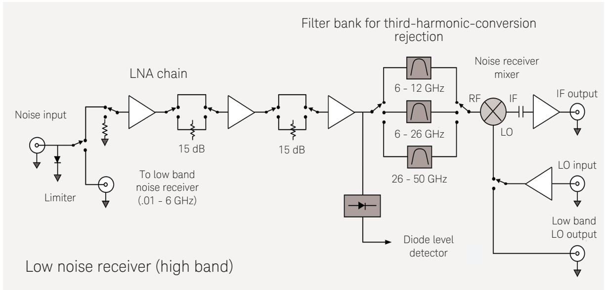
Figure 14. In the dedicated low-noise receiver, the signal path leading to the mixer includes a low-noise amplifier and a filter bank.
