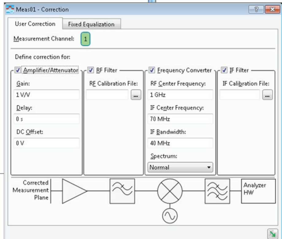
Figure 23. System level calibration example using Keysight's 89600 VSA software.
