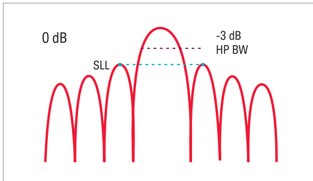
Figure 1. Sin(x)/x antenna radiation pattern.
