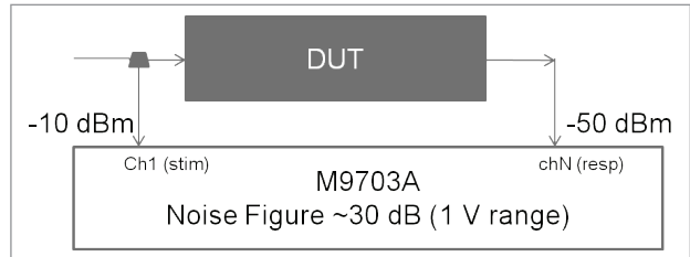
Figure 37. Estimating the digitizer performance of the M9703.
