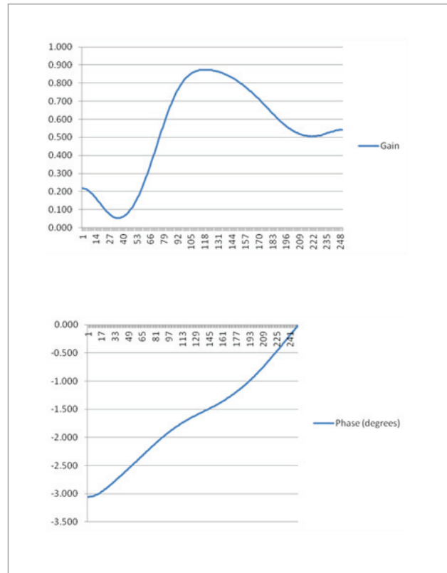
Figure 21. Magnitude and phase response for a single digitizer channel.
