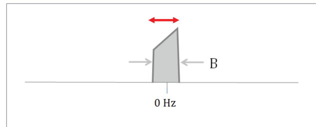
Figure 8. Complex signal asymmetric about DC.
