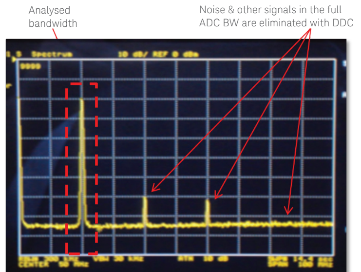
Figure 14. Bandwidth and noise reduction using a DDC.
