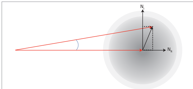
Figure 36. The real and imaginary components of noise vector.
