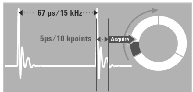
Figure 30. Circular acquisition buffer for segmented memory.
