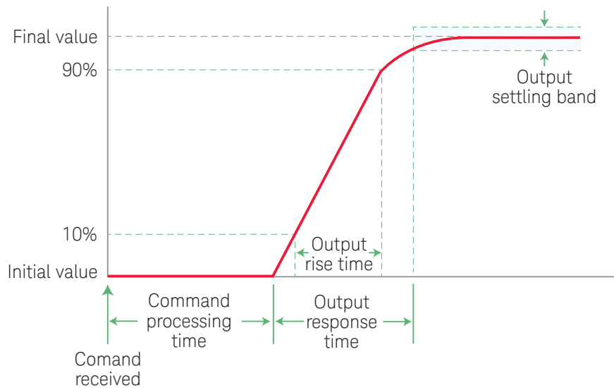
Figure 1-1. Power supply command processing time for an output level change
