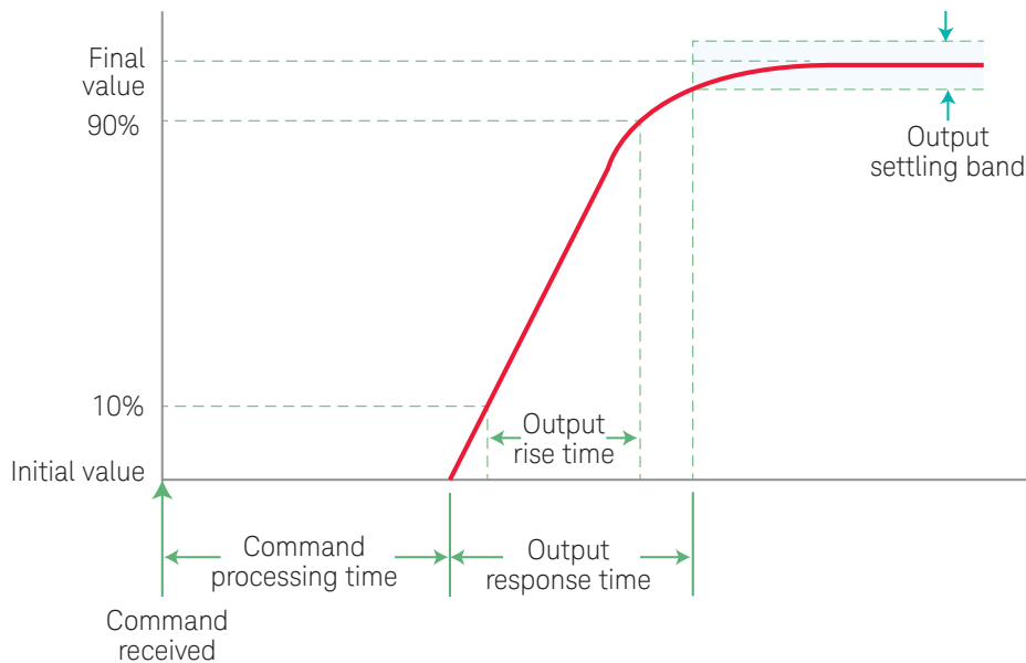
Figure 2-1. Power supply up-programming response time
