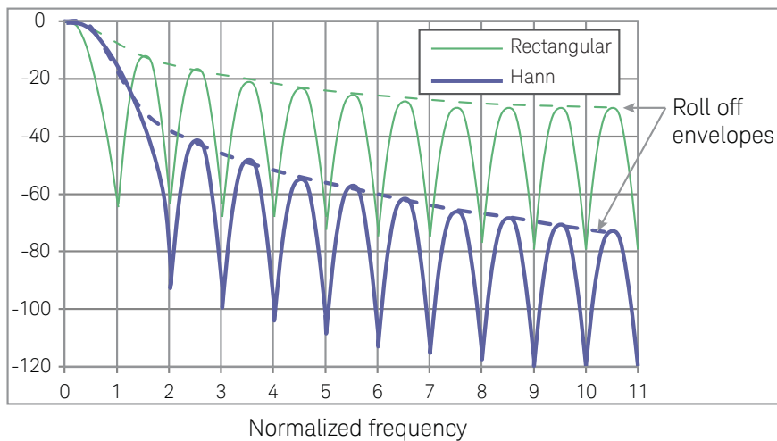
Figure 4-1. Rectangular and Hann window filter response characteristics
