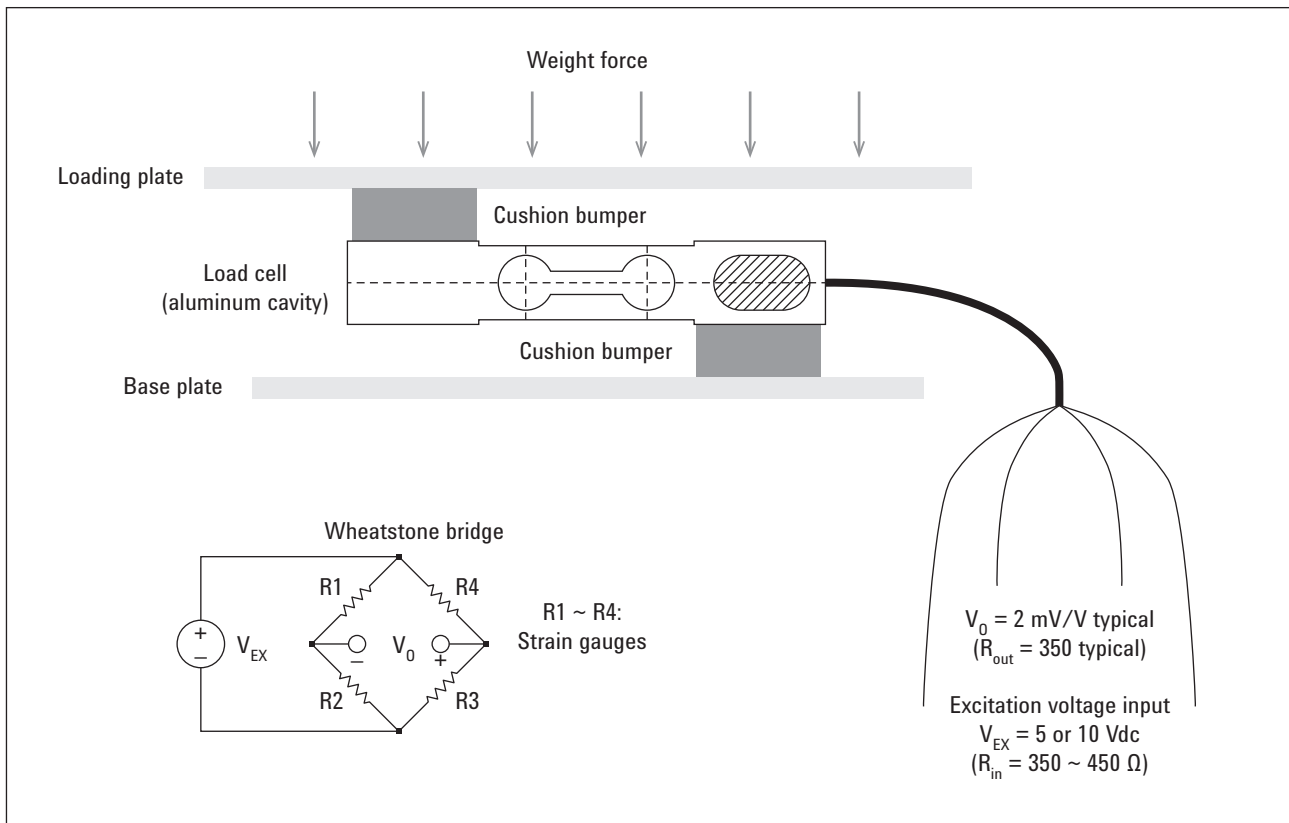
Figure 1. A weight indicator using a load-cell structure
