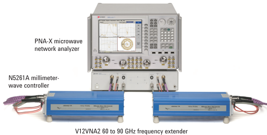
Figure 7. PNA-X with banded frequency extender
