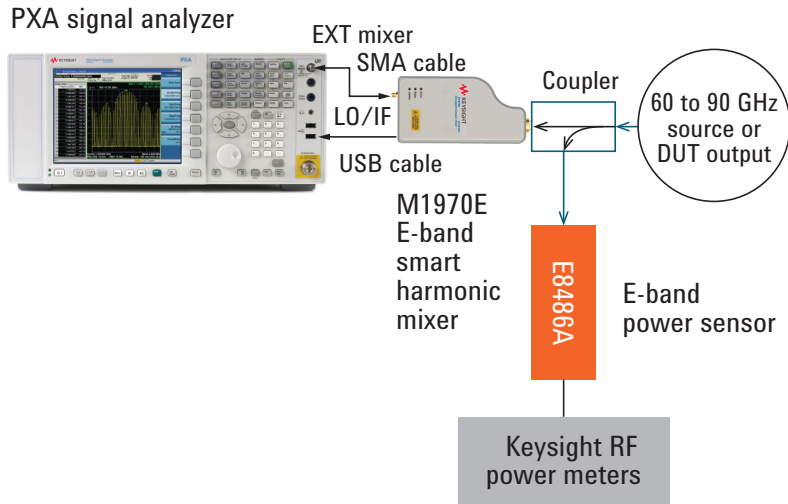
Figure 8. E-band spectrum analysis with RF power monitoring
