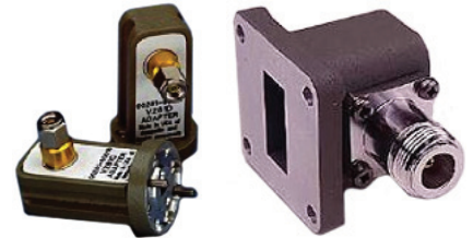
Figure 1. Waveguide to coaxial adaptors
