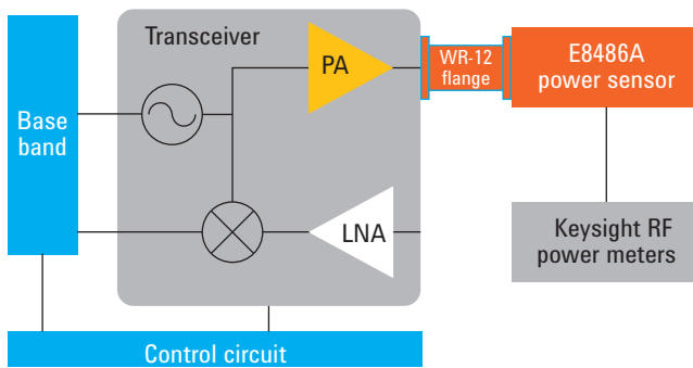
Figure 3. P2P transceiver output power measurement
