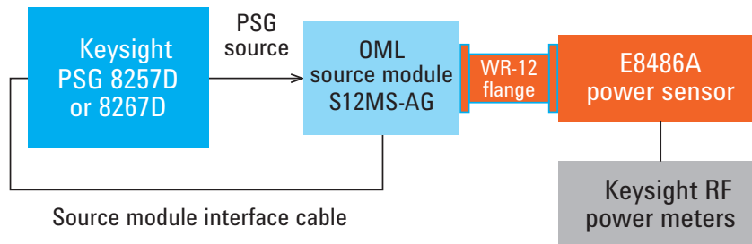
Figure 6. 60 to 90 GHz banded mm-wave source power calibration
