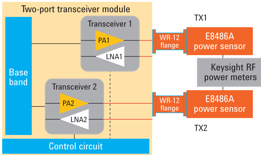
Figure 5. Two-channel, 77-GHz automotive radar transmitter output power measurement
