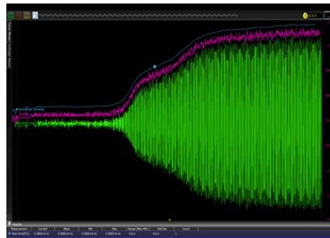
Amplitude demodulation
