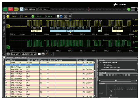
Protocol decode
